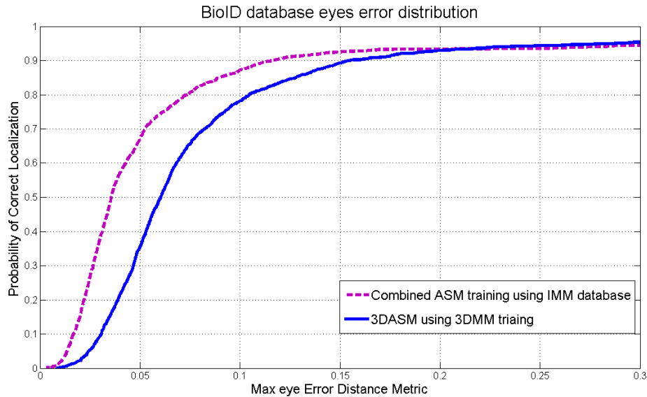
Figure 3.5: Comparison of our 3D-ASM and Combined-ASM from Chapter 2 on the BioID database for the two eyes.
