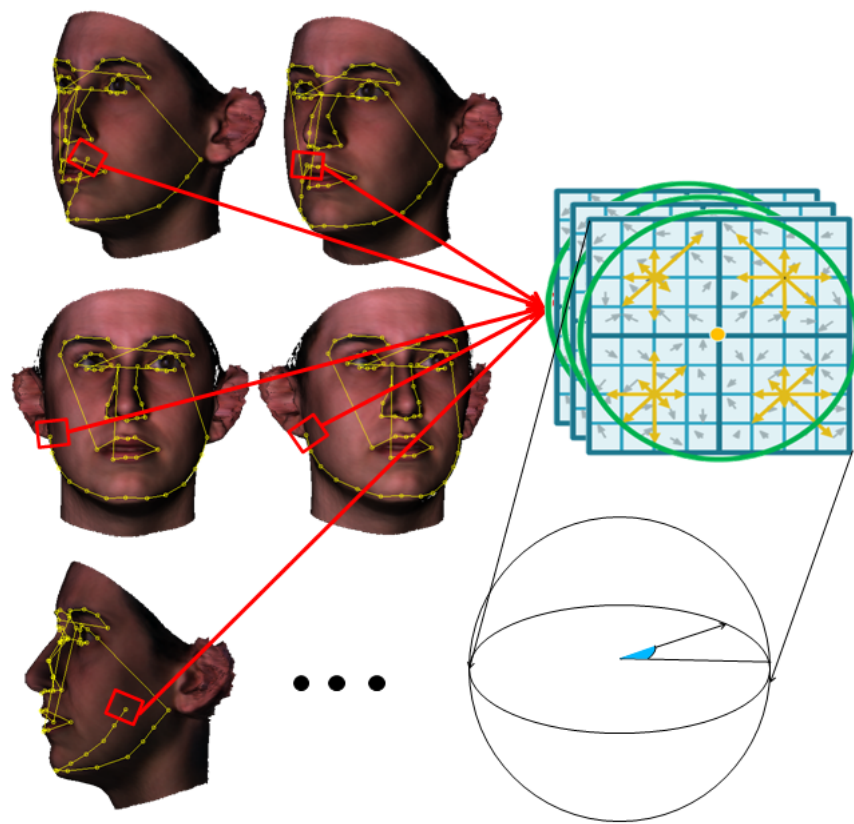
Figure 3.1: Illustration of 3D Local Texture Model. For each landmark, one 2DLTM is built separately for each viewpoint. 7 view-based 2DLTM compose our 3DLTM.
