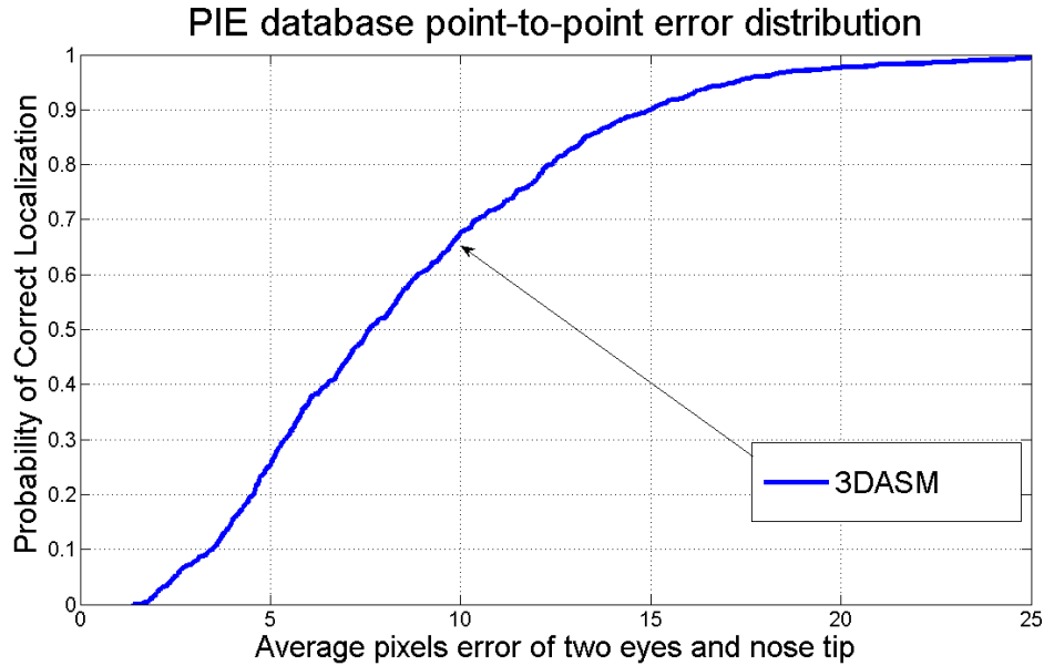
Figure 3.8: The 3D-ASM facial landmarks detector point-to-point error distribution on all 13 cameras on a subset of PIE database, for eyes and nose center points.
