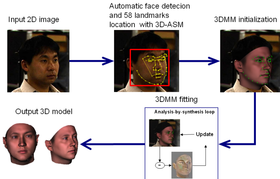
Figure 4.1: The framework of our automatic 3D face reconstruction algorithm from a single image with nonfrontal face. By using the landmarks detected by 3D-ASM, the pose of the 3DMM and the main facial feature are recovered. Example input 2D image is from the PIE database [60].
