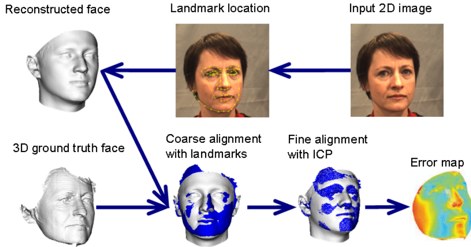
Figure 4.4: The framework of our 3D face reconstruction evaluation protocol. The input 2D image and the 3D ground truth scan are from the IV2 database [50].
