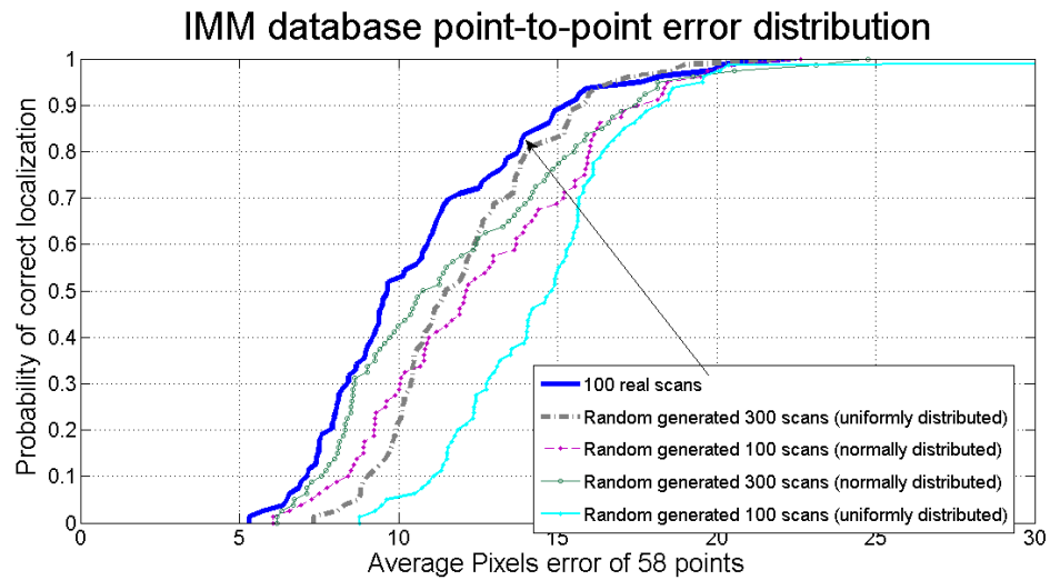
Figure 3.11: Influence of the training data to 3D-ASM. Comparison of landmarks location precision using different training data on the subset of IMM database.
