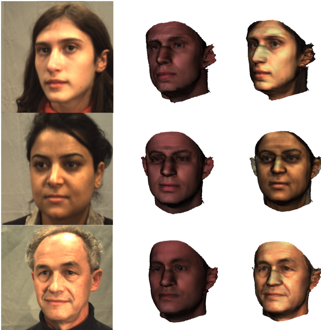
Figure 4.11: Typical 3D face reconstruction results using 3D-ASM landmark lactation for initialization. First column: the input 2D images. Second column: 3D reconstructed faces mapping with the texture from the 3DMM. Third column: 3D reconstructed faces mapping with texture extracted from the input 2D images . The input 2D images are from the IV^2 database [50].
