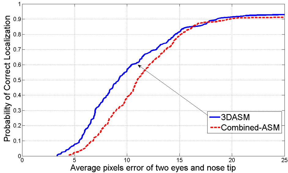
Figure 3.6: Comparison of our 3D-ASM and Combined-ASM from Chapter 2 on the subset of PIE Database.
