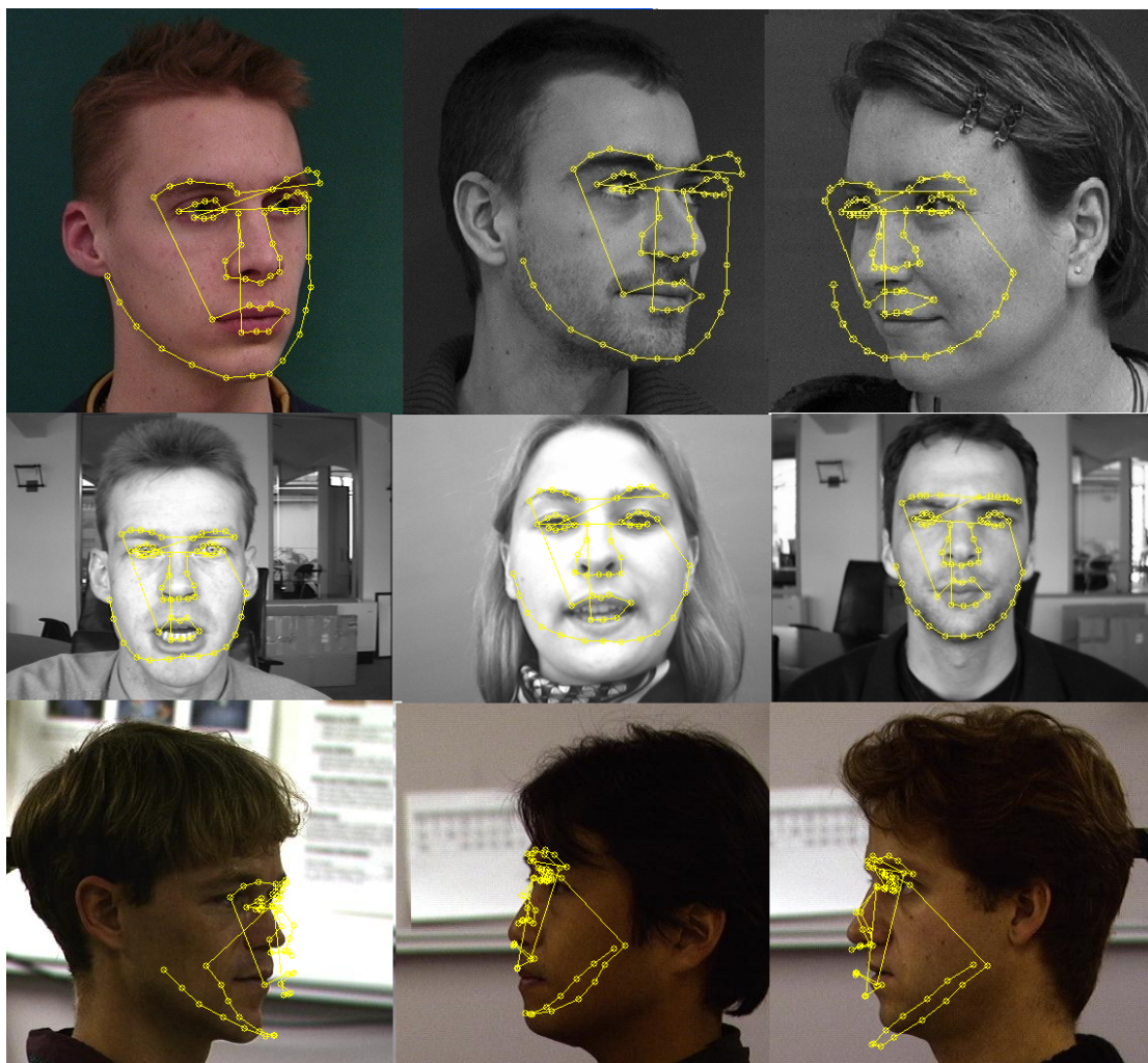
Figure 3.13: Error analysis: Bad landmark location examples from IMM, BioID and PIE database.
