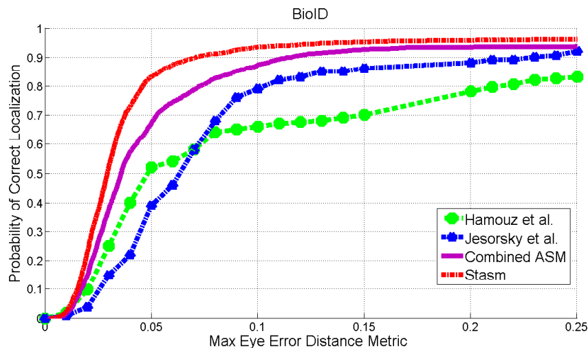
Figure 2.8: Comparison of the proposed Combined-ASM with already published results for eyes detections on the BioID database.
