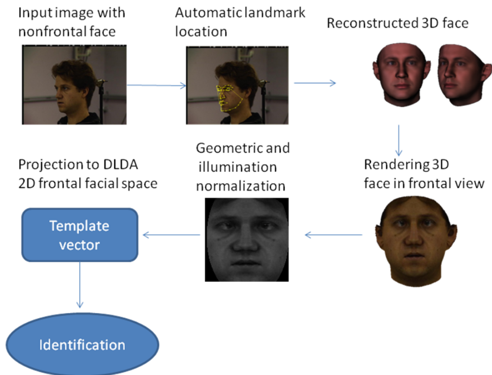
Figure 5.3: Flow charts of face identification across pose by viewpoint normalization approach.
