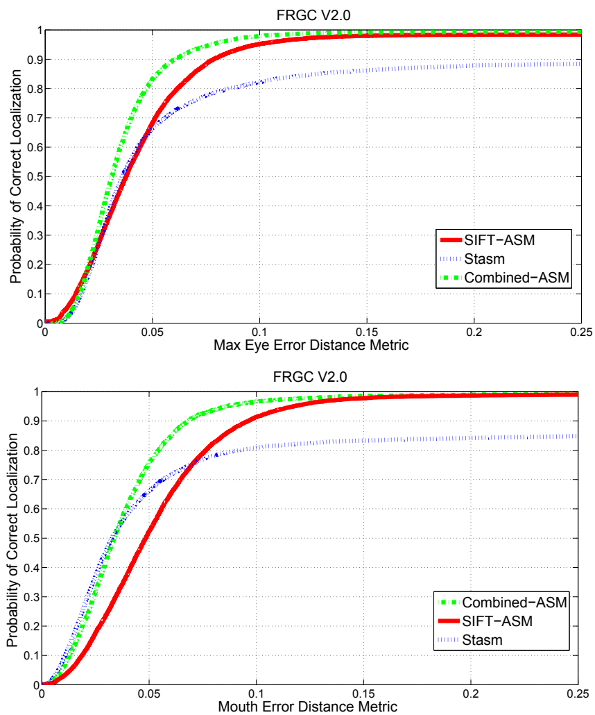
Figure 2.9: Cumulative histograms on FRGCv2.0 database with maximum eyes and mouth error, the Stasm in this experiential we used the default training data (STASM-original).
