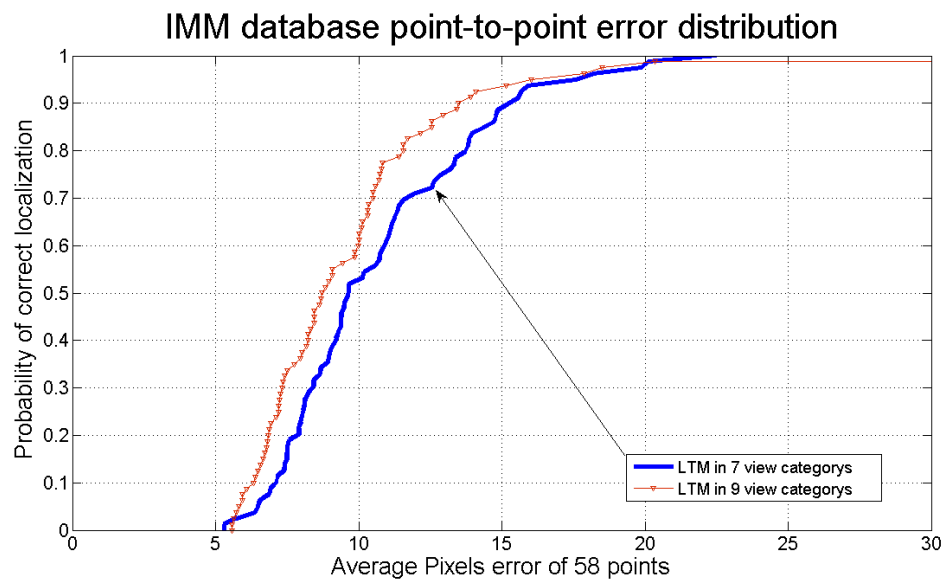
Figure 3.12: Comparison of landmarks location precision using different view categories for training. Evaluated on IMM database.
