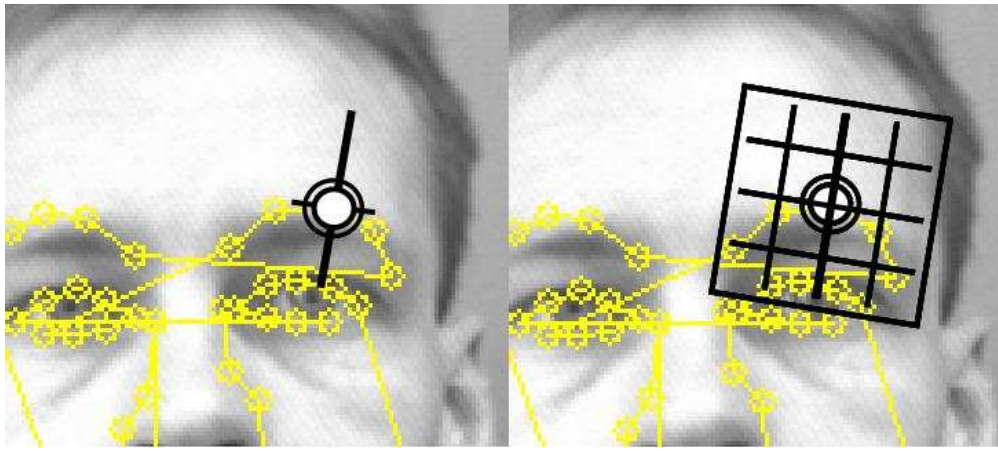
Figure 2.2: Difference of the Grey-Level Profile and the SIFT descriptor. Left: The Grey-Level Profile (GLP) is extracted from the neighbourhood pixels perpendicular to the contour. Right: The SIFT descriptor is computed over a patch along the normal vector at the landmark (the original image is from the BioID database [34]).
