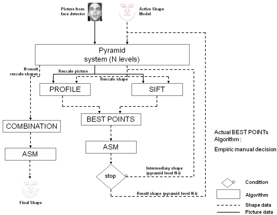
Figure 2.5: Combined Active Shape Model marching algorithm flow chart.
