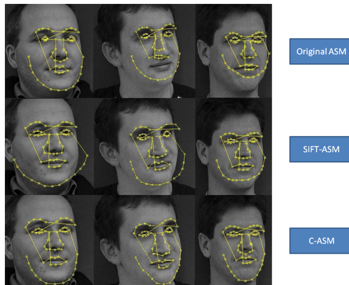
Figure 2.6: Typical fitting result of non frontal faces achieved by original ASM (top row), SIFT-ASM (middle row) and C-ASM (bottom row). (The original images are from the IMM database [63]).
