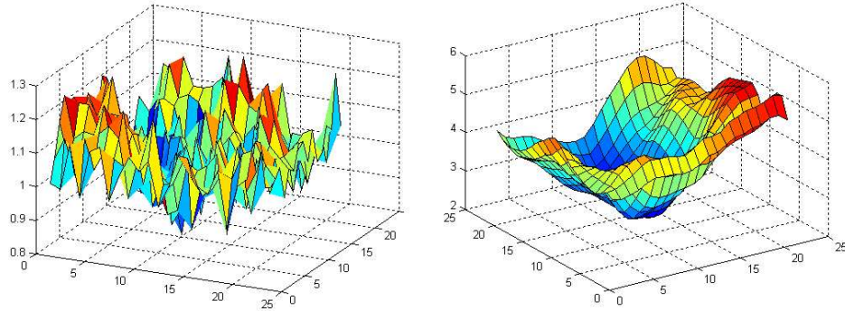
Figure 2.3: Comparison of the Grey-Level Profile and the SIFT descriptor cost function from Eq 2.3. Left: Gradient profile matching cost of the landmark highlighted in Figure 2.2 over a window of size 21x21. Notice the multiple minima resulting in poor alignment of shapes. Right: SIFT descriptor matching cost for the same landmark point.
