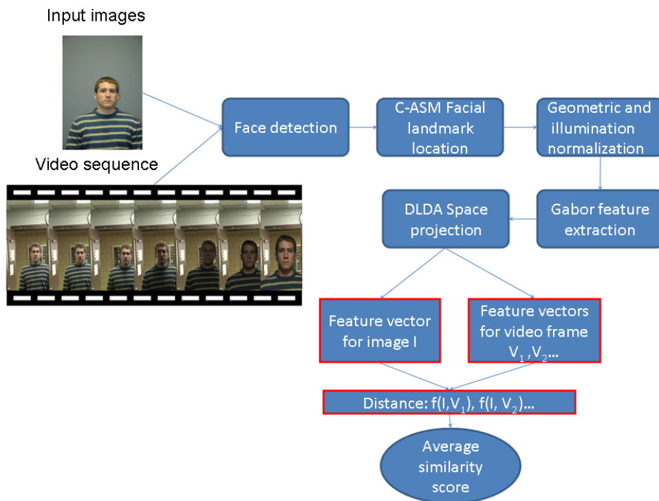
Figure 2.10: Flow chart of the system for our fully automatic face recognition based on C-ASM and global features. Images and video from MBGCv1 portal challenge [46].
