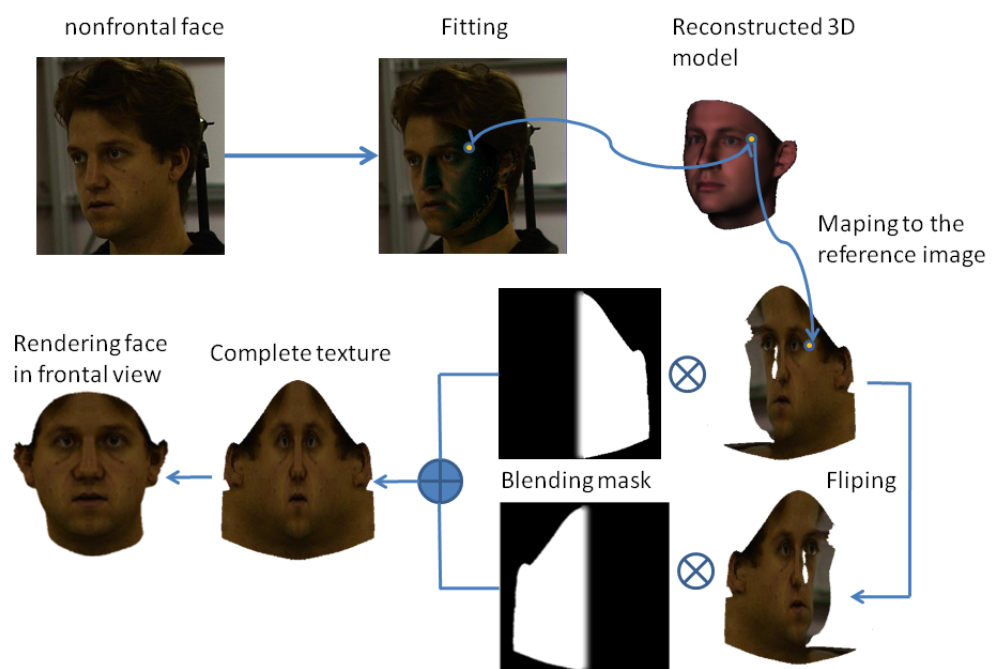
Figure 5.5: Block diagram for pose normalization using 3DMM fitting and facial symmetry. Texture from the input image is extracted by projecting the vertices of the 3DMM on the image plane. If these vertices are visible, the RGB values will be taken and copied to the texture map which is presented in cylindrical coordinates. The final texture is completed using symmetry property of faces.
