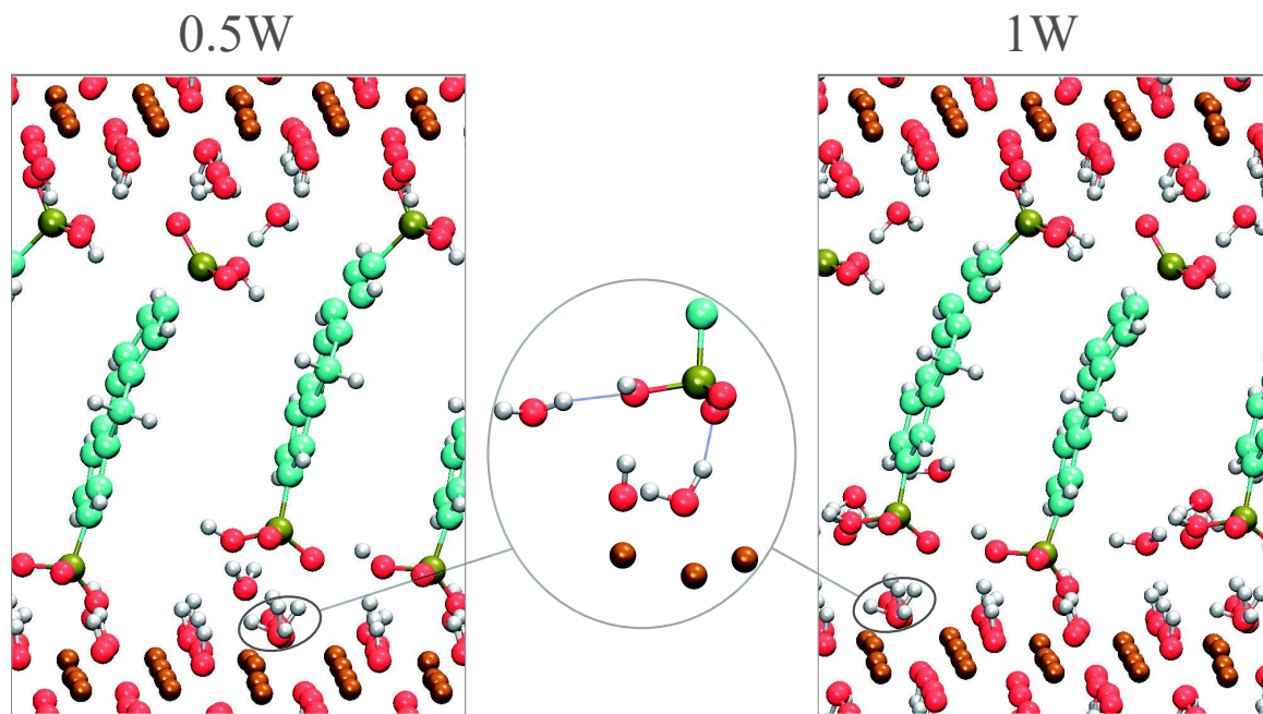
Figure 70 – Optimized structures of a hydrated copper hydroxide fluorene biposphonic compound \text{Cu}_2(\text{OH})_{3.75}(\text{C}_{13}\text{H}_{10}\text{O}_6\text{P}_2)_{0.25}(\text{H}_2\text{O})_y with y = 0.5 (left part) and y = 1 (right part). The specific local configuration of water molecules in "cavities" positions (see text) is represented in the central part of the figure
