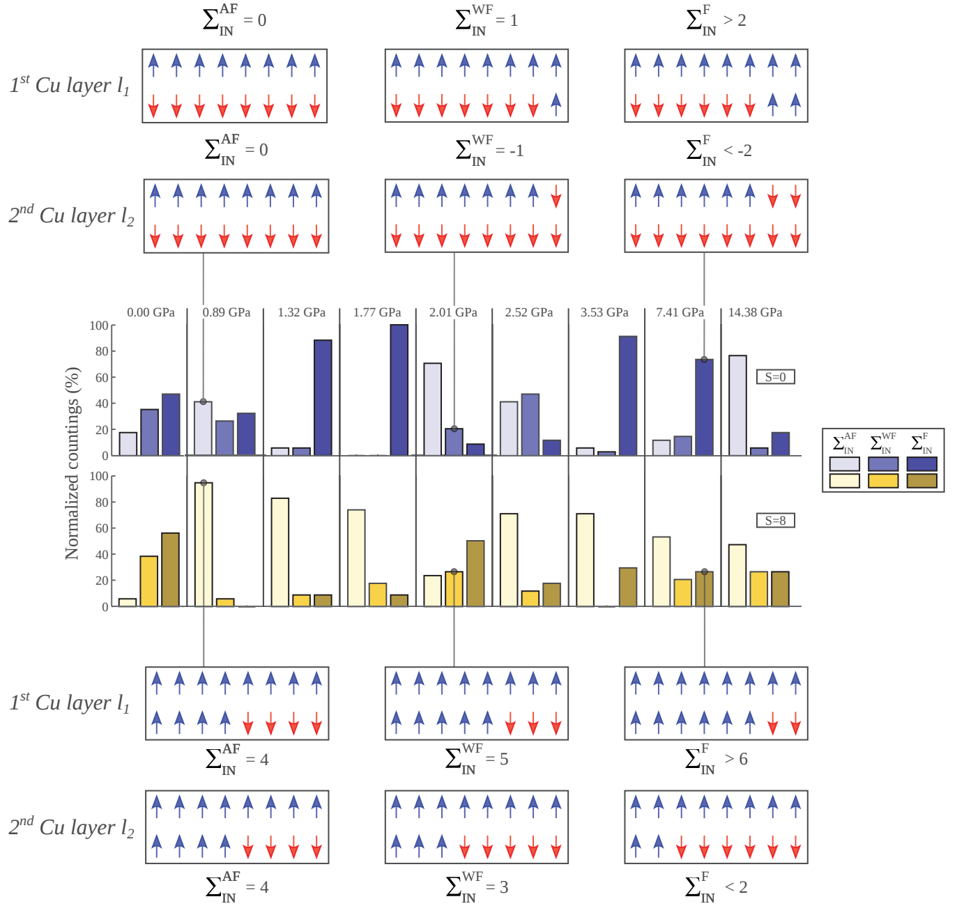
Figure 91 – Spin density distribution analysis of copper hydroxide acetate system in two magnetic configurations, the anti-ferromagnetic one (S=0) and a ferromagnetic one (S=8). In-layer (copper layers) magnetizations \Sigma_{IN} among the two layers ( l_1 and l_2 ) are represented in schematic pictures allowing to visualize the various spin configurations corresponding to the colors of the bar plot. This bar plot gives, for each pressure system, an evaluation (in percent) of the number of stable magnetic configurations obtained (from the 17 DFT calculations performed at each pressure), sorted by colors from light color (low in layer magnetization, AF), intermediate color (weak ferromagnetism, WF) to darker colors (in layer ferromagnetic behaviors, F)
