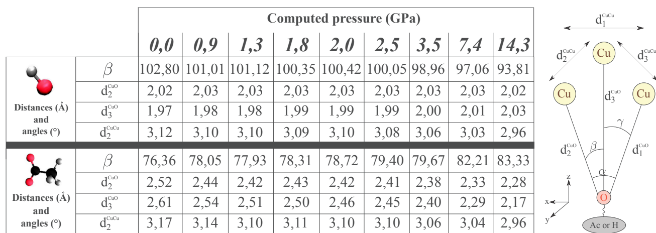
Figure 90 – Specific Oxygen atoms ( O_{81}^{Hydroxide} and O_{79}^{Acetate} ) tetrahedra deformation as a function of external pressure in copper hydroxide acetate system
