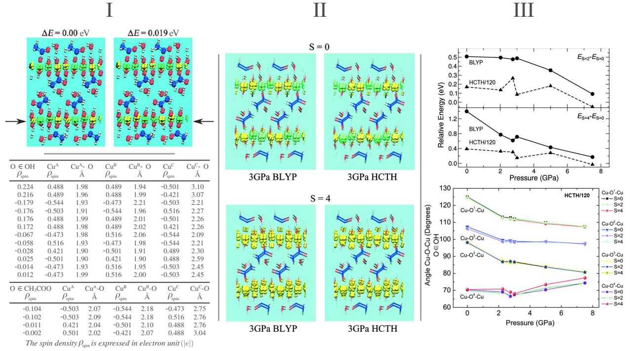
Figure 27 – I ) Top part: Copper hydroxide acetate \text{Cu}_2(\text{OH})_3(\text{CH}_3\text{COO}) \cdot \text{H}_2\text{O} ( \text{CuOHAc} ) optimized structure ([010] view) for the antiferromagnetic configuration (total spin S = 0 ) for the two spin density distributions resulting in the lowest total energies of the system. Cu atoms are brown, C in blue, O in red, H in white and the solid surfaces correspond to isosurfaces of spin density ( \alpha in green and \beta in yellow) at a value of \pm 0.03 \text{ e}/\text{\AA}^3 ( adapted from Figure 1 of ref. [36] ). Bottom part: Spin density values ( \rho_{spin} ) localized on the two types of oxygen atoms (see text) in correspondence with the spin density and distances of the three nearest neighbor copper centers \text{Cu}^A , \text{Cu}^B and \text{Cu}^C ( adapted from TABLE 4 of ref. [36] ). II ) Spin density distribution for the \text{CuOHAc} system under 3 GPa of applied pressure calculated with BLYP (left) and HCTH (right) exchange correlation functionals and for two total spin states of the system, S = 0 (top) and S = 4 (bottom). \alpha and \beta isospin surfaces are in light green and yellow respectively and the isosurfaces are plotted for spin density values of \pm 0.01 \text{ e}/\text{\AA}^3 ( adapted from figures 2 and 3 of ref. [37] ). III ) Top part: Relative total energies, with respect to the S = 0 AF configuration, of the S = 2 and S = 4 spin states of \text{CuOHAc} system as function of the applied pressure and for two exchange-correlation functionals: BLYP (solid line, filled circles) and HCTH/120 (dashed line, filled triangles). Bottom part: \text{Cu-O-Cu} angles as function of applied pressure for each oxygen (belonging to \text{CH}_3\text{CO}_2^- group) bridging copper sites in \text{CuOHAc} structure. For clarity, \text{Cu-O}^i\text{Cu} ( i=1-4 ) curves are rigidly shifted along the y-axis ( the corresponding original Figure and numerical values are present in Figure 4 and Tables 2, 3 and 4 of ref. [7] ).
