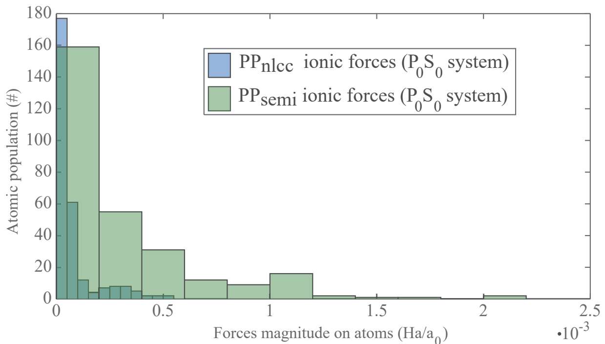
Figure 53 – Histogram of ionic forces corresponding to the 288 atoms of the copper hydroxide acetate structure studied with two different PP used for describing copper ions: the semi-core PP (green) and NLCC (blue). The system considered is the anti-ferromagnetic ground state of CuOHAc system at 0 pressure
