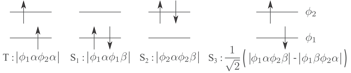
Figure 22 – The two possible electrons configuration: the Triplet (T) and Singlet (S) states corresponding to \phi_1 and \phi_2 , the molecular orbitals constructed from the partially occupied d_{x^2-y^2} orbitals of two metal centers forming a M_a -X- M_b bridged system (X being the anion)
