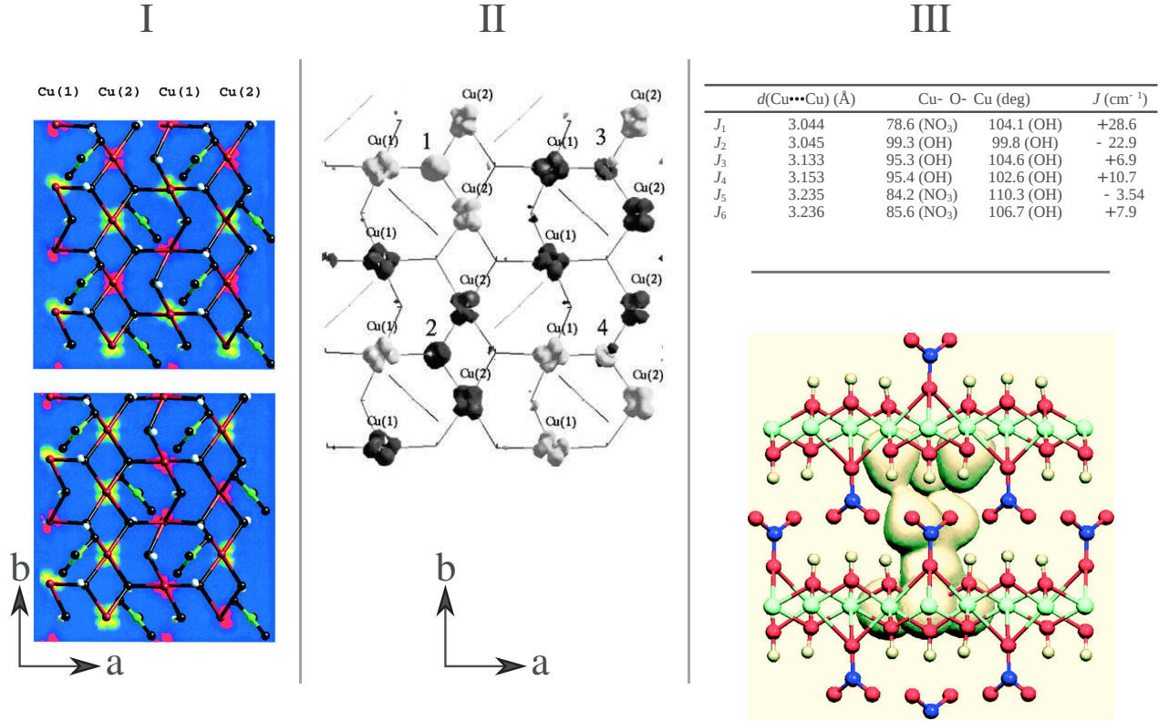
Figure 26 – I) Two different (a,b) planes of the model used by Massobrio and coworkers [115] for the \text{Cu}_2(\text{NO}_3)(\text{OH})_3 system. The contour slices correspond to values of spin densities ranging from -0.1 to 0.1 |e| with positive and negative spin densities in red and green respectively. Spin density is localized around copper sites (brown spheres) while negligible amounts appear in the rest of the system. O atoms are black, N atoms are green and H atoms are white spheres (adapted from Figure 3 of ref. [115]). II) Spin density distribution in the (a,b) plane of copper hydroxide nitrate system highlighting non-negligible spin densities on oxygen sites. The solid surfaces correspond to majority (grey) and minority (black) spin density isosurfaces at 5 \cdot 10^{-2} \text{ e}/(\text{bohr})^3 . The labels Cu(1) and Cu(2) correspond to copper sites with different environments and 1, 2, 3, 4 labels correspond to the oxygen bridges between specific copper sites (adapted from Figure 2 of ref. [116]). III) The table shows the exchange coupling constants J_i ( i=1,\dots,6 ) and structural parameters for the six exchange pathways identified in copper hydroxynitrate calculated using first-principles methods with the use of B3LYP exchange-correlation functional (adapted from table 1 of ref. [117]). The bottom part shows the total electron density isocontour at a value of 0.12 \text{ e} \cdot \text{\AA}^{-3} for the \text{Cu}_3 \cdots \text{NO}_3 \cdots (\text{OH})_3 fragment in the interlayer region of CuOHN system (adapted from Figure 7 of ref. [118])
