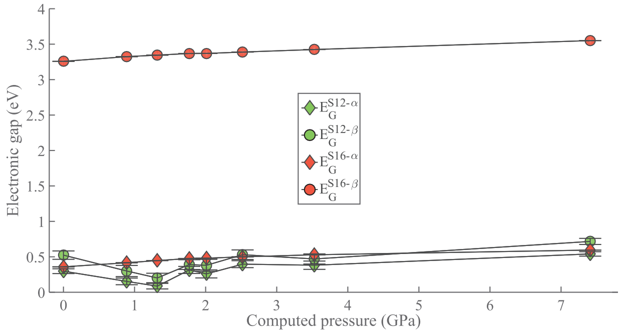
Figure 93 – Evolution of copper hydroxide acetate electronic gaps as function of pressure computed from first-principles calculations. The two magnetic states considered are ferromagnetic configurations ( S=12 in green and S=16 in red). The errorbars are produced from the randomization procedure applied on the initial electronic of freedom resulting in multiple energy minima landscape
