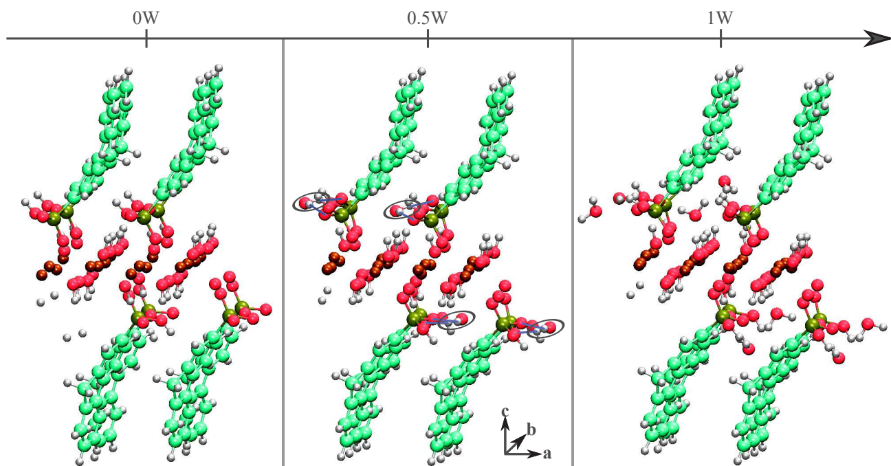
Figure 67 – Atomic structures of optimized hydrated copper hydroxide fluorene monophosphonic compounds Cu_2(OH)_3(C_{13}H_{10}O_3P)_1 \cdot (H_2O)_y with y = 0, 0.5 (4 water molecules) and 1W (8 water molecules). In the 0.5W system, water molecules are highlighted with black ellipses and the corresponding H-bonds are drawn in blue dotted lines
