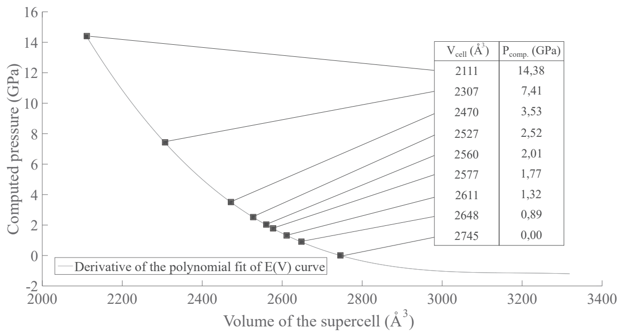
Figure 82 – Equation of state, i.e pressure as function of volume corresponding to the compression of copper hydroxide acetate system starting from the optimal structural ground state identified in the parametric space of crystallographic lattice parameters. The deformations of the system are evaluated following the experimental observations by Suzuki et al [4] of copper hydroxide acetate lattice variations when pressure is applied along the \vec{c} -direction
