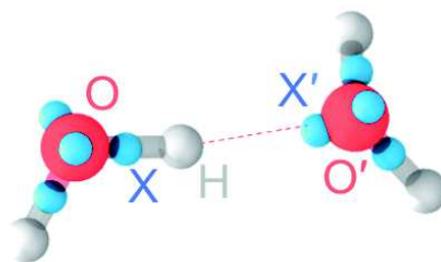
Figure 77 – Schematic representation of a typical hydrogen bond promoted by two water molecules. The oxygen (O), hydrogen (H) and WFCs (X) are indicated in red, gray, and cyan respectively. The acceptor oxygen and one of its lone pair WFC are indicated as O' and X', respectively
