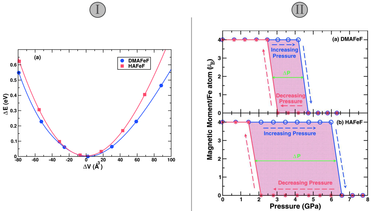
Figure 58 – I Energy as a function of volume for the two compounds considered in ref. [6]. II : computed magnetic moment per Fe atom as a function of increasing (blue) and decreasing (red) pressure for both DMAFeF (a) and HAFeF systems (b). Data published by H. Banerjee et al. [6]
