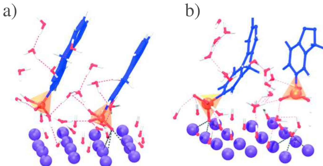
Figure 76 – The local bonding environments surrounding the phosphonate groups ( -\text{PO}_3\text{H} ) for 3a ⊂ Cu and 6a ⊂ Cu are visualized in (a) and (b), respectively. The interaction between Cu atoms with the -\text{PO}_3\text{H}^- groups as well as with the O atoms of the water molecules are indicated as gray dashed lines. The H-bonding network is highlighted in red dashed lines
