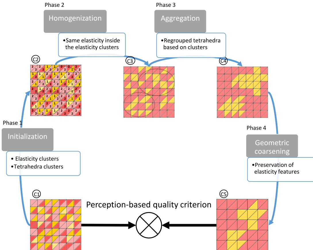
Figure 3.2 – Schematic diagram of our elasticity-based clustering approach. It is composed of 4 phases: 1) Initialization: creates elasticity bins and tetrahedra clusters inside these elasticity bins. 2) Homogenization: unifies the elasticity inside the elasticity bins. 3) Aggregation: modifies the elasticity inside the object according to the tetrahedra clusters. 4) Geometric coarsening: attributes elasticity to the coarse mesh. Cube 1 (C1) represents the initial distribution of the elasticity. Red and yellow elements represent respectively stiff and soft elements, and the different tints for each color represent close elasticity values. Cube 2 (C2) represents the cube after the initialization phase, with information added to the tetrahedra: all tetrahedra are labelled with their elasticity bins (1 or 2); and barycentric clusters have been computed for all elasticity bins except one (here two clusters for the yellow elements). After the homogenization phase, in Cube 3 (C3), all tints for each color have been modified to the homogenized elasticity value for each elasticity bin. Tetrahedra are then regrouped for each cluster around the cluster barycenter in Cube 4 (C4), creating two large homogeneous volumes. A coarser mesh is finally used for Cube 5, with fewer elements, and the elasticities are chosen to match at best the elasticity from the fine resolution.
