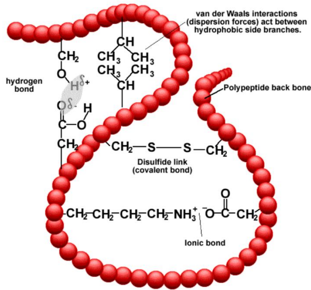
Fig. II.3: Protein tertiary structure stabilizing interactions. Interactions between amino acids side chains: Ionic bonds, hydrogen bonds, van der Waals interactions, and covalent disulfide bridges.
