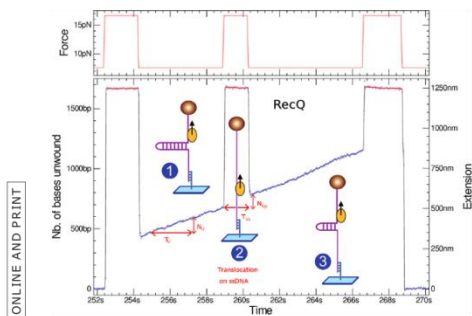
Figure 10. To investigate the translocation of a helicase on ssDNA the following assay has proved useful. Once the enzyme has started to unwind the hairpin fork, the force is increased such as to mechanically unzip the hairpin. The enzyme thus proceeds by translocating on ssDNA for a time T_{SS} determined by the time span over which the hairpin is maintained open. Upon reducing the tension of the DNA molecule, the hairpin rewinds until its fork encounters the helicase. At that point the increase in the DNA's extension, N bpS, allows one to deduce the rate of translocation of the enzyme on ssDNA: v_{SS} = N \text{ bpS} / T_{SS}
