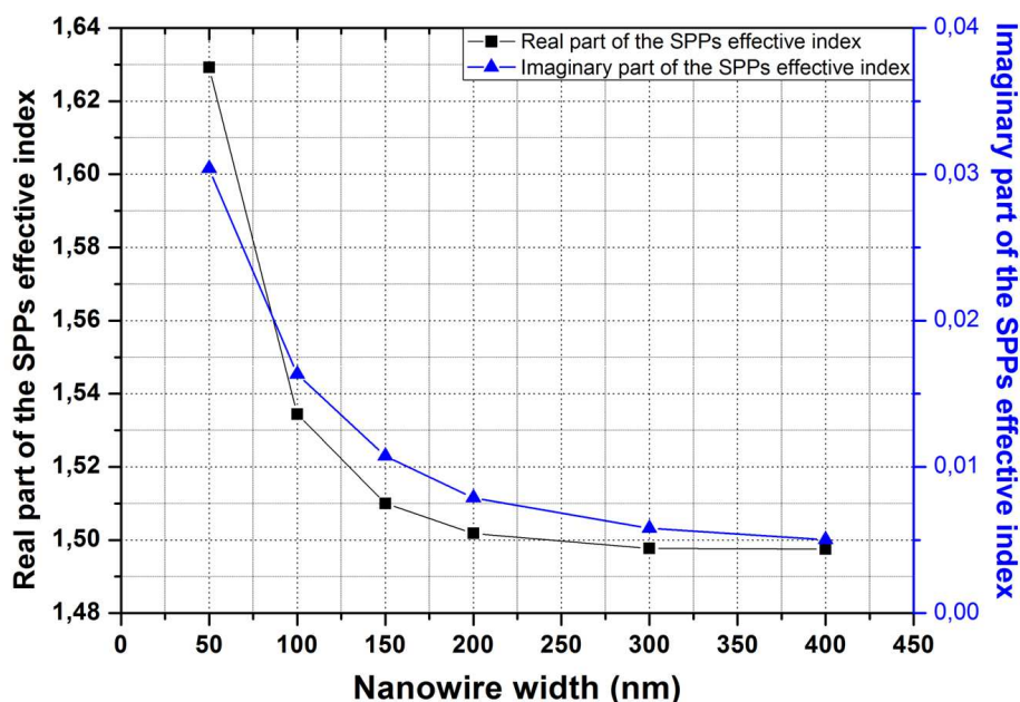
Figure 4.3: Numerically calculated effective mode index of the SPPs propagation versus the nanowire width ranging from 50 nm to 400 nm at \lambda = 1.55 \mu\text{m} telecom wavelength
