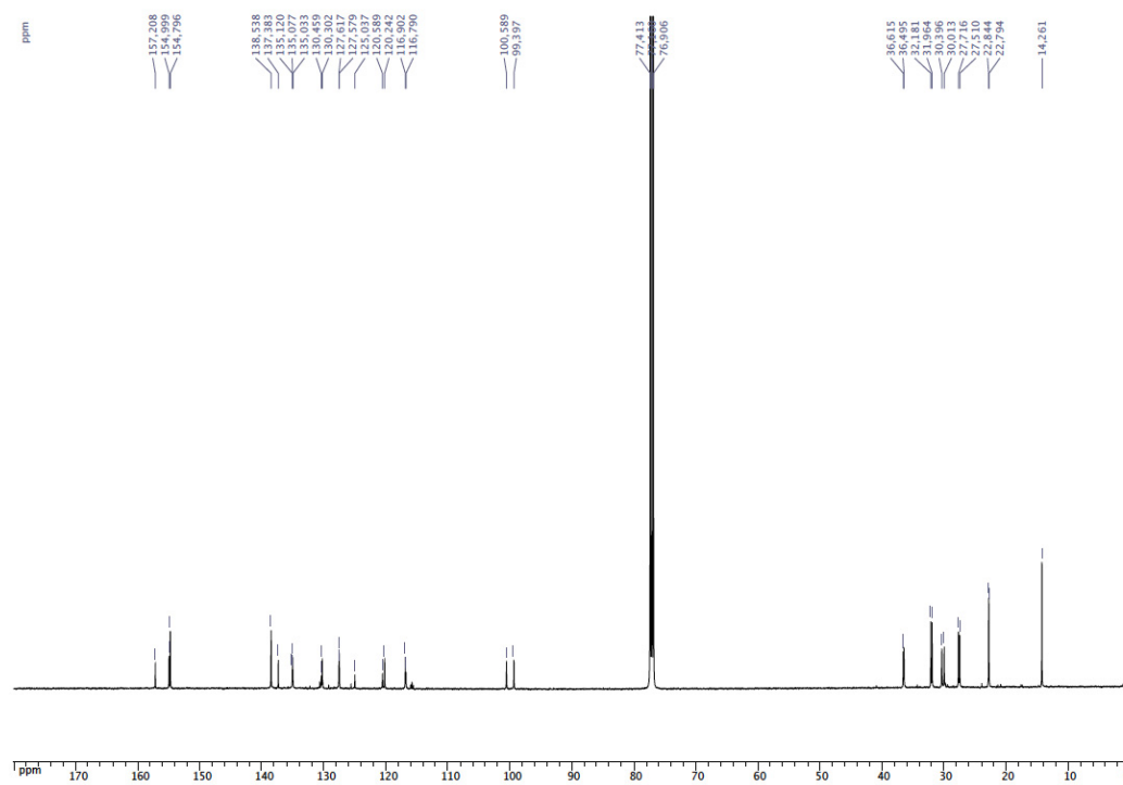
^{13}\text{C}\{^1\text{H}\} NMR spectrum of 13 ( \text{CDCl}_3 )
