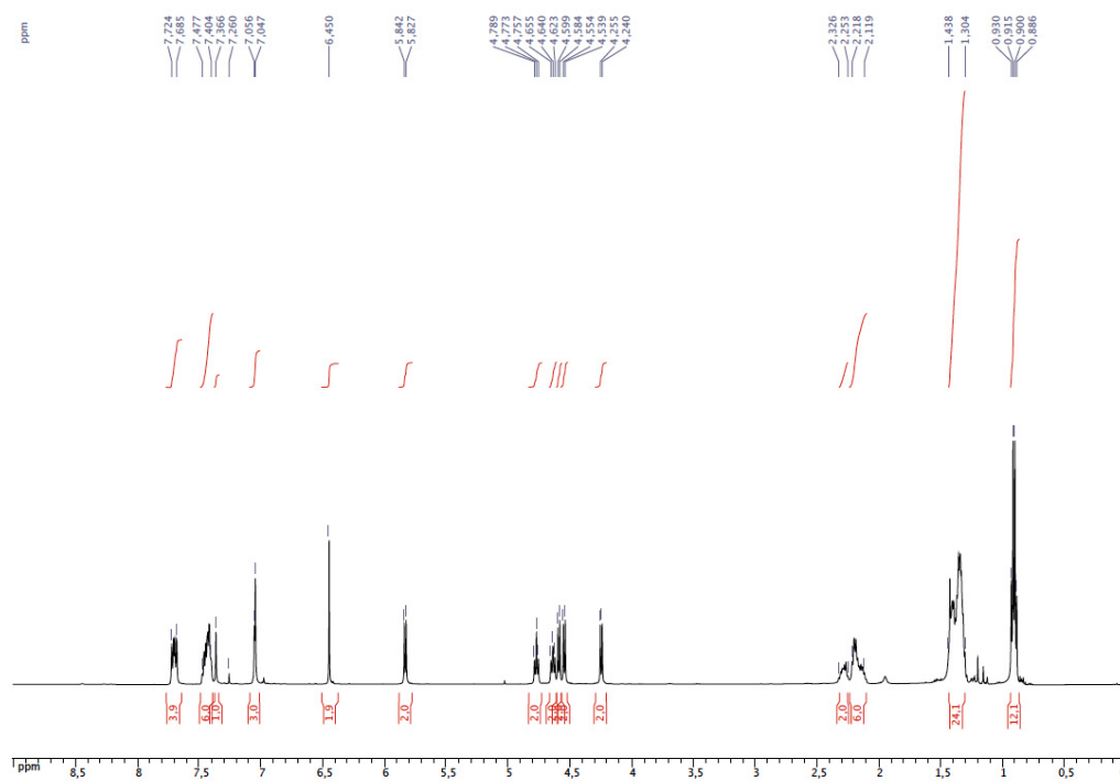
^1\text{H} NMR spectrum of 2 ( \text{CDCl}_3 )
