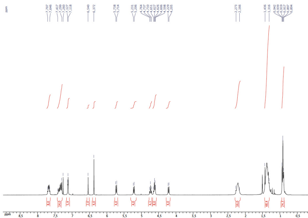
^1\text{H} NMR spectrum of 13 ( \text{CDCl}_3 )
