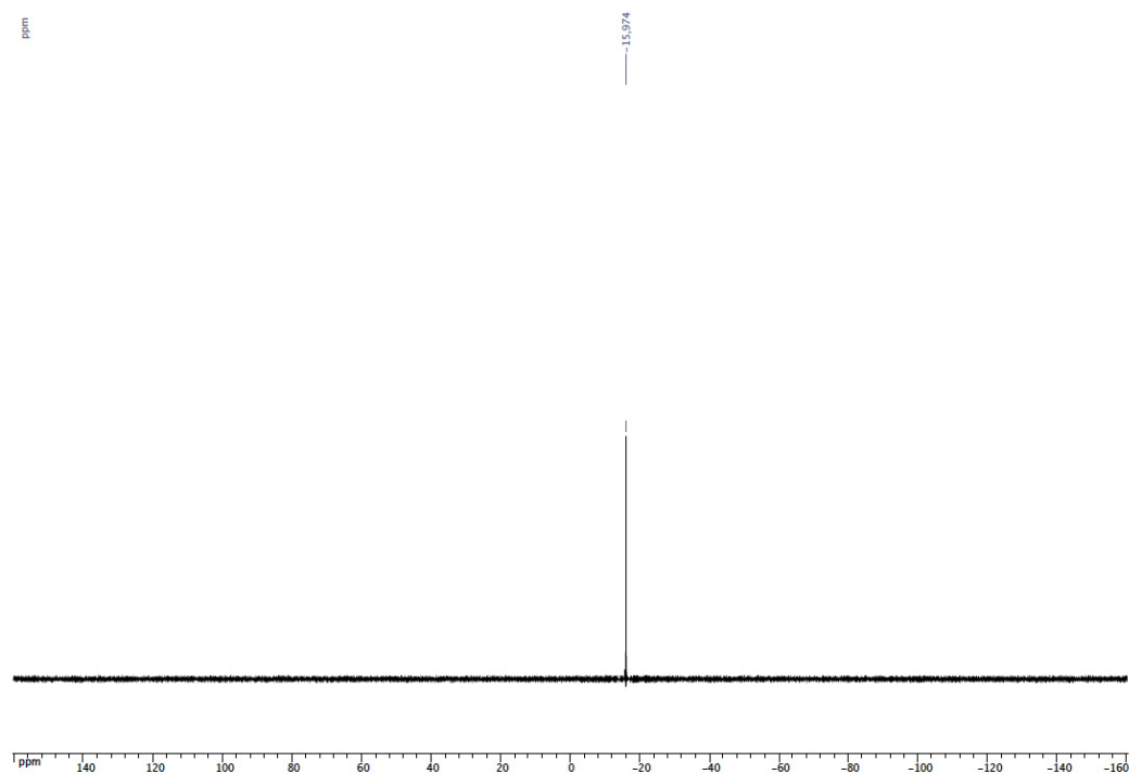
^{31}\text{P}\{^1\text{H}\} NMR spectrum of 6 ( \text{CDCl}_3 )
