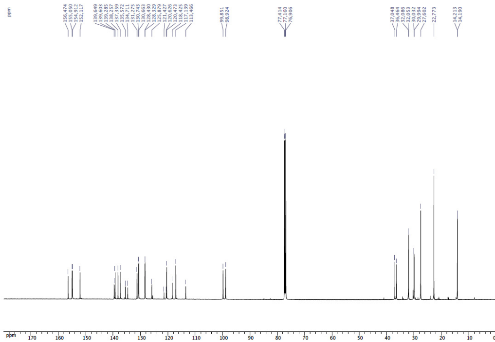
^{13}\text{C}\{^1\text{H}\} NMR spectrum of 2 ( \text{CDCl}_3 )
