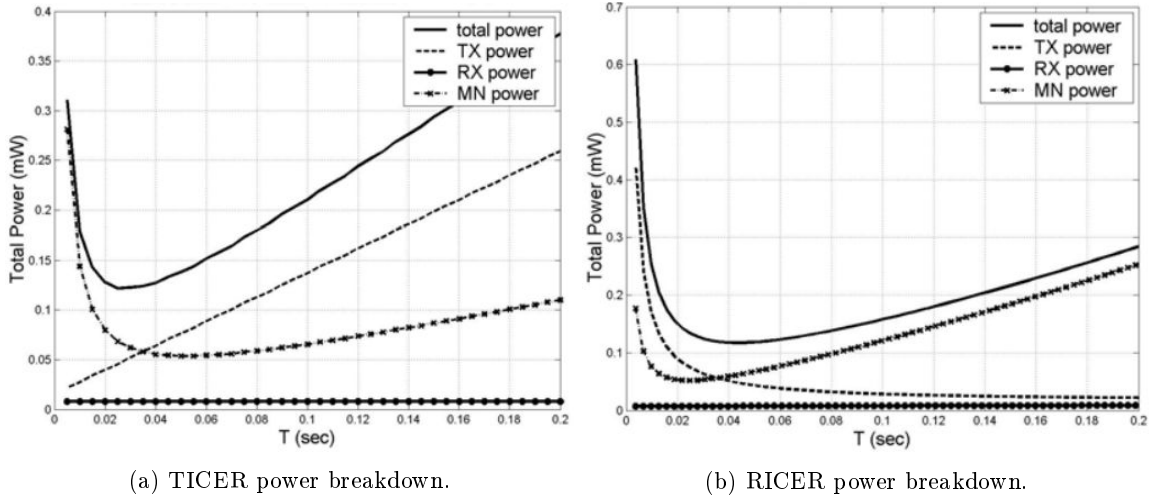
Figure 1.5 – TICSER and RICSER power breakdown, from [1]. TX: transceiver transmitting, RX: transceiver receiving, MN: transceiver sensing, T is the wake up interval, denoted by T_{WI} in this thesis.
