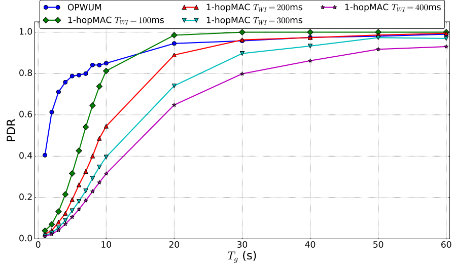
Figure 7.6 – Packet delivery ratio as a function of packet generation period T_g . The contention window D_c is set to 50 ms.
