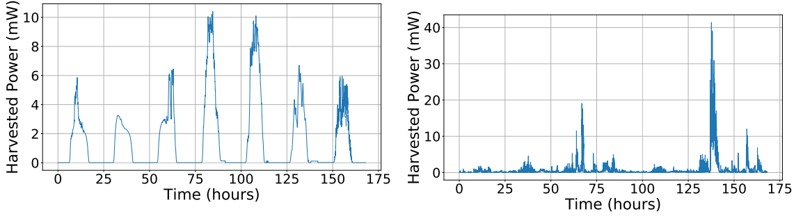
(a) Typical indoor ambient light power trace (from EnHANTs [78]). (b) Typical wind power trace (from NREL [79]).
