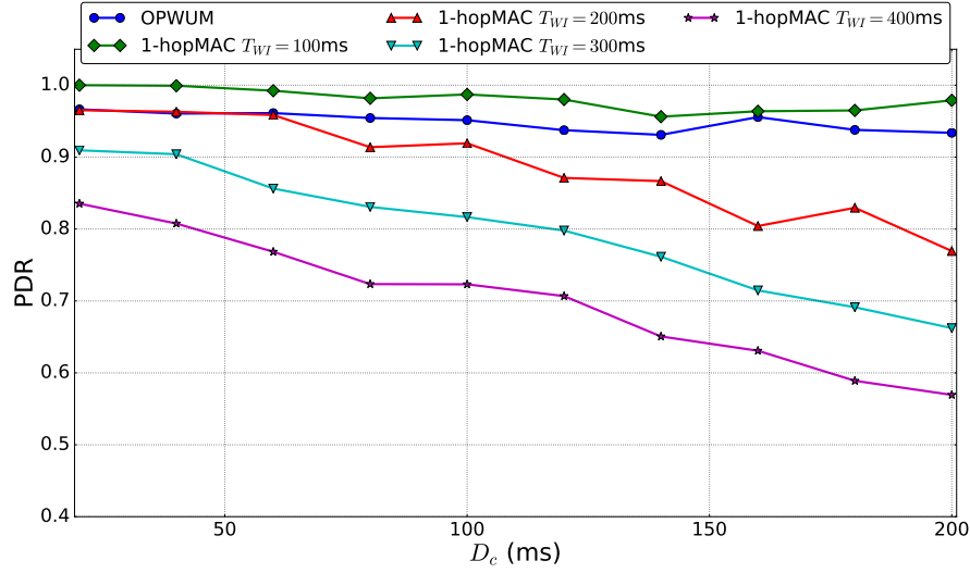
Figure 7.7 – Packet delivery ratio as a function of contention period duration D_c . The packet generation period T_g is set to 30 s.
