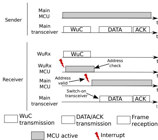
Figure 6.2 – Illustration of a packet transmission using TI WuR.
