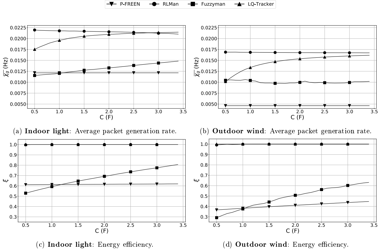
Figure 4.5 – Average packet generation rate and energy efficiency for different capacitance values, in the case of indoor light and outdoor wind.
