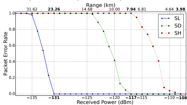
(b) LoRa TM sensitivity and theoretical range for different setups.
