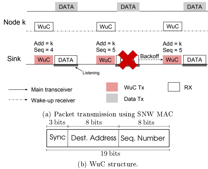
Figure 8.3 – SNW MAC packet transmission illustration and WuC format.
