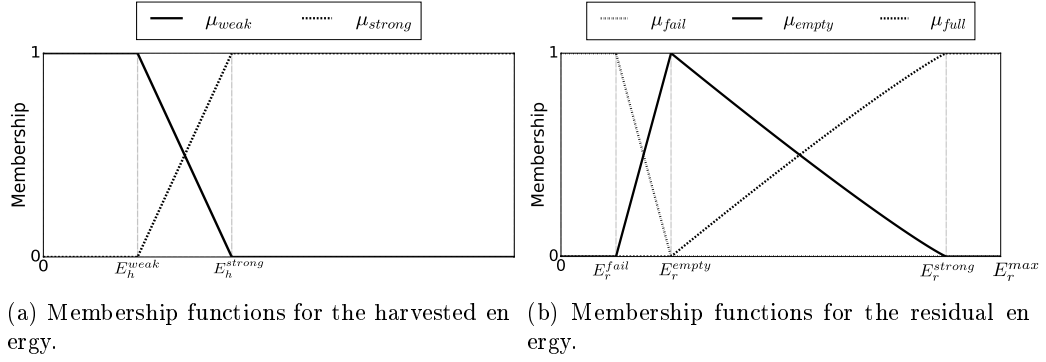
Figure 3.3 – Membership functions used by the fuzzification module.
