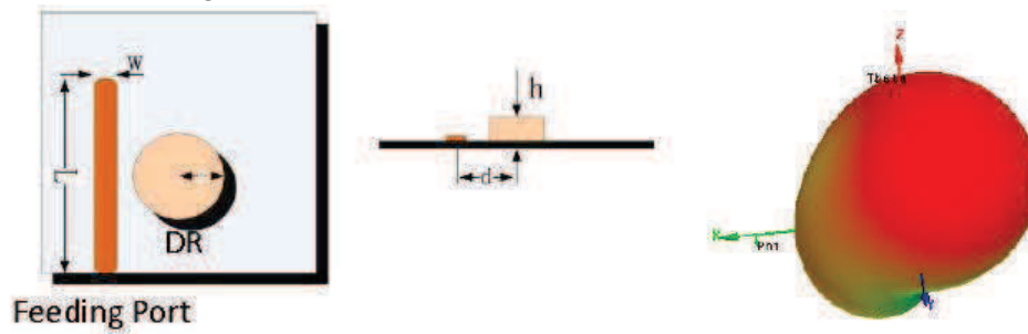
Figure 132: A single port of a cylindrical DRA and its radiation pattern
