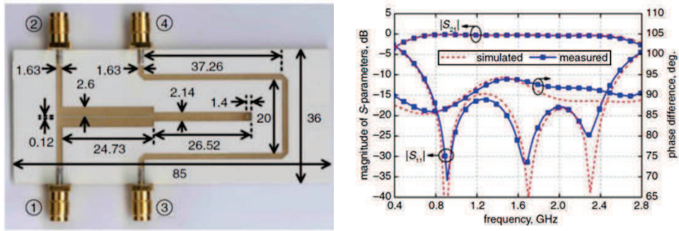
Figure 28: Switched line phase shifter for 90^\circ
