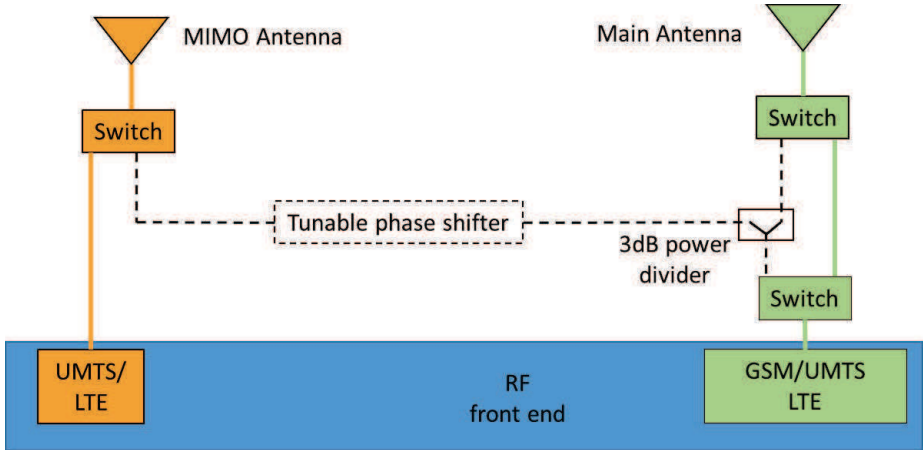
Figure 5: MIMO antenna system concept for LTE.
