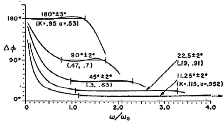
Figure 30: Reflection type phase shifter for 90^\circ
