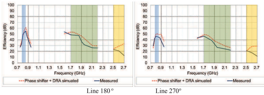
Figure 145: Performance of DRA with manual-switched lines
