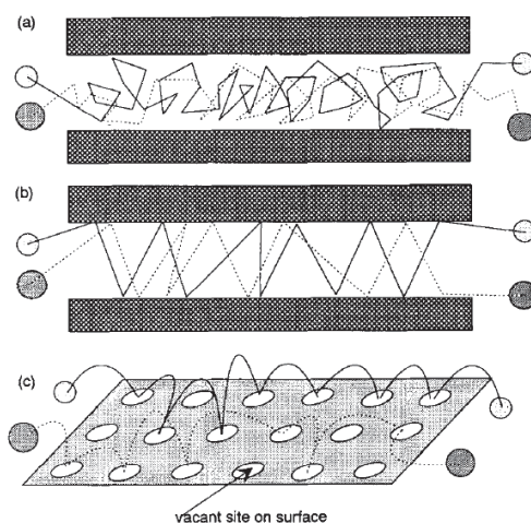
Figure 21 – Three main diffusion mechanisms: (a) Bulk diffusion, (b) Knudsen diffusion, (c) Surface diffusion [83]
