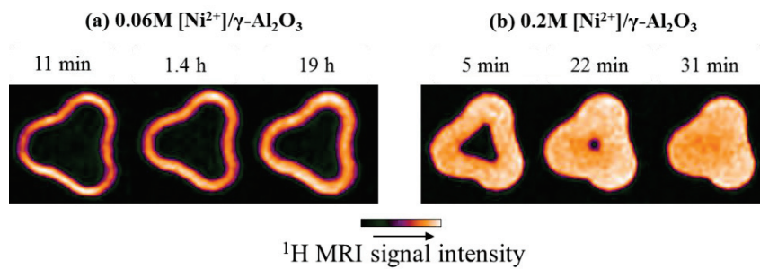
Figure 57 – ^1\text{H} MRI images corresponding to transport of (a) 0.06 M [\text{Ni}^{2+}] and (b) 0.2 M [\text{Ni}^{2+}] solution within the porosity of a \gamma\text{-Al}_2\text{O}_3 pellet obtained by a SPI sequence (FOV= 3\times 3\times 1 mm; Spatial resolution= 47\times 47\times 125 \mu\text{m}/\text{pixel} ; Matrix= 64\times 64\times 8 )
