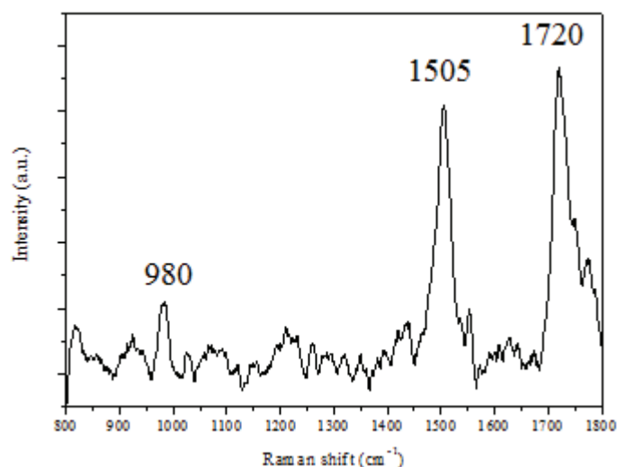
Figure B. 1 - Raman spectra recorded at different positions within a \gamma -alumina pellet
