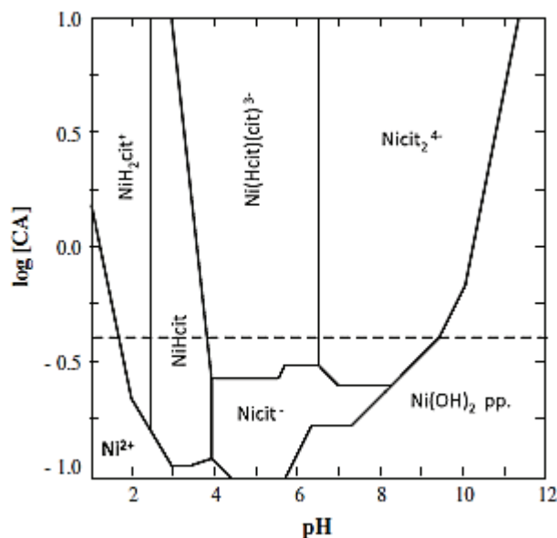
Figure 9 – Diagram for aqueous solution Ni(II)-CA ( [\text{Ni}(\text{II})_{\text{aq}}]=0.167\text{M} and [\text{CA}]_{\text{aq}}=0.437\text{M} ) [70]
