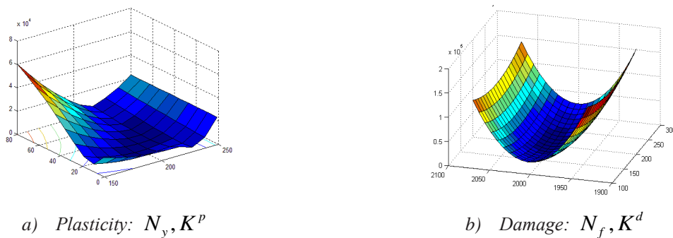
Figure 2.7 Shapes of the objective function for parameters in the second phase
