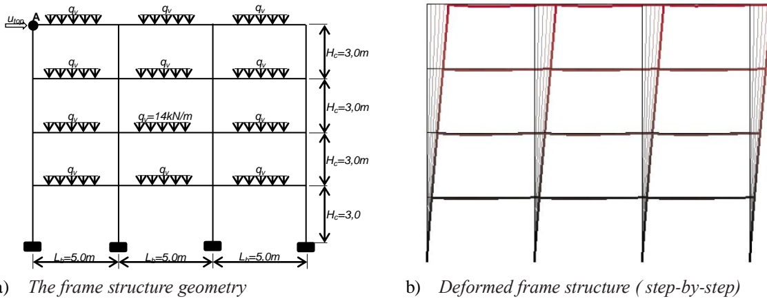
Figure 5.27 The symmetric steel frame
