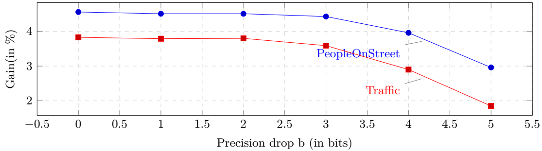
Figure 6.2 – BD-rate gain as function of the drop in precision bits
