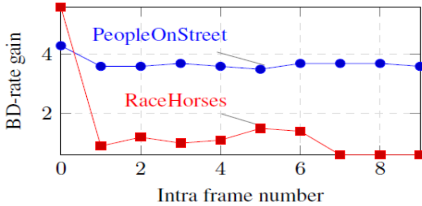
Figure 5.5 – BD-rate gain (in %, relatively to HEVC) at each intra frame
