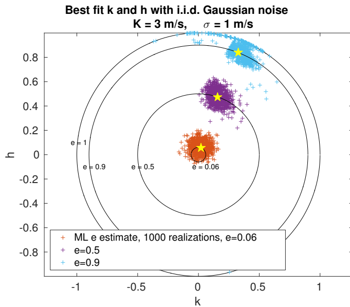
Figure 3.3: Estimates of k and h for true eccentricities e=0.06 , 0.5 and 0.9 when the noise standard deviation is \sigma=1 \text{ m}\cdot\text{s}^{-1} and K=3\text{m}\cdot\text{s}^{-1} (left) or K=1.5 \text{ m}\cdot\text{s}^{-1} (right).
