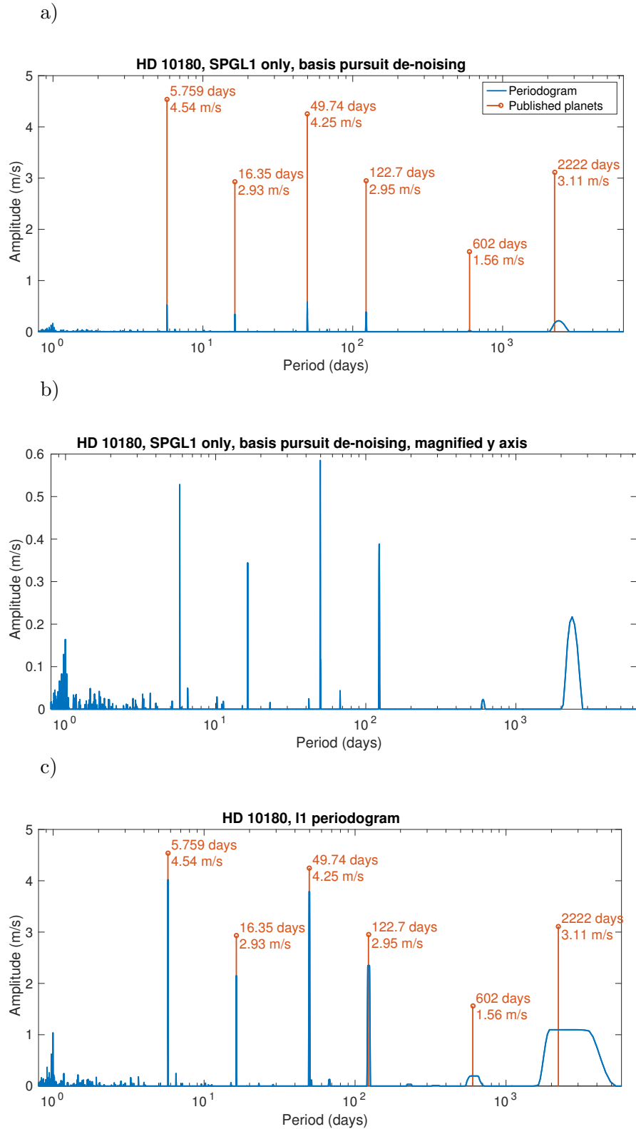
Figure 2.12: Basis pursuit denoising with SPGL1 (A has complex columns) a) Without normalization of the input of the solver nor averaging. b) Same figure as a) with zoom on the y axis c) “ \ell_1 -periodogram” with weighting by matrix \mathbf{W} , normalization of the input and averaging of the solution.
