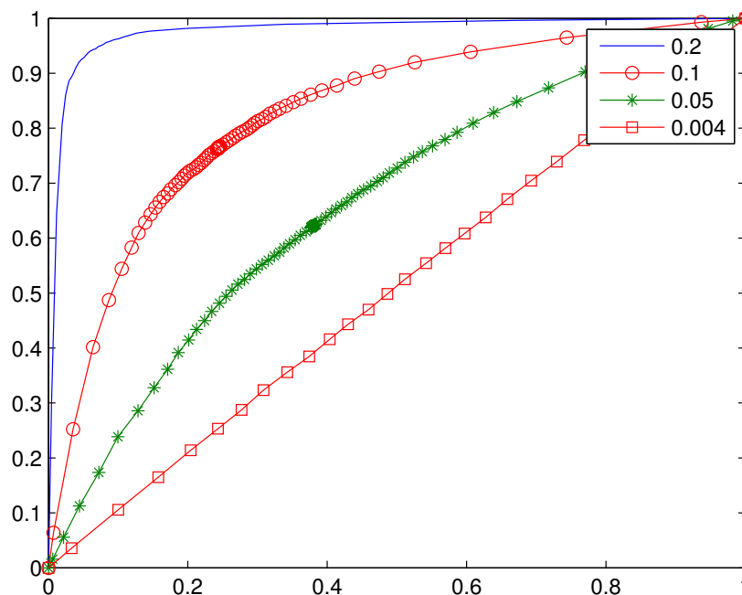
Fig. 2.1: ROC curves on different payloads.
