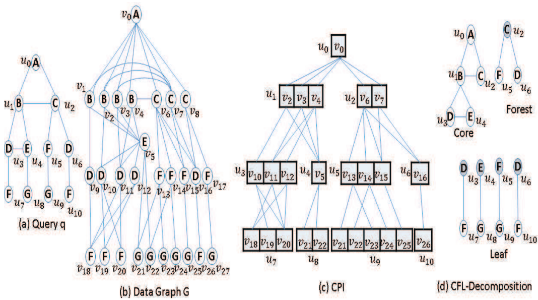
Figure 2.9: Running Example [6]
