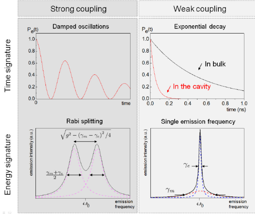
Figure 1.7 – Figure reproduced from [121]. The two regimes of the CQED system. Both the temporal and the spectral characteristics are shown for the strong coupling (left) and weak coupling (right) regime.
