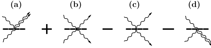
Figure 2.3 – Hong-Ou-Mandel interference between two single photons. The four figures represents the four possible outcomes of two photons impinging of a beam splitter: (a) the first reflected and the second transmitted, (b) both transmitted, (c) both reflected, (d) the first transmitted and the second reflected. When the two photons are indistinguishable the cases (b) and (c) destructively interfere.
