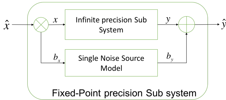
Figure 6.1 – Abstraction of the Single Noise Source model.
