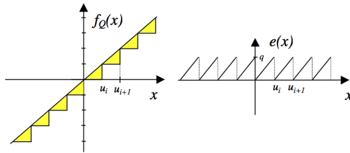
Figure 2.5 – Quantization process with truncation
