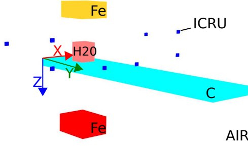
(a) Simulation model of the current OR layout considering the physical properties of each object.
