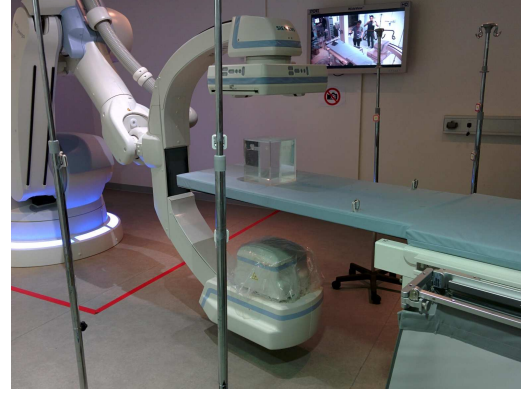
(b) Real-world setup: robotized C-arm, water-filled phantom and dosimeters sparsely distributed around the table.
