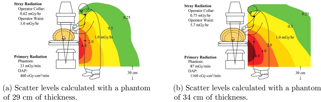
Figure 1.3: Effect of increasing patient abdomen thickness on operator exposure, courtesy of [Schueler 2006]. The drawings illustrate scattered radiation isodose curves calculated with a phantom simulating abdomen thicknesses. A 5 cm increase almost doubles staff exposure.
