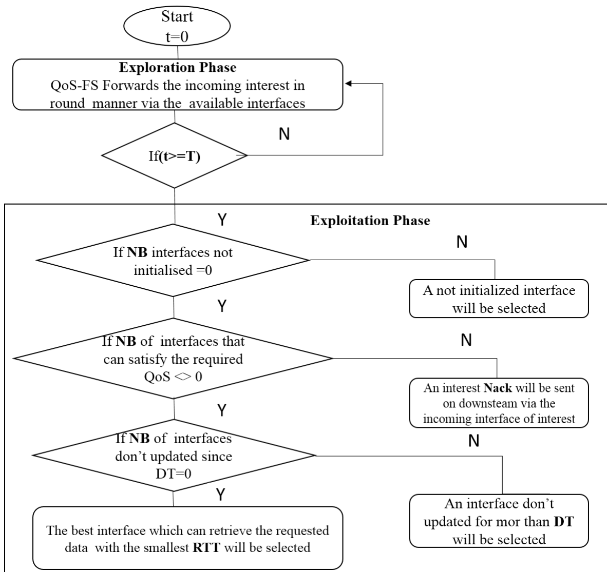
Figure 4.5: Exploration and exploitation phases.
