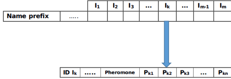
Figure 6.3: FIB entry data structure in MC-QoS-FS .
