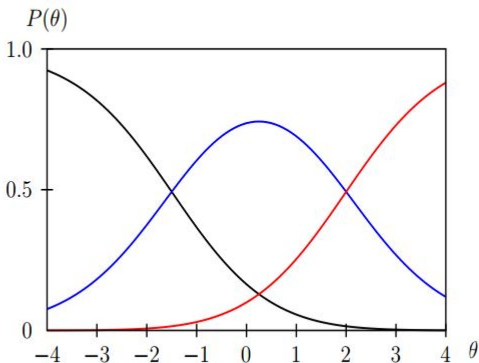
Figure 8: an example of a Category Characteristic Curve of a polytomous item.
