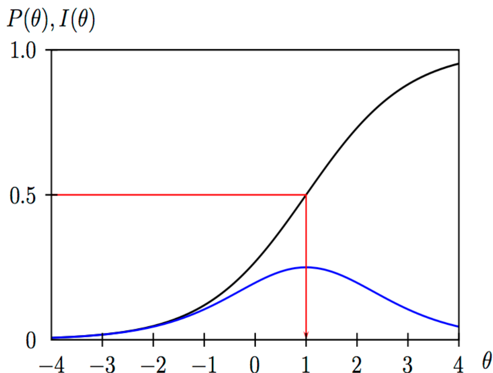
Figure 11: Item Characteristic Curve (in black) and item information function (in blue) of the 1-PL.
