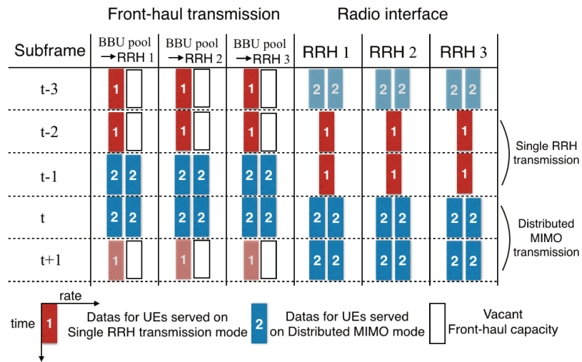
Fig. 7.4 Equal fronthaul transmission capacity constraint for the UEs served on Single transmission mode and in distributed MIMO mode.
