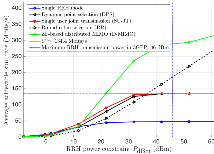
Fig. 5.13 Average achievable sum rate vs. RRH power constraint P_{\text{dBm}} ( \bar{C} = 134.4 Mbits/s, d_c = 0 m).
