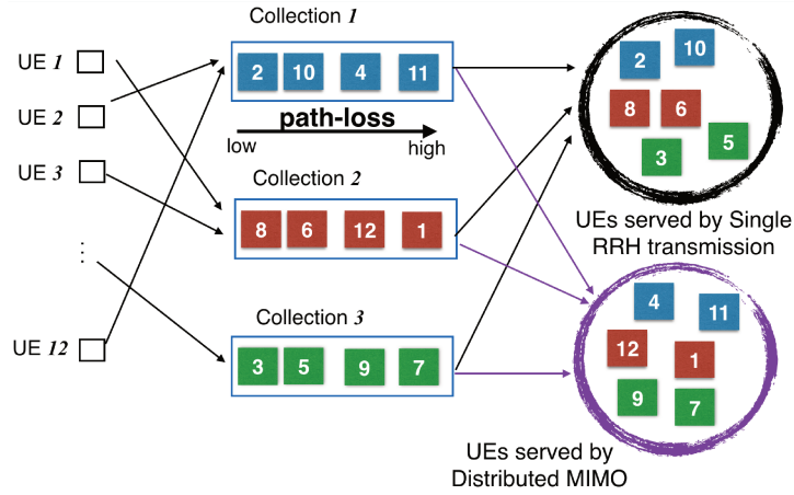
Fig. 7.3 Process of separating UEs to two parts, some served in single RRH mode and the others in distributed MIMO mode.
