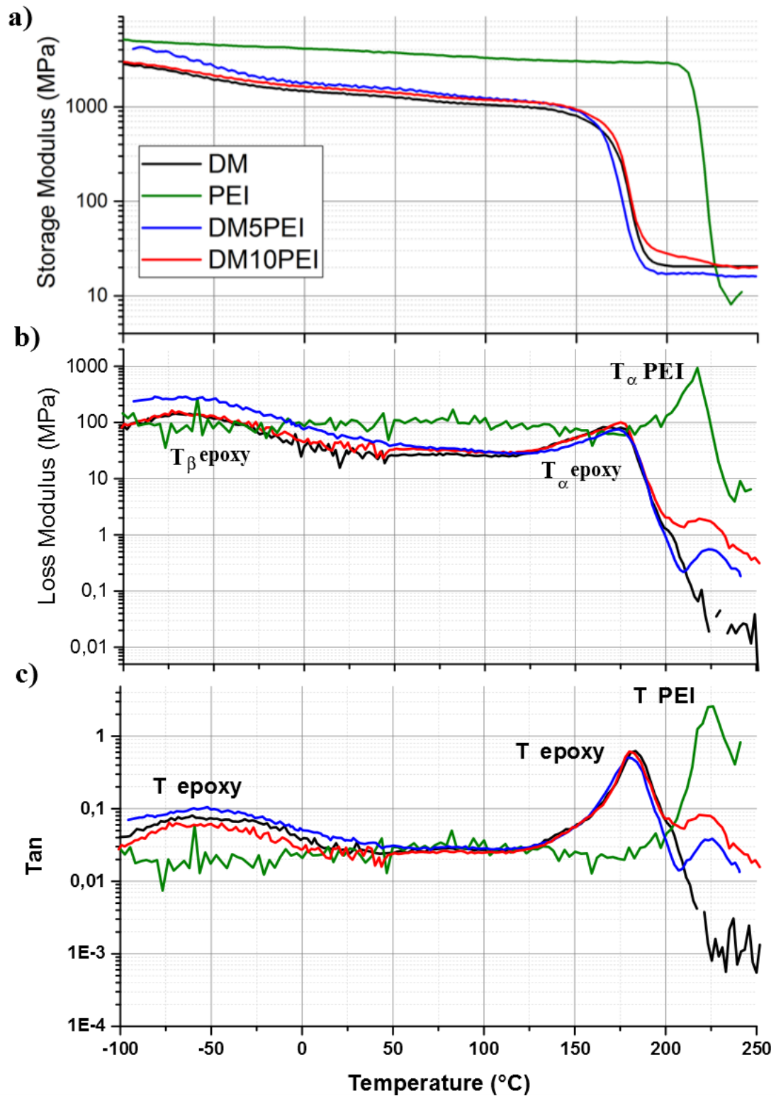
Figure 56: Storage Modulus E' (a) loss modulus (b) and loss factor \text{Tan } \delta (c) as function of temperature of DM, PEI, DM5PEI and DM10PEI at 1 Hz.
