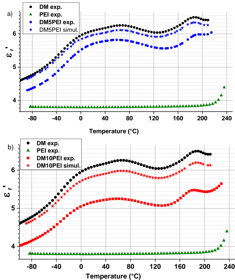
Figure 62: Experimental and effective modulated permittivity of (a) DM5PEI and (b) DM10PEI at 1 kHz
