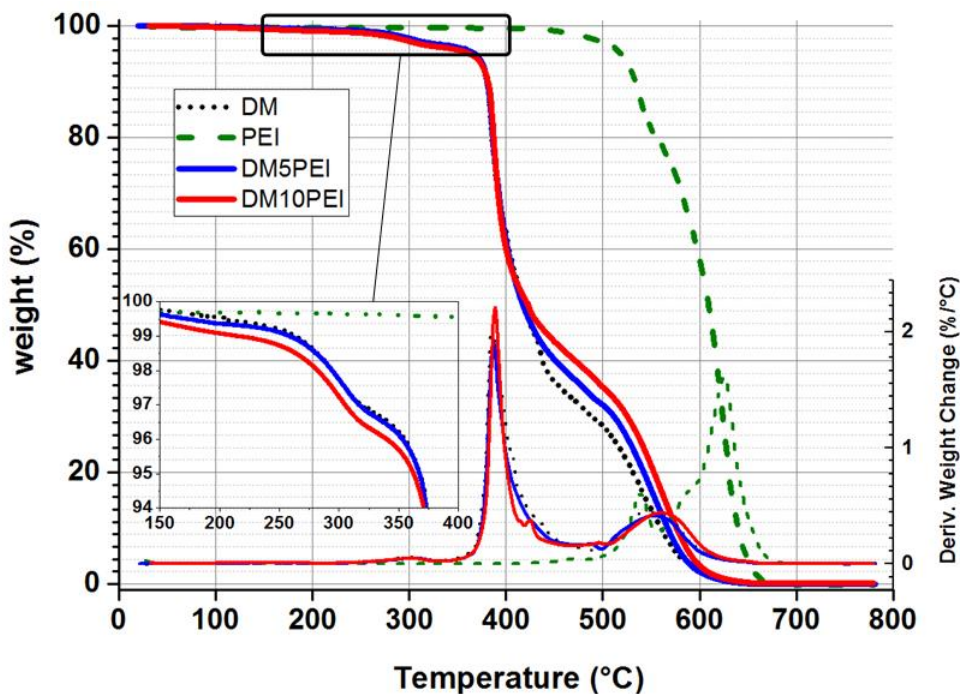
Figure 53: Weight loss and derivative of weight change of DM, PEI, DM5PEI and DM10PEI under air atmosphere. The inset is a zoom on the beginning of the degradation.
