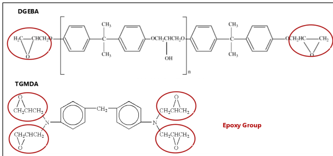
Figure 22: Different epoxy structures
