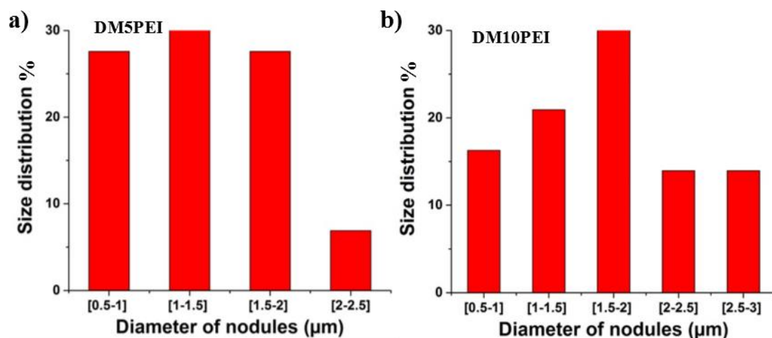
Figure 50: Size distribution of PEI nodules in the epoxy blends of a) DM5PEI and b) DM10PEI.
