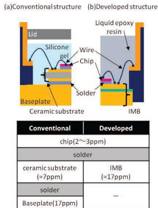
Figure 13: Cross-sectional views of IGBT modules proposed by Kaji et al. [Kaji'16]
