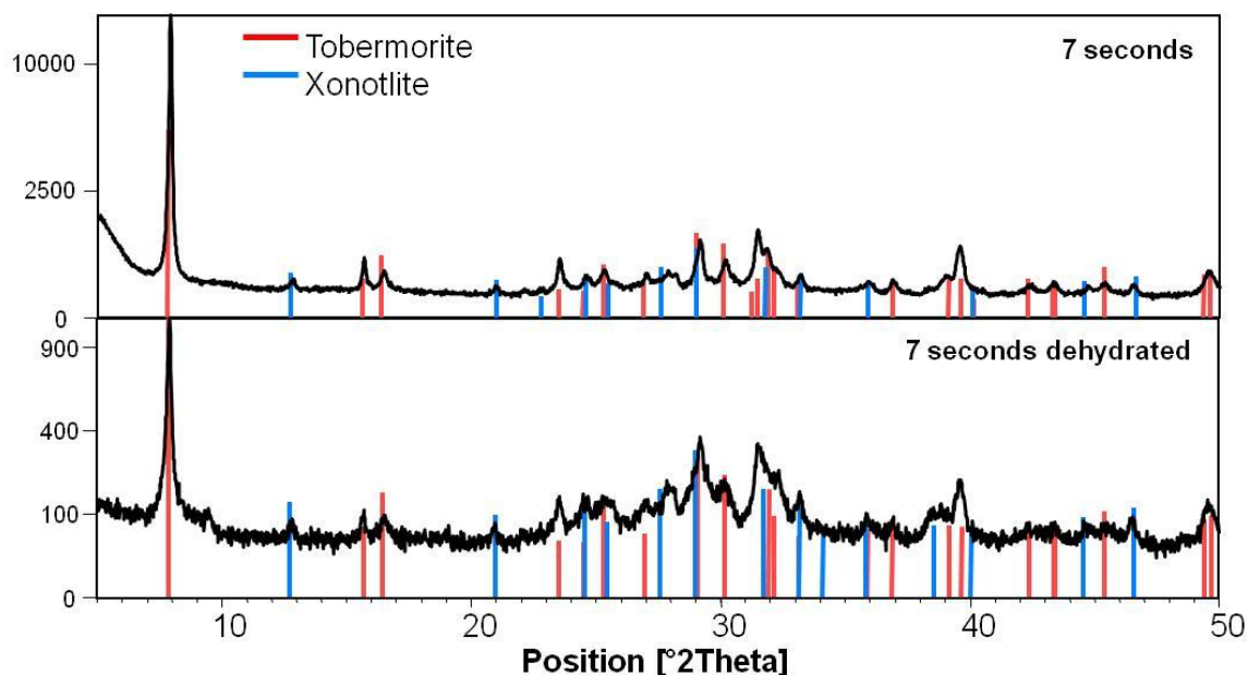
Figure III.2-24: XRD analysis of the supercritical tobermorite sample before and after the thermal treatment at 300°C.
