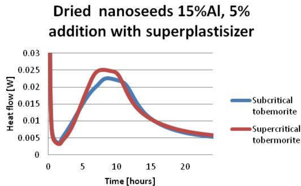
Figure IV.2-6: Calorimetric measurements of seeds synthesized under different conditions.
