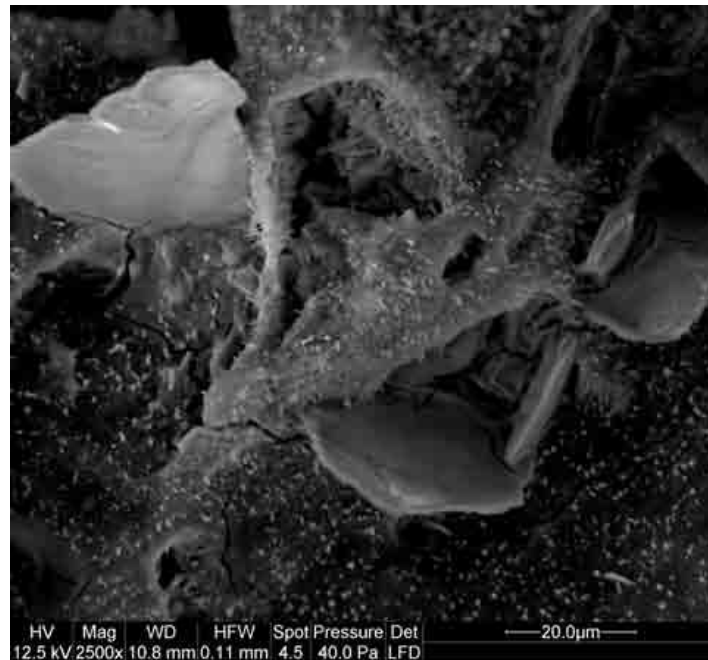
Figure I.1-8: SEM image of hydrated cement paste. [34]
