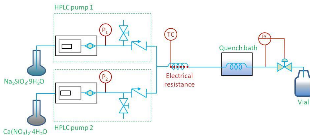
Figure III.2-4: First design done of the continuous hydrothermal supercritical reactor.
