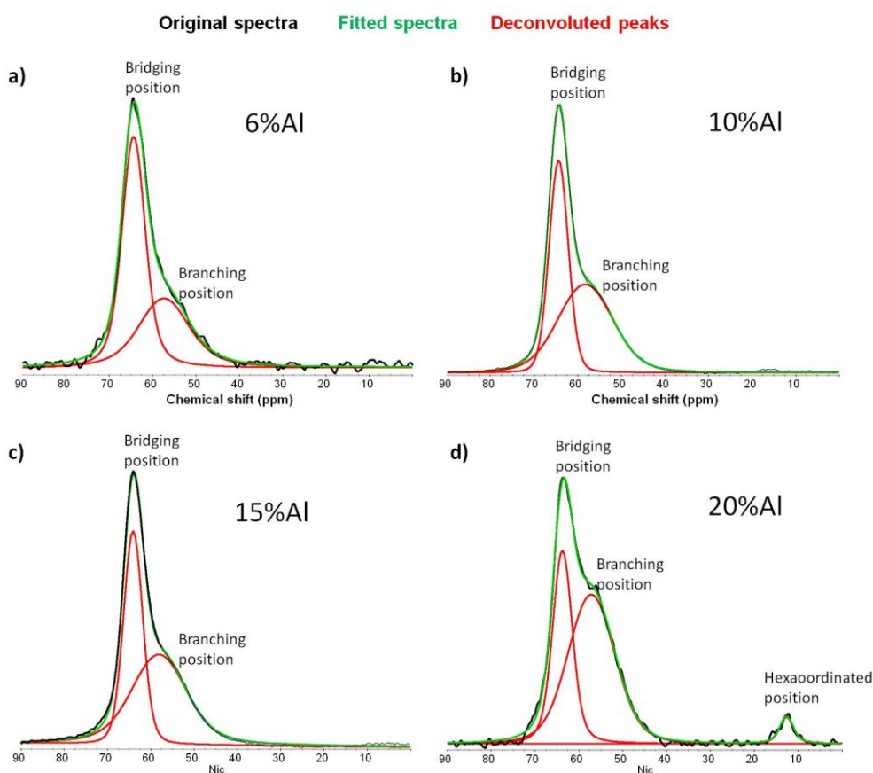
Figure III.1-23: Deconvolution of the ^{27}\text{Al} -MAS-NMR spectra. a) 6%Al normal tobermorite, b) 10%Al normal tobermorite, c) 15%Al normal tobermorite and d) 20%Al half-anomalous tobermorite.
