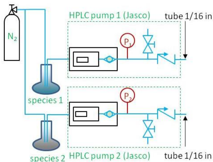
Figure III.2-7: Set-up 1c) with the modification in the inlet adding a nitrogen flow.
