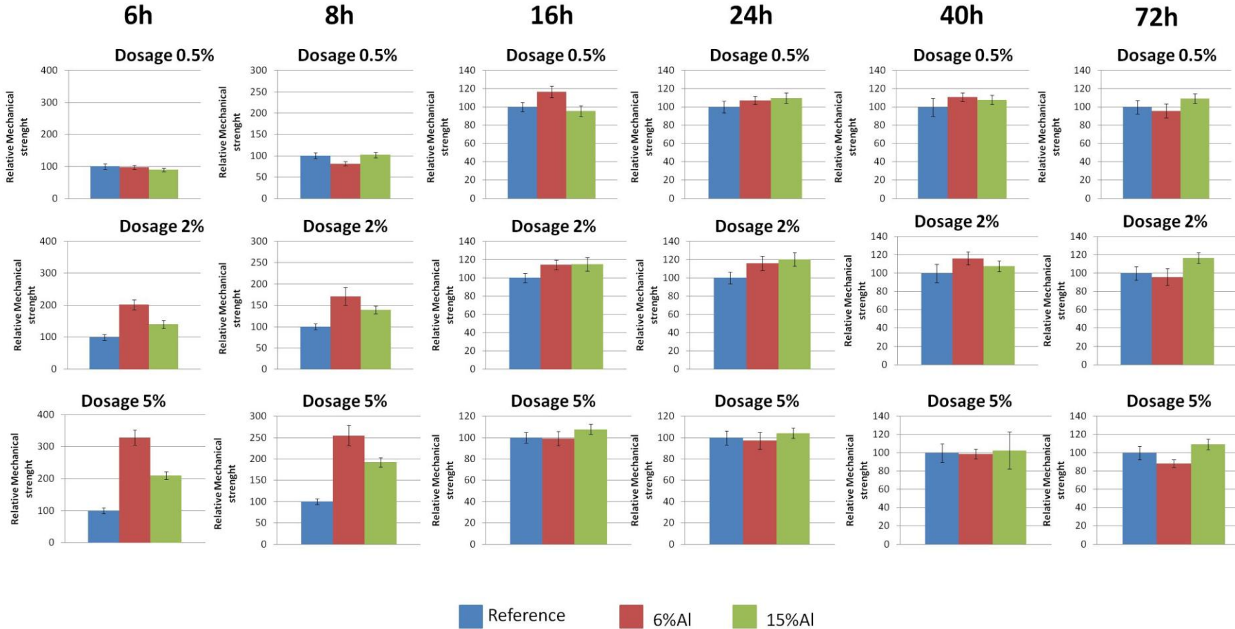
Figure IV.2-9: Compression test for dried samples of different times, dosages, and %AI. Comparison as function of the AI content.
