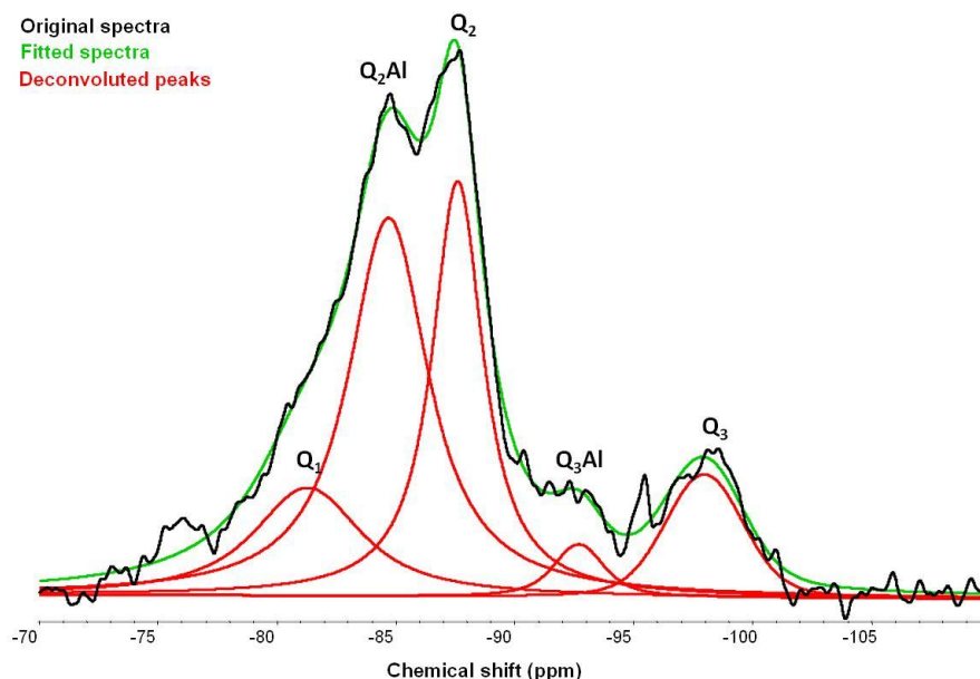
Figure III.2-23: ^{29}\text{Si} MAS-NMR spectrum of the supercritical tobermorite.
