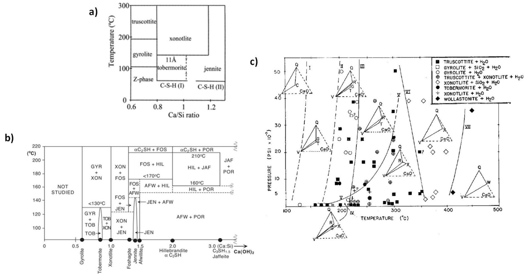
Figure I.3-3: a) CaO-SiO 2 -H 2 O phase diagram from Ca/Si of 0.6 to 1.3 and range of temperatures from 0°C to 300°C [77] , b) phase diagram obtained from several hydrothermal experiments, the dashed lines indicate uncertainties [140] and c) Phase boundaries of the CaO-SiO 2 -H 2 O system components as function of temperature and pressure. Q=quartz, C = CSH(I), T = tobermorite, G = gyrolite, R =truscottite, X = xonotlite, W = wollastonite, and V = H 2 O [137] .
