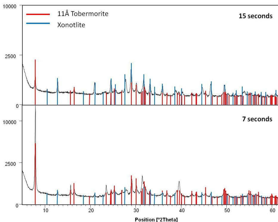
Figure III.2-17: XRD of the product obtained from the syntheses of tobermorite in the set-up 2 with 15 and 7 seconds of residence time respectively.
