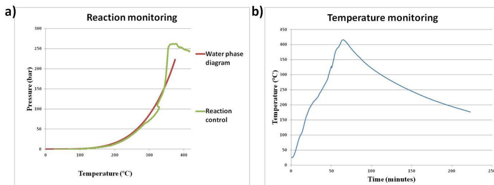
Figure III.2-25: Diagrams of the monitoring of the reaction, a) pressure/temperature and b) temperature/time
