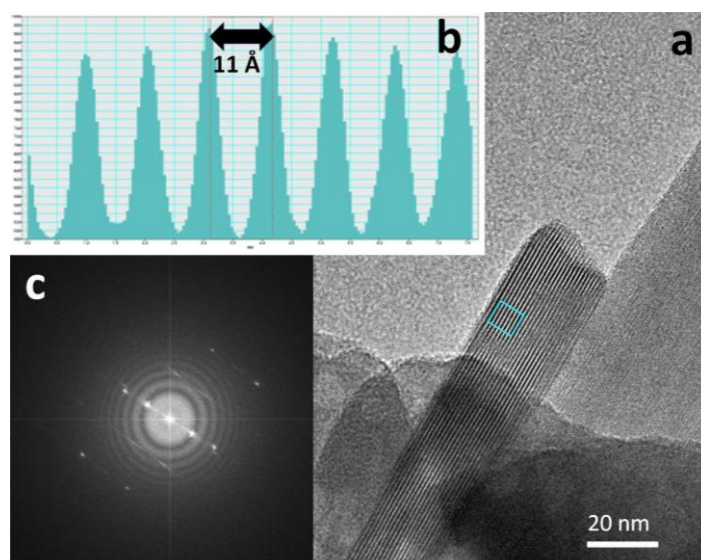
Figure III.2-22: TEM analysis of the 11Å tobermorite obtained under supercritical conditions. a) TEM image of a fiber, b) profile image representing the planes corresponding to the basal peak with a distance of 11Å between planes and c) FFT image of the fiber also representing the basal planes.
