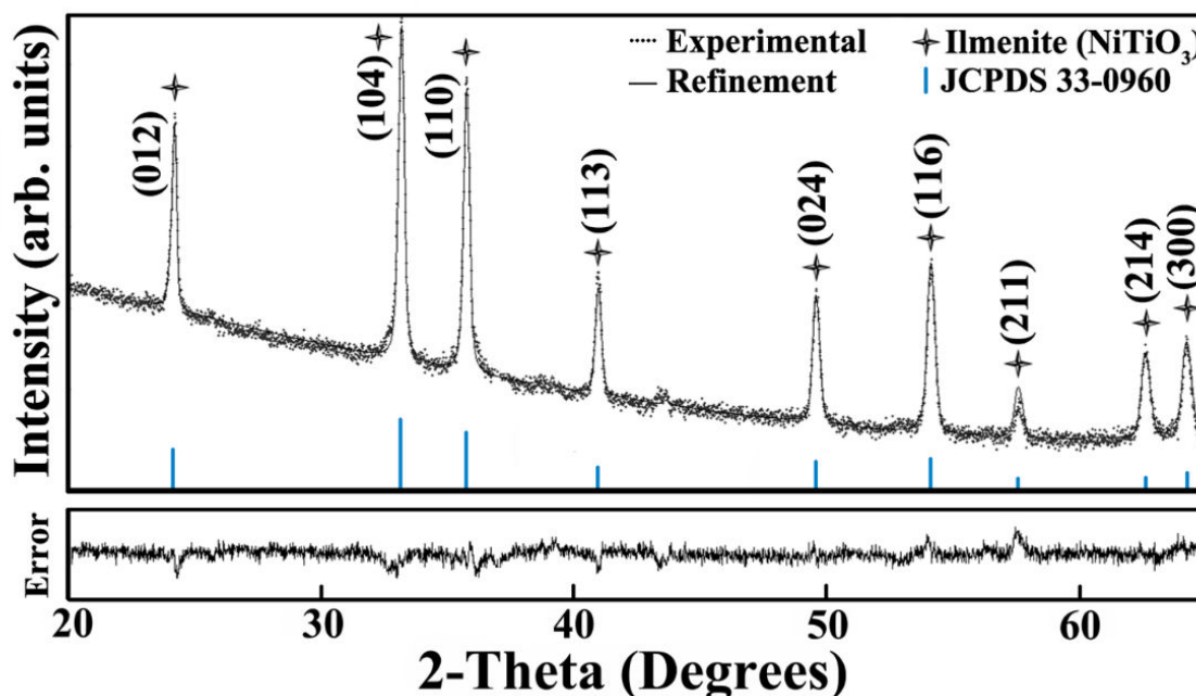
Fig. 6.2 XRD refinement of a representative \text{NiTiO}_3 thin film deposited on a Silicon substrate and annealed at 1000 °C for 2 hours in air as a pure ilmenite phase by using the Rietveld method. The standard reference JCPDS No. 33-0960 is shown.
