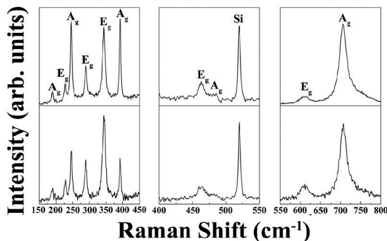
Fig. 5 Raman spectra collected from a representative NiTiO 3 thin film annealed at 1000 °C for 2 hours in air atmosphere using: parallel polarization (top) and cross polarization (bottom).
