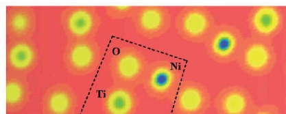
Fig. 3 Electron density projection in a selected plane of the NiTiO 3 ilmenite structure.
