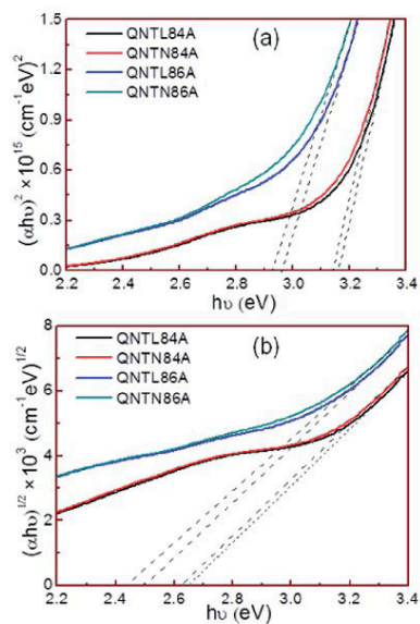
Fig. 10 Transformed absorption spectra of \text{NiTiO}_3 thin films deposited at different Ti power (200 W (QNTL84A) and 250 W (QNTL86A)) with nitrogen doping (QNTN84A and QNTN86A) showing (a) direct and (b) indirect band gap energies.
