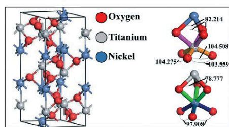
Fig. 3 Representation of the NiTiO 3 ilmenite unit cell and local environments of Ti and Ni.
