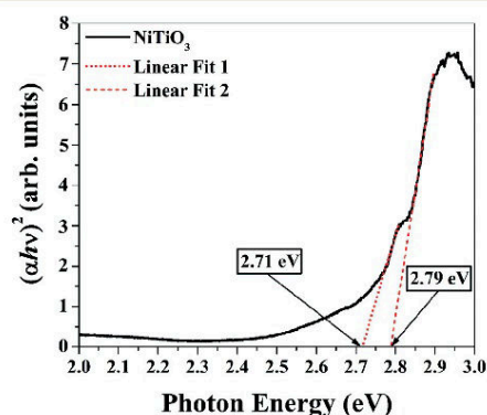
Fig. 8 Tauc plot of a NiTiO 3 thin film deposited on a quartz substrate; the film was annealed at 1000 °C under air and exhibits the ilmenite structure.
