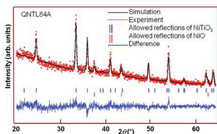
Fig. 3 Rietveld refinement for XRD pattern of NiTiO 3 thin film deposited at 200 W Ti power using FullProf software.
