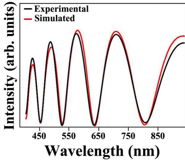
Fig. 6.8 Representation of the optical interferometry pattern made by a \text{NiTiO}_3 thin film annealed at 1000\text{ }^\circ\text{C} for 2 hours in air atmosphere. The values of the fit are summarized in Table 6.1.
