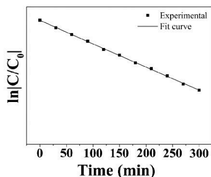
Fig. 10 Kinetics of the photocatalytic degradation of MB by visible light irradiated \text{NiTiO}_3 . The graph reports the semi-logarithmic plot of the normalized concentration C/C_0 versus irradiation time.
