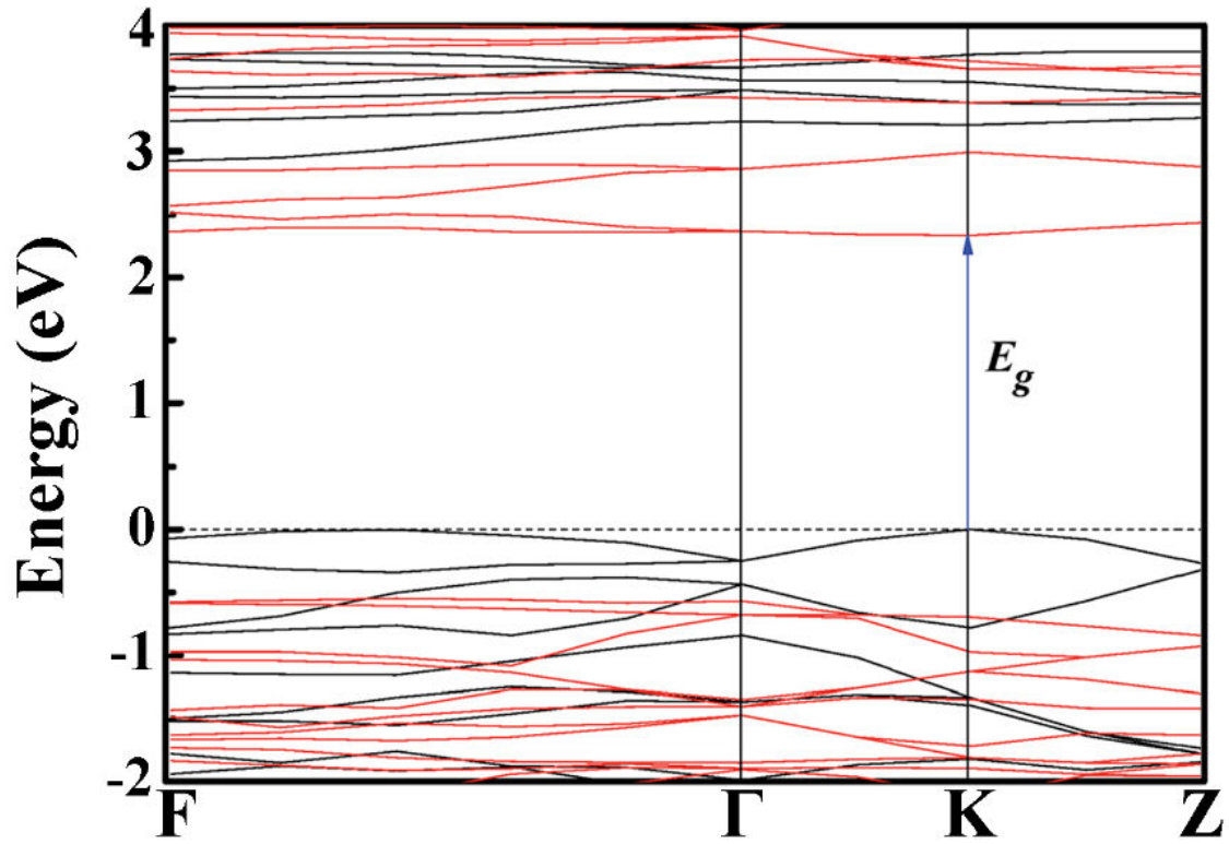
Fig. 2.4 Electron band structure calculated by the DFT/PBE functional within the Hubbard approximation U . The energy levels with spin polarized alpha electrons (black) and energy levels with a beta state (red) are shown.
