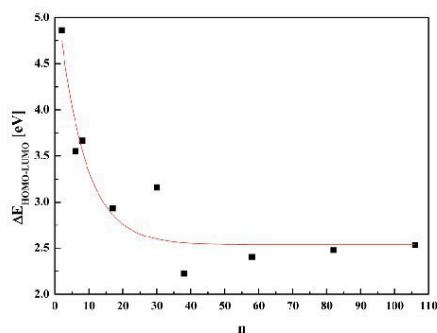
Fig. 6 Evaluation of the \Delta E_{\text{HOMO-LUMO}} energy splitting versus number n of (\text{NiTiO}_3)_n units calculated by the PM6 methodology.
