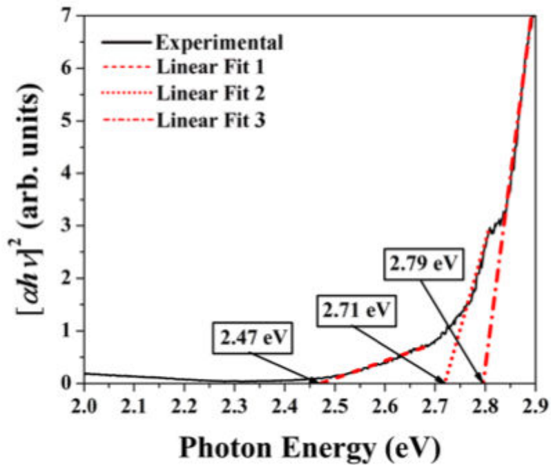
Fig. 6.9 Tauc plot of a \text{NiTiO}_3 thin film deposited on a quartz substrate; the film was annealed at 1000\text{ }^\circ\text{C} under air and exhibits the ilmenite structure.
