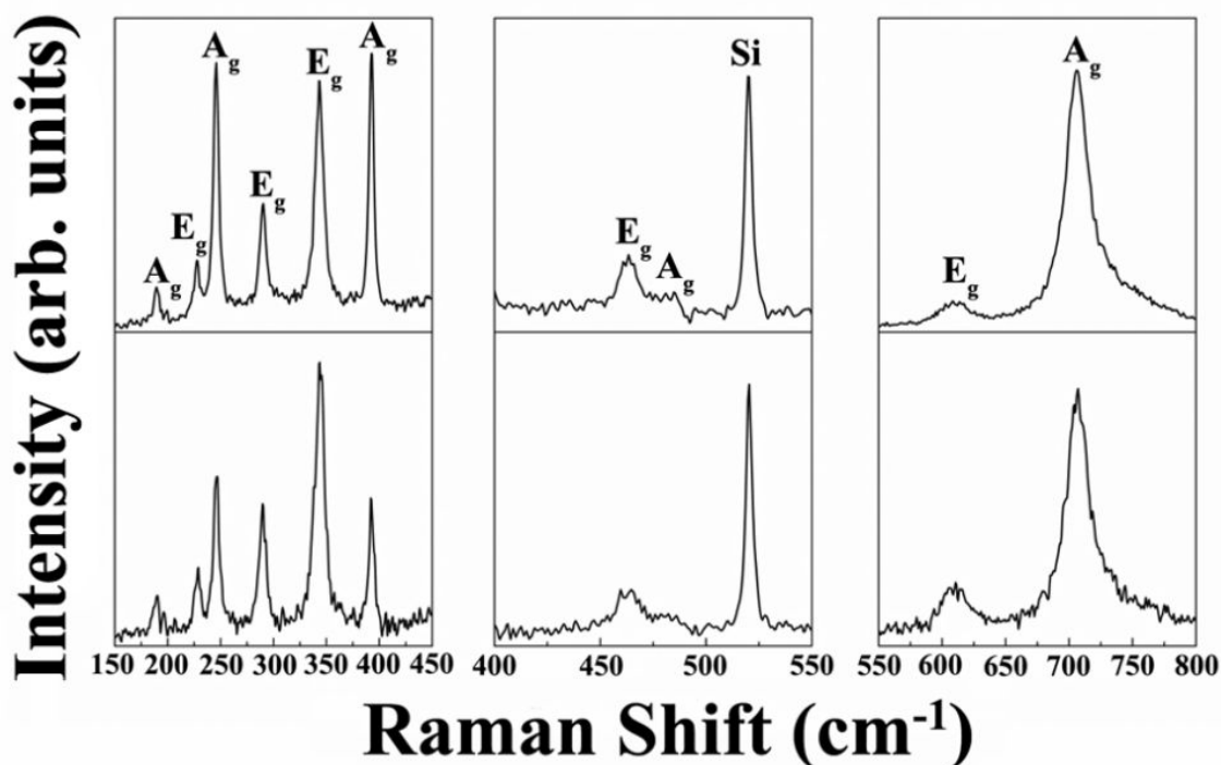
Fig. 6.6 Raman spectra collected from a representative NiTiO 3 thin film annealed at 1000 °C for 2 hours in air atmosphere using: parallel polarization (top) and cross polarization (bottom).
