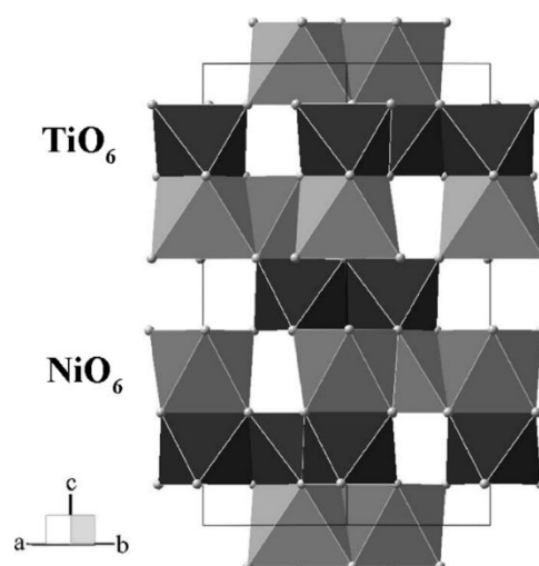
Fig. 8.4 Crystal structure of \text{NiTiO}_3 showing the \text{NiO}_6 (light gray) and \text{TiO}_6 (dark grey) octahedral.
