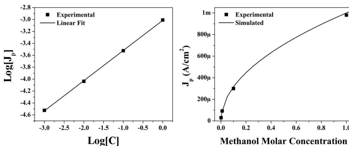
Fig. 7.6 Logarithm of peak current density ( J_p ) vs logarithm of methanol concentration ( C ) showing a linear behavior (left panel). Peak current density ( J_p ) vs methanol concentration ( C ) displaying the simulated behavior of peak current (right panel).
