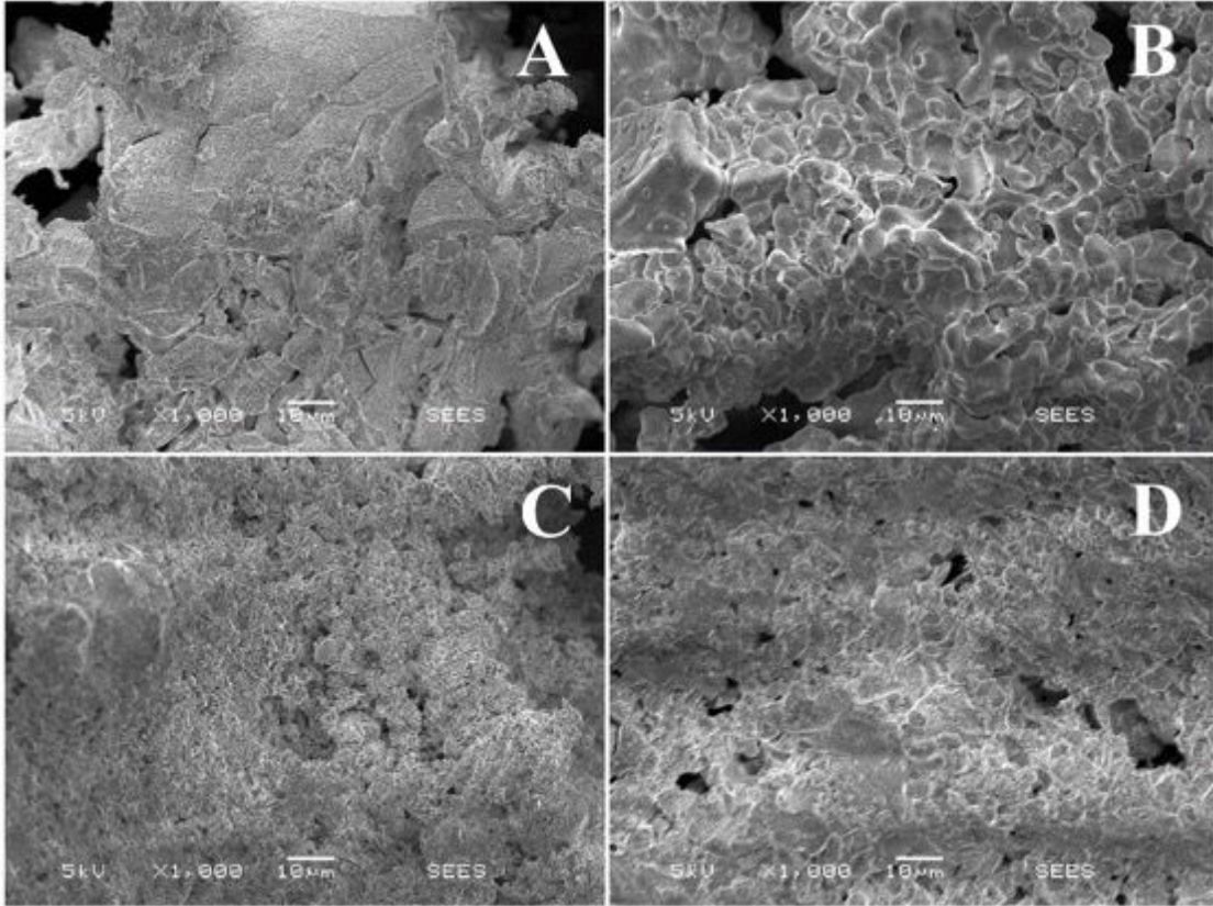
Fig. 4.1 SEM image of the surface of P1-SG-A1000C (A); P1-SG-A1350C (B); P2-SSR-A1000C (C); P2-SSR-A1350C (D). Acceleration voltage set to 5kV, objective set to \times 1000 , and the reference shown is 10 \mu\text{m} .
