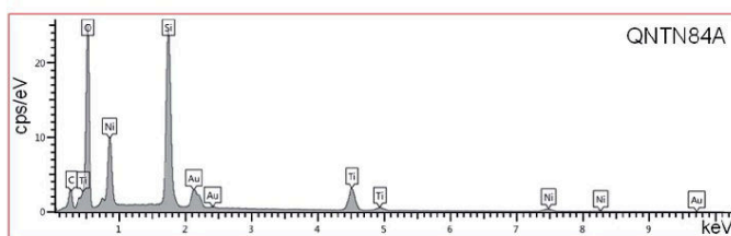
Fig. 6 EDAX spectrum of NiTiO 3 thin film deposited at 200 W Ti power with nitrogen doping.
