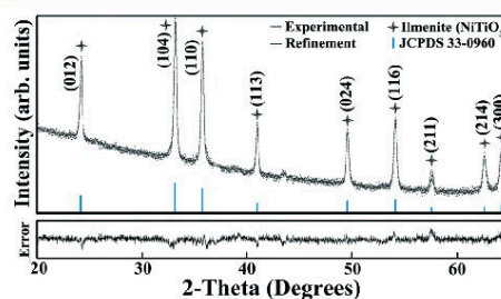
Fig. 2 XRD refinement of a representative NiTiO 3 thin film annealed at 1000 °C for 2 hours in air as a pure ilmenite phase by using the Rietveld method. The standard reference JCPDS No. 33-0960 is shown.
