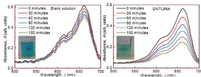
Fig. 11 Absorption changes of MB solution on blank (without sample) and \text{NiTiO}_3 thin films deposited at 250 W Ti power without nitrogen doping. A photograph of MB solution in the inset shows the de-colorization of the solution before and after the reaction.
