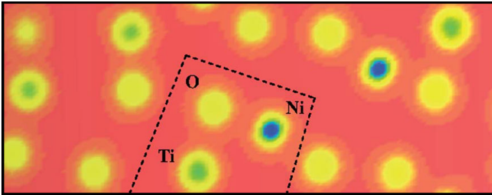
Fig. 2.3 Electron density projection in a selected plane of the NiTiO 3 ilmenite structure.
