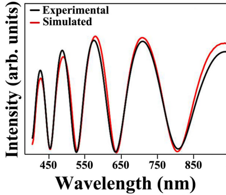
Fig. 6.8 Representation of the optical interferometry pattern made by a \text{NiTiO}_3 thin film annealed at 1000^\circ\text{C} for 2 hours in air atmosphere. The values of the fit are summarized in Table 6.1.
