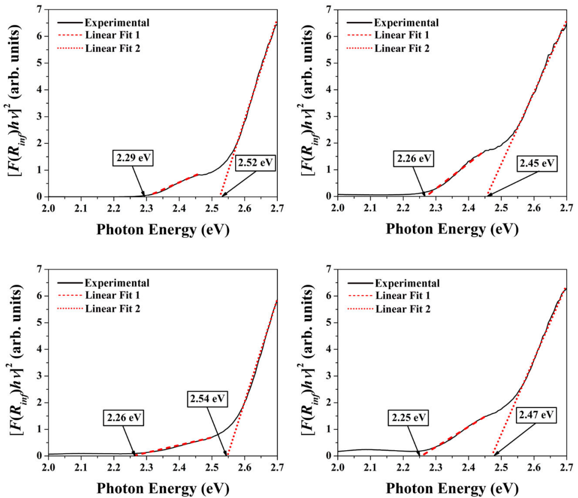
Fig. 4.5 Tauc plots of P1-SG-A1000C (top left), P1-SG-A1350C (top right), P2-SSR-A1000C (bottom left) and P2-SSR-A1350C (bottom right).
