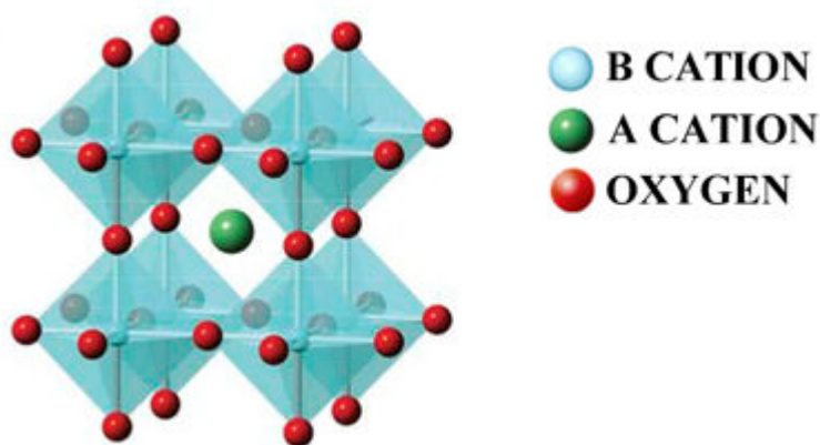
Fig. 1.1 ABO_3 perovskite crystal structure.
