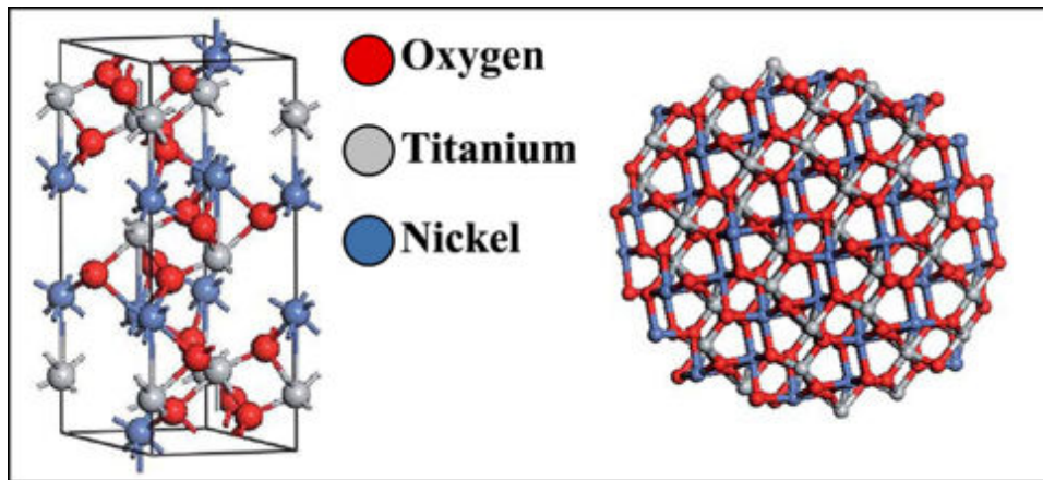
Fig. 2.1 The unit cell of crystalline \text{NiTiO}_3 (left) and the unpassivated nanocrystalline structure made by the formula (\text{NiTiO}_3)_{82} (right).
