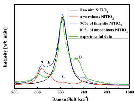
Fig. 9 Raman spectra for the (\text{NiTiO}_3)_{17} nanoparticles calculated by the parametrised PM6 method as well as experimental spectrum.
