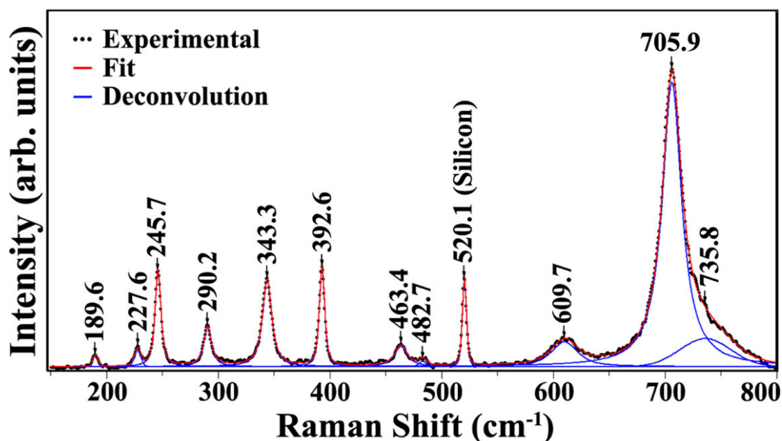
Fig. 8.6 Experimental and simulation of the Raman spectrum of the representative \text{NiTiO}_3 thin film annealed at 1000^\circ\text{C} for 2 hours in air atmosphere.
