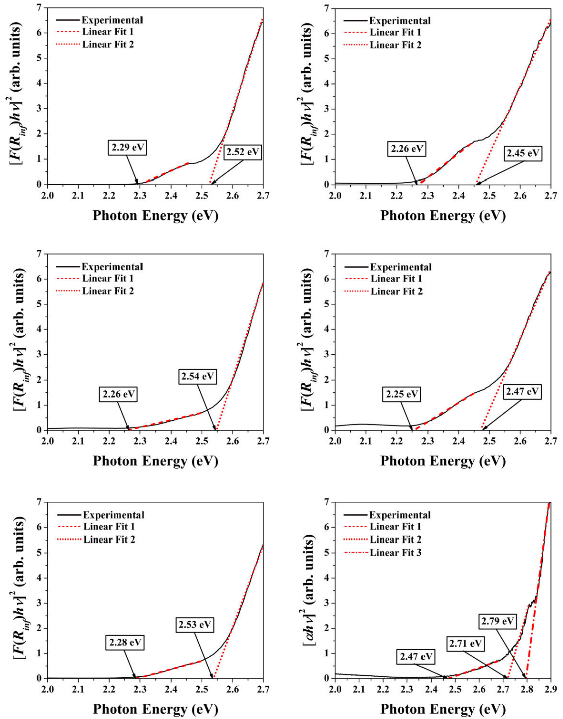
Fig. 8.4 Tauc plots of P1-SG-A1000C (top left), P1-SG-A1350C (top right), P2-SSR-A1000C (middle left), P2-SSR-A1350C (middle right), P3-SG-A650C (bottom left) and Thin Film (bottom right).
