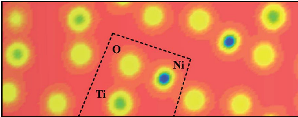
Fig. 2.3 Electron density projection in a selected plane of the NiTiO 3 ilmenite structure.
