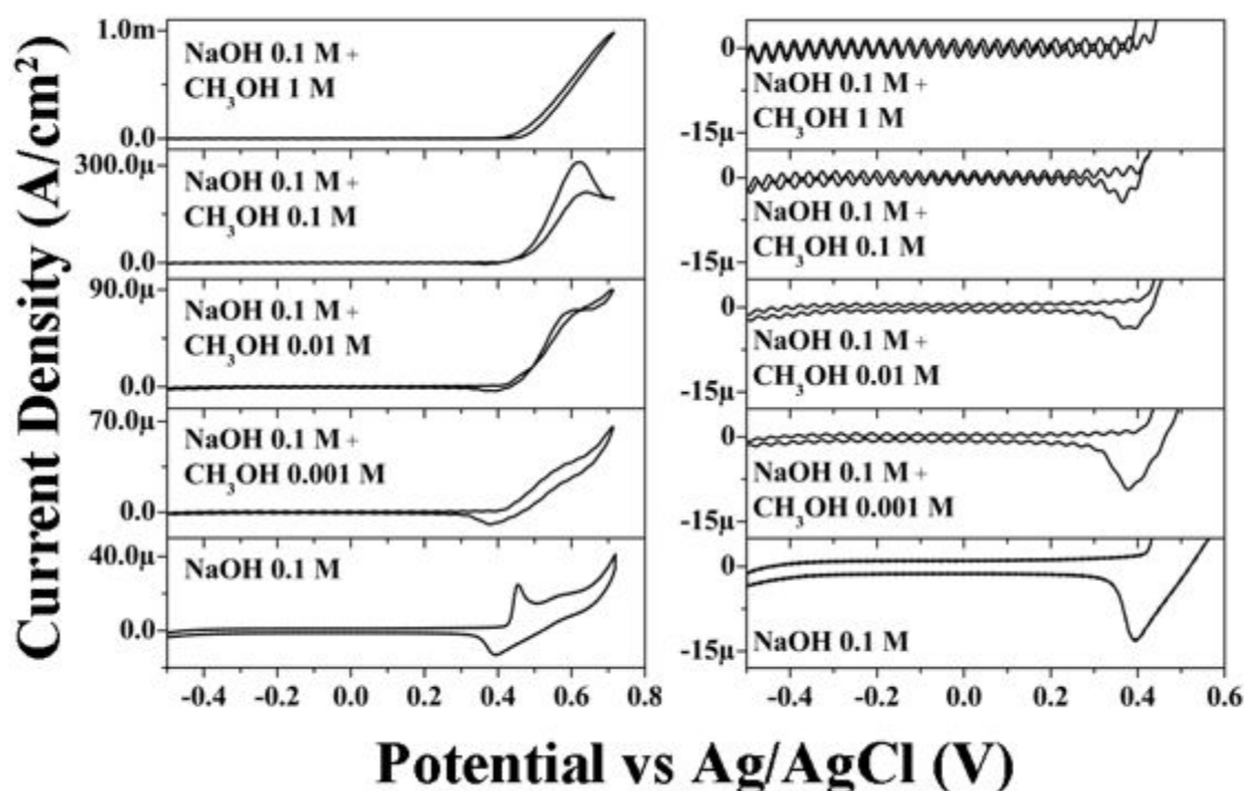
Fig. 7.5 Cyclic Voltammetry of the P3-SG-A650C in the presence of Methanol. The activation in NaOH 0.1 M is showed as a reference. NaOH 0.1 M + Methanol 0.001 M, 0.01 M, 0.1 M and 1 M are displayed. The left-hand panel shows the reactions taking place. The right-hand panel allows to observe the change in intensity of the cathodic peak at 0.4 V with respect to methanol concentration. Scan rate 20 mV/s.
