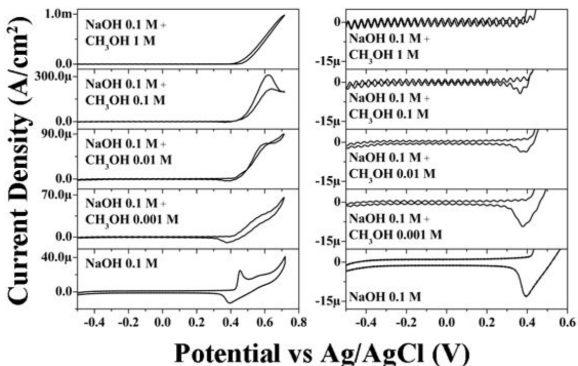
Fig. 7.5 Cyclic Voltammetry of the P3-SG-A650C in the presence of Methanol. The activation in \text{NaOH} 0.1 M is showed as a reference. \text{NaOH} 0.1 M + Methanol 0.001 M, 0.01 M, 0.1 M and 1 M are displayed. The left-hand panel shows the reactions taking place. The right-hand panel allows to observe the change in intensity of the cathodic peak at 0.4 V with respect to methanol concentration. Scan rate 20 mV/s.
