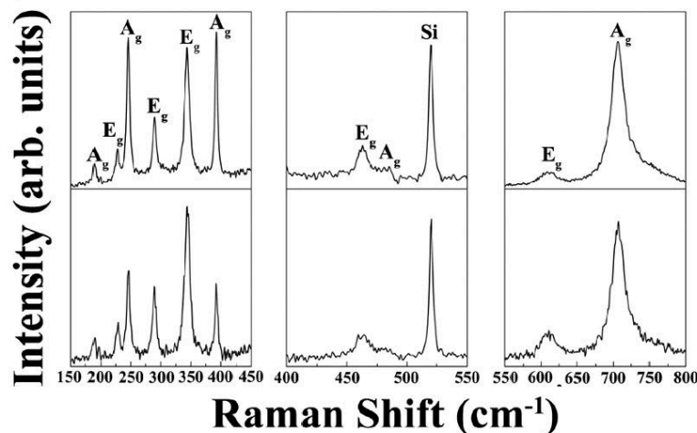
Fig. 5 Raman spectra collected from a representative \text{NiTiO}_3 thin film annealed at 1000^\circ\text{C} for 2 hours in air atmosphere using: parallel polarization (top) and cross polarization (bottom).
