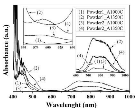
Fig. 6. Absorbance spectra of the samples, obtained from diffuse reflectance spectra.
