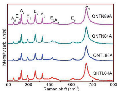
Fig. 4 Raman spectra of NiTiO 3 thin films deposited at different Ti power (200 W (QNTL84A) and 250 W (QNTL86A)) with nitrogen doping (QNTN84A and QNTN86A).
