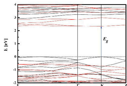
Fig. 4 Electron band structure calculated by the DFT/PBE functional within the Hubbard approximation U . The energy levels with spin polarized alpha electrons (black) and energy levels with a beta state (red) are shown.
