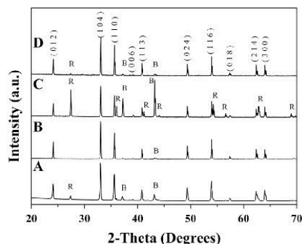
Fig. 2. XRD patterns of NiTiO 3 Powder1 and Powder2, annealed at different temperatures in air atmosphere. The letter “R” refers to the Rutile phase of TiO 2 and “B” to the Bunsenite phase of NiO. (A) Powder1_A1000C. (B) Powder1_A1350C. (C) Powder2_A1000C. (D) Powder2_A1350C.
