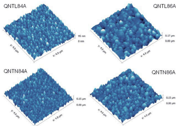
Fig. 8 AFM images of \text{NiTiO}_3 thin films deposited at 200 and 250 W Ti power with nitrogen doping.
