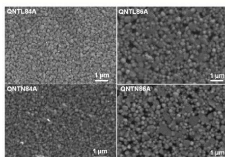
Fig. 5 SEM micrographs of NiTiO 3 thin films deposited at 200 and 250 W Ti power with nitrogen doping.
