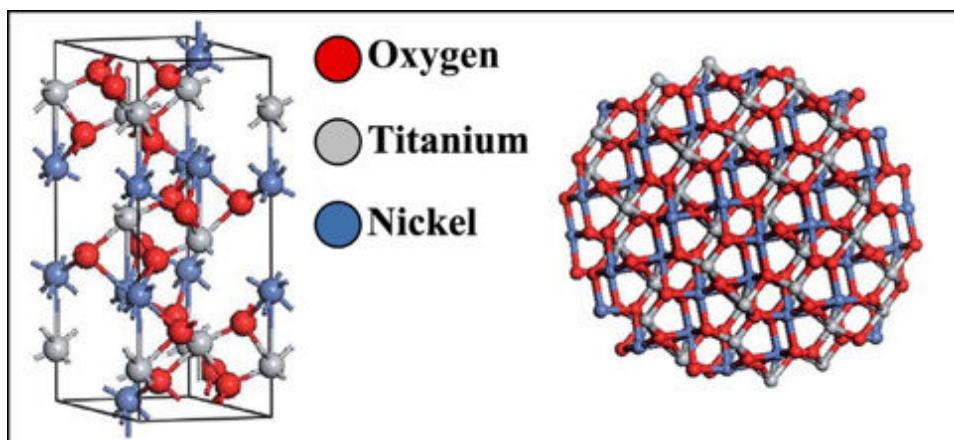
Fig. 2.1 The unit cell of crystalline \text{NiTiO}_3 (left) and the unpassivated nanocrystalline structure made by the formula (\text{NiTiO}_3)_{82} (right).
