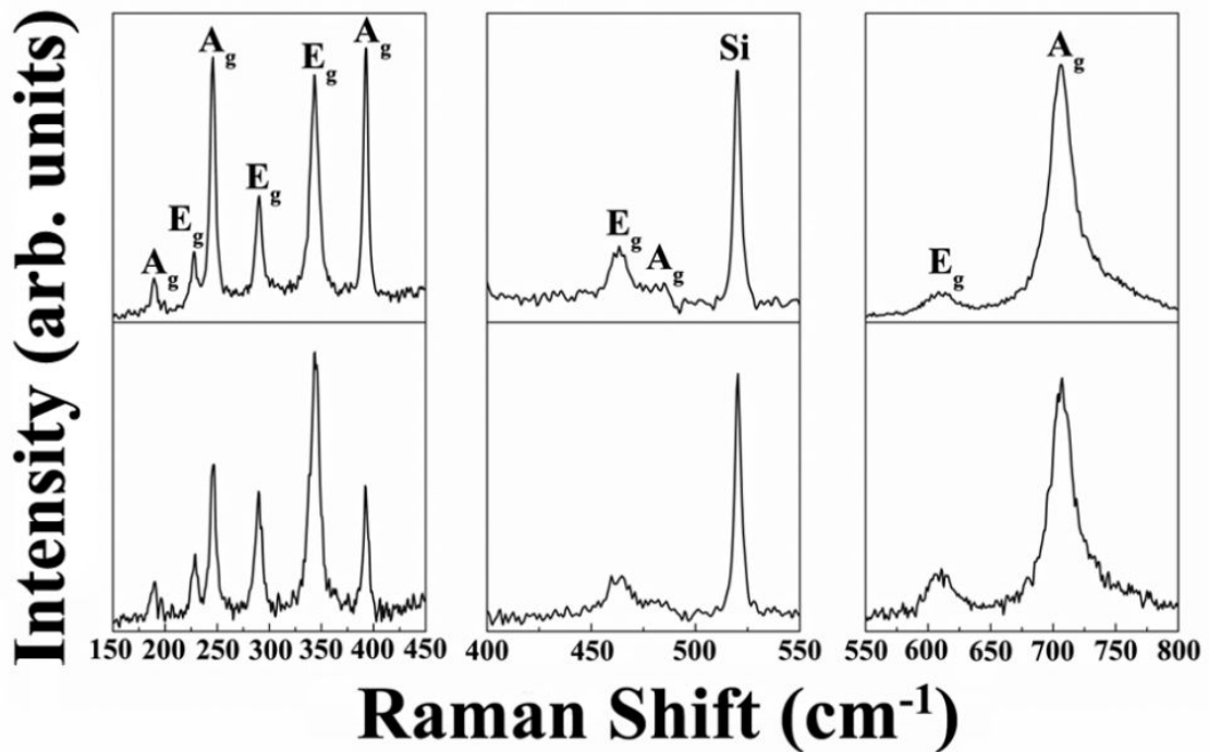
Fig. 8.7 Raman spectra collected from a representative \text{NiTiO}_3 thin film annealed at 1000\text{ }^\circ\text{C} for 2 hours in air atmosphere using: parallel polarization (top) and cross polarization (bottom).
