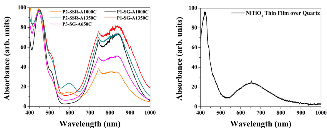
Fig. 8.1 UV-Vis absorption spectra obtained experimentally for the different \text{NiTiO}_3 powders (left) and the \text{NiTiO}_3 Thin Film deposited on quartz (right).
