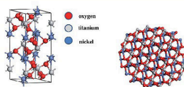
Fig. 1 The unit cell of crystalline NiTiO 3 (left) and the unpassivated nanocrystalline structure made by the formula (NiTiO 3 ) 82 (right).
