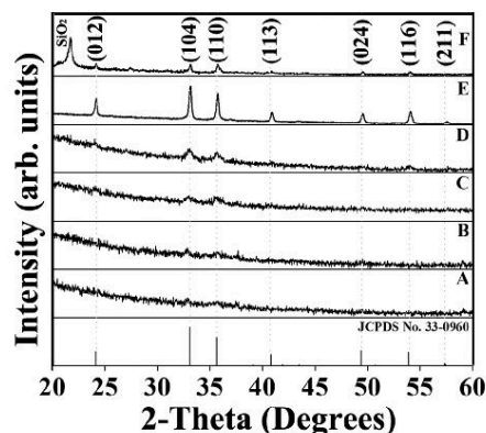
Fig. 1 XRD patterns of NiTiO 3 thin films annealed at different temperatures and durations under air. A) Annealed at 800 °C for 2 hours. B) Annealed at 800 °C for 4 hours. C) Annealed at 900 °C for 2 hours. D) Annealed at 900 °C for 6 hours. E) Annealed at 1000 °C for 2 hours. F) Annealed at 1100 °C for 2 hours.
