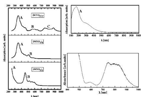
Fig. 7 UV-Vis absorption spectra calculated by the PM6 model for different clusters (left-hand panel), the spectrum calculated for the bulk crystal by using the DFT/PBE + U functional (upper right-hand panel) and the experimentally obtained data (lower right-hand panel).
