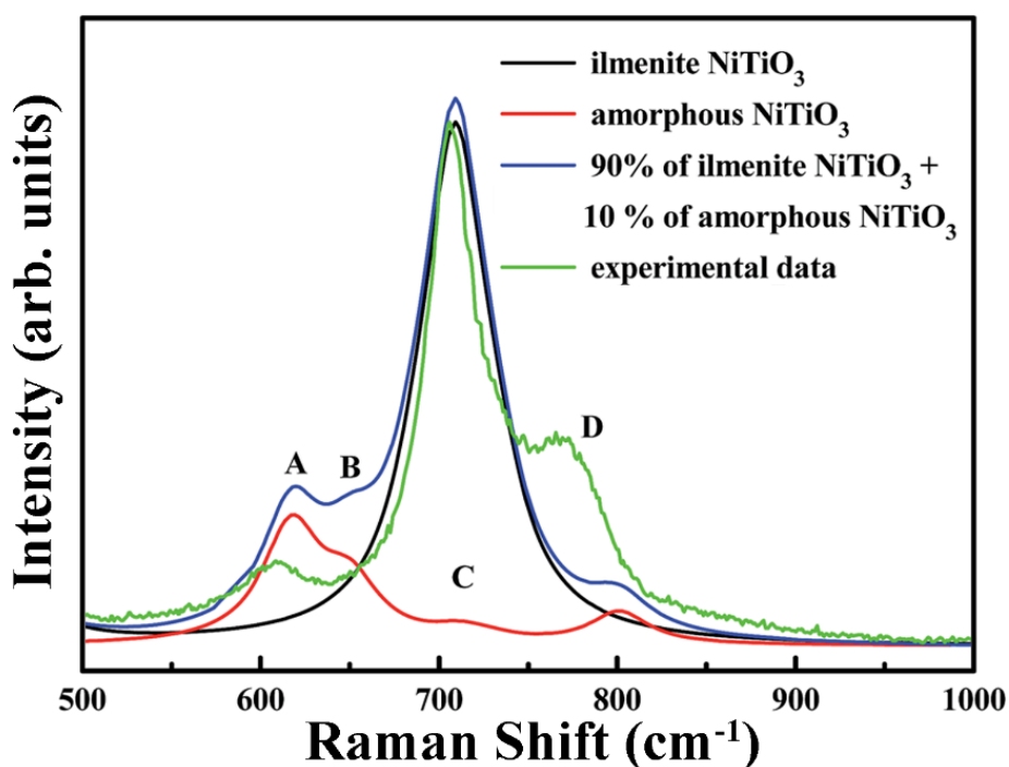
Fig. 8.8 Raman spectra for the (\text{NiTiO}_3)_{17} nanoparticles calculated by the parametrized PM6 method as well as experimental spectrum.
