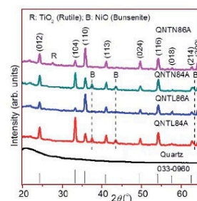
Fig. 2 XRD patterns of NiTiO 3 thin films deposited at different Ti power (200 W (QNTL84A) and 250 W (QNTL86A)) with nitrogen doping (QNTN84A and QNTN86A).
