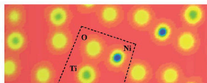
Fig. 3 Electron density projection in a selected plane of the \text{NiTiO}_3 ilmenite structure.
