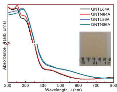
Fig. 9 Absorption spectra of \text{NiTiO}_3 thin films deposited at different Ti power (200 W (QNTL84A) and 250 W (QNTL86A)) with nitrogen doping (QNTN84A and QNTN86A). An inset shows post-annealed film deposited at 200 W Ti power without nitrogen doping.
