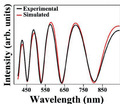
Fig. 7 Representation of the optical interferometry pattern made by a NiTiO 3 thin film annealed at 1000 °C for 2 hours in air atmosphere. The values of the fit are summarized in Table 1.
