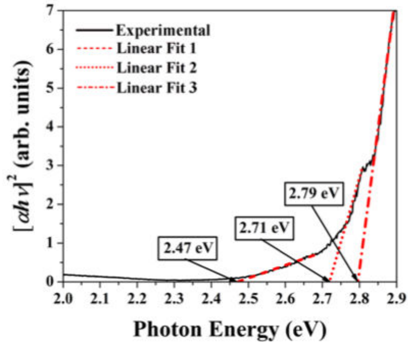
Fig. 6.9 Tauc plot of a \text{NiTiO}_3 thin film deposited on a quartz substrate; the film was annealed at 1000^\circ\text{C} under air and exhibits the ilmenite structure.
