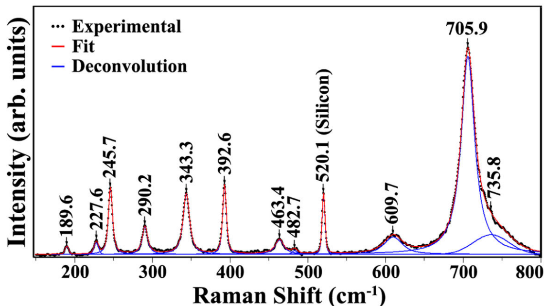
Fig. 6.5 Experimental and simulation of the Raman spectrum of the representative \text{NiTiO}_3 thin film annealed at 1000 °C for 2 hours in air atmosphere.
