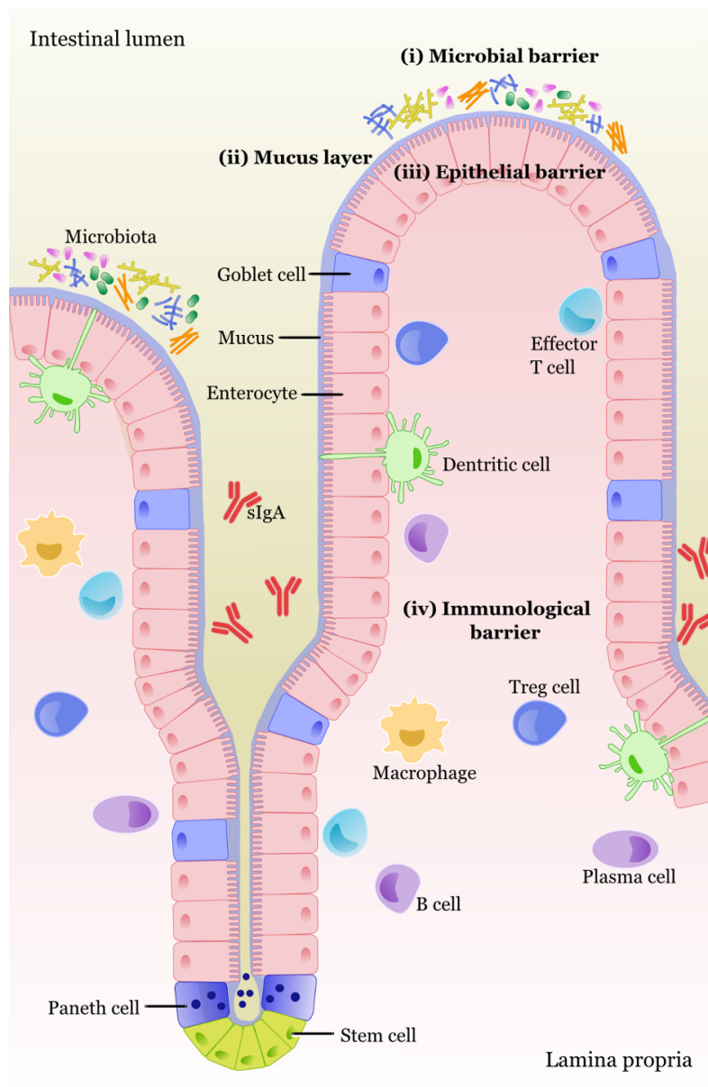
Fig. 1. The intestinal barrier. SIgA, secretory immunoglobulin A; Treg cell, regulatory T cell.
