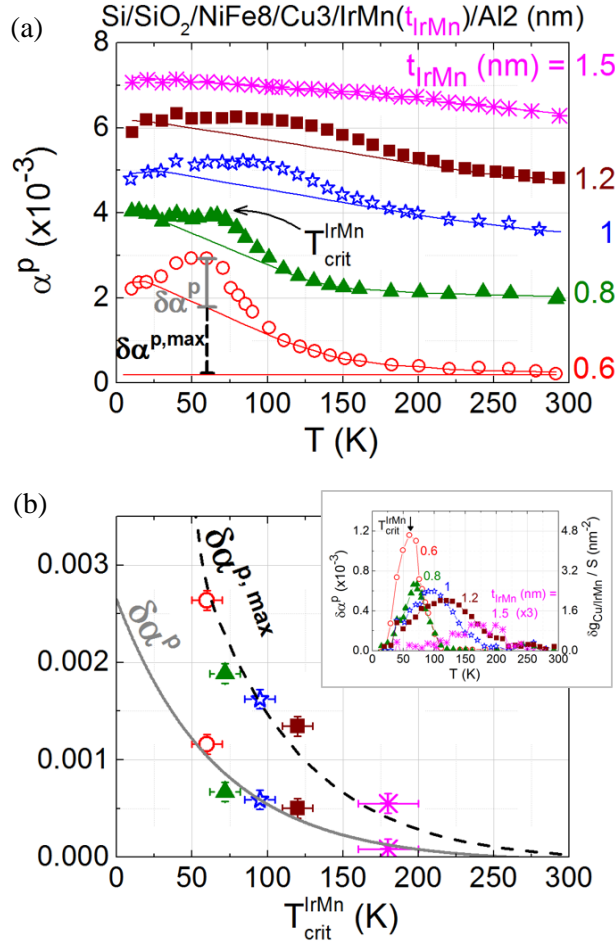
Figure 27 : (a) Dependence of additional extra non-local damping ( \alpha^p ) on temperature. To facilitate reading, the data were shifted vertically. Note: \alpha^p (295 K) \sim (0.2, 1.4, 0.75, 1.25 and 1.25) \times 10^{-3} for t_{IrMn} = 0.6, 0.8, 1, 1.2, and 1.5 nm, which translates to g_{eff}^{\uparrow\downarrow} / S (295 K) \sim 0.8, 5.6, 3, 5, and 5 nm -2 , respectively. The baselines are visual guides. From Ref. [1]. (b) Dependence of \delta\alpha^{p,max} on temperature for T=T_{crit}^{IrMn} . An exponential function was fitted to the data as a visual guide. Inset: Temperature dependence of \delta\alpha^p . Adapted from Ref. [1].
