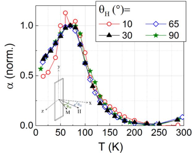
Figure 32 : \alpha Gilbert damping vs temperature, for different applied magnetic field direction, \theta_H ; 10, 30, 65 and 90° for \text{Si}/\text{SiO}_2/\text{NiFe8}/\text{Cu3}/\text{IrMn0.6}/\text{Al2} nm stack. For \theta_H = 90, 65, 30 and 10^\circ we get \alpha(300\text{K}) and \alpha(70\text{K}) = (8.5 \times 10^{-3}, 9.7 \times 10^{-3}, 17.7 \times 10^{-3}, 32.6 \times 10^{-3}) and (10.8 \times 10^{-3}, 12.1 \times 10^{-3}, 22.2 \times 10^{-3}, 42.6 \times 10^{-3}) , respectively.
