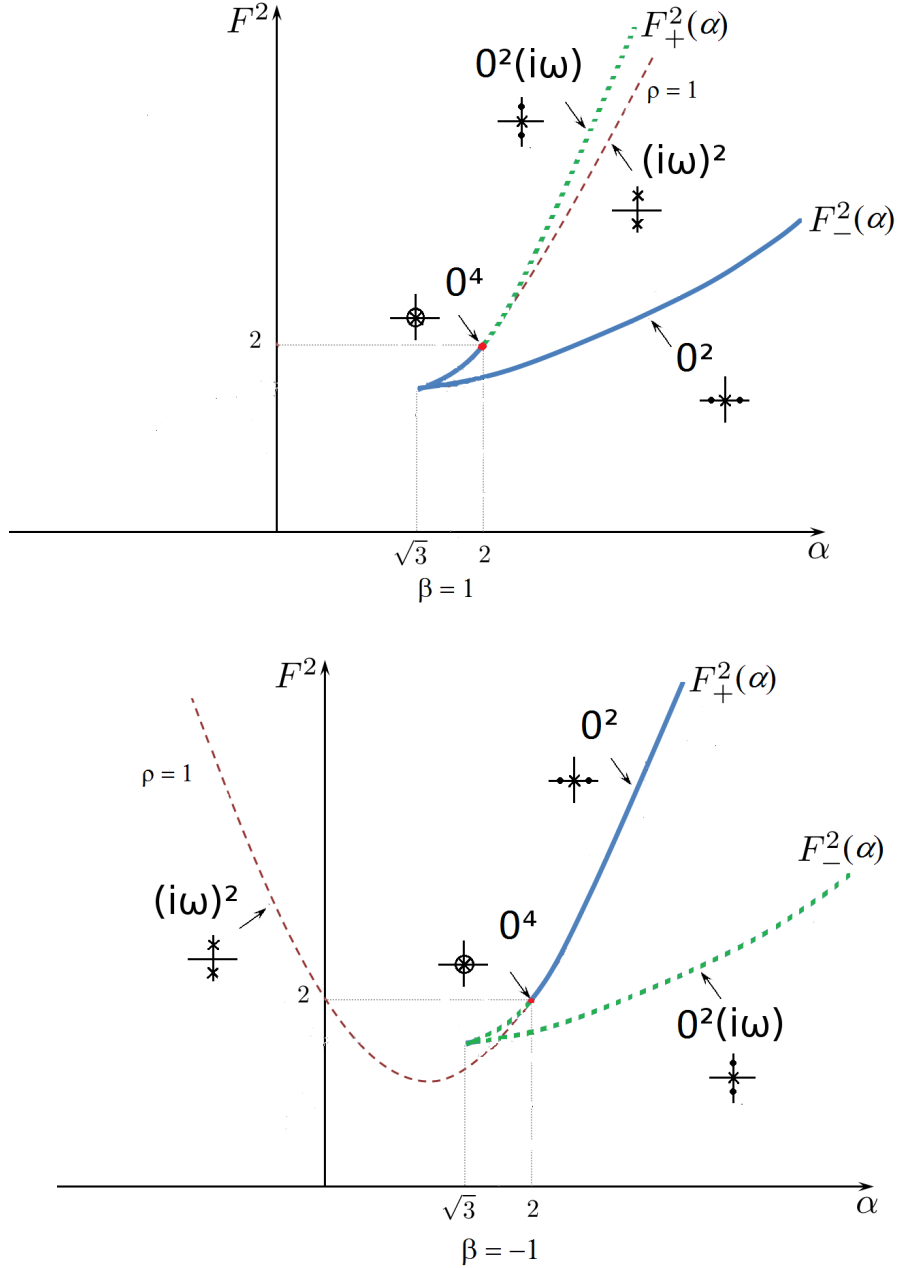
FIGURE 1.5 – Bifurcation diagrams for the case of normal (up) and anomalous (down) dispersion. (i\omega)^2 bifurcations occur along the dashed lines (of equation \rho = 1 ); 0^2(i\omega) and 0^2 bifurcations occur along the dotted lines, and the continuous lines, respectively (of equations F^2 = F_{\pm}^2(\alpha) ). In both cases a 0^4 bifurcation occurs at the point (\alpha^*, F^{*2}) = (2, 2) .
