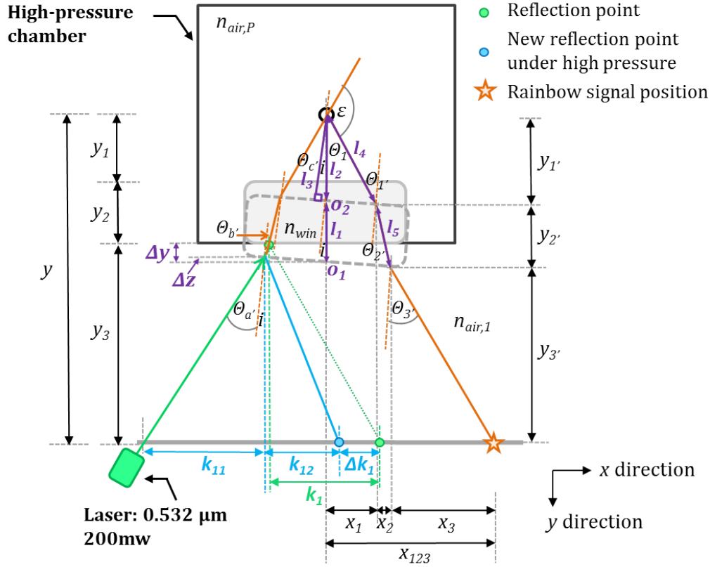
Figure 3.16: Orientation of the move of the optical window and the light path from the laser source through the screen for the third case (top view)
