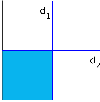
Figure 4.5: Figure of the cone \mathcal{P}_M in Example 4.1.2
