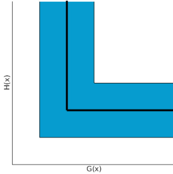
Figure 5.5: L-shape relaxation
