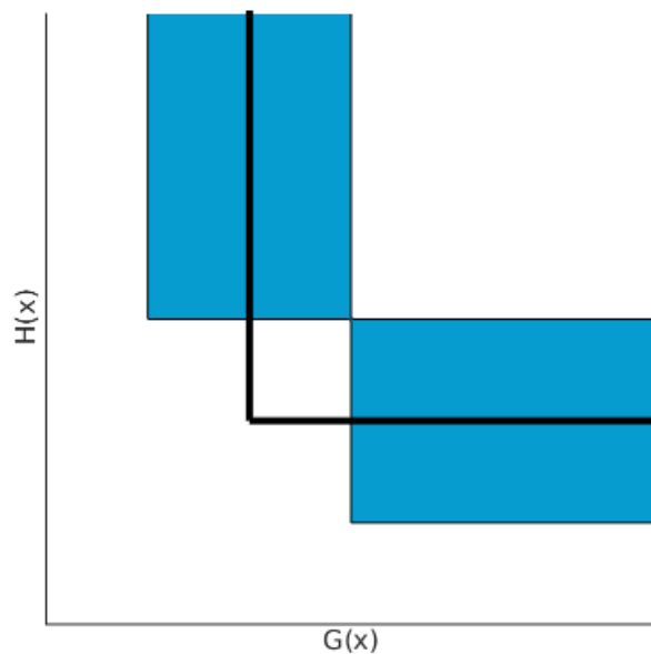
Figure 5.4: Boxes relaxation
