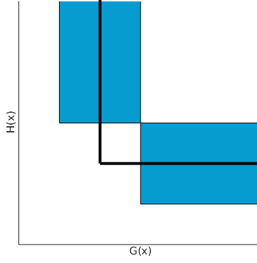
Figure 7.1: Feasible set of the approximation (KDB).
