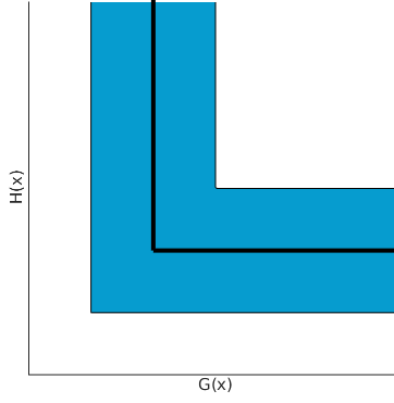
Figure 7.2: Feasible set of the relaxation (KS).
