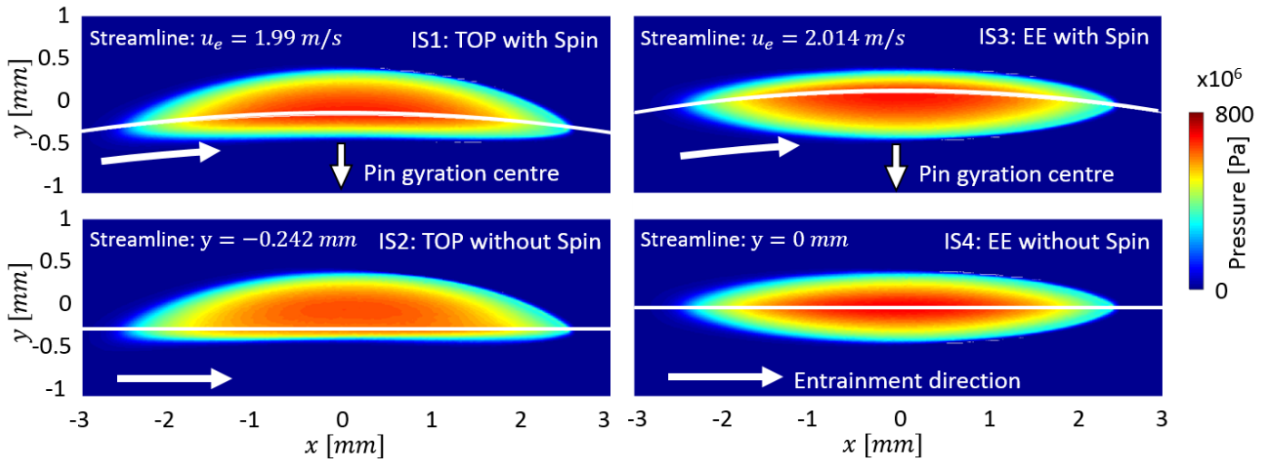
Figure 4.1-6 - The four investigative simulations: pressure fields and their inlet streamlines, friction reference case with \lambda = -1^\circ and SRR_-(x,0) = 0\%
