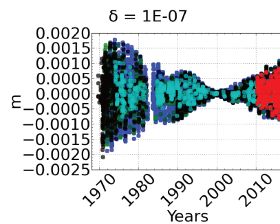
C_{4,0}, Earth
