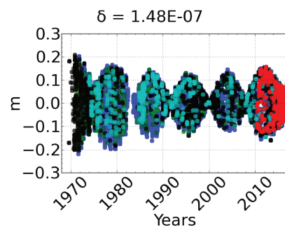
C_{3,0}, Earth
