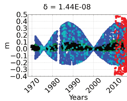
C_{3,1}, Moon
