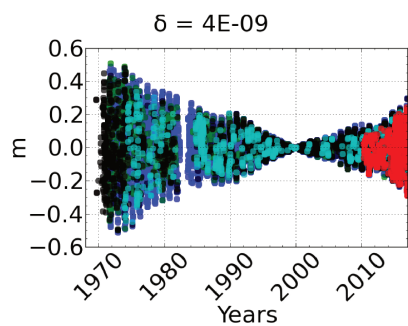
C_{2,0}, Earth
