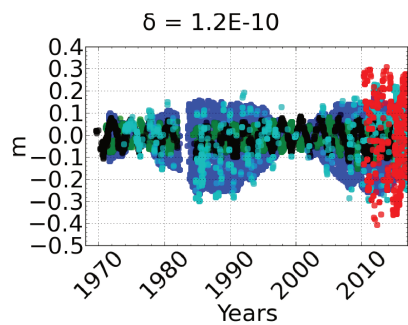
C_{2,2}, Moon
