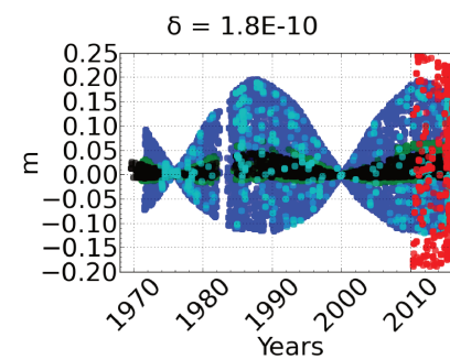
C_{2,0}, Moon
