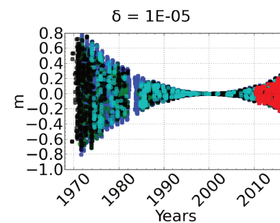
\tau_{R2}, Earth
