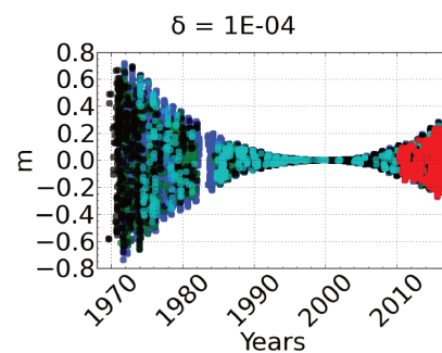
\tau_{R1}, Earth
