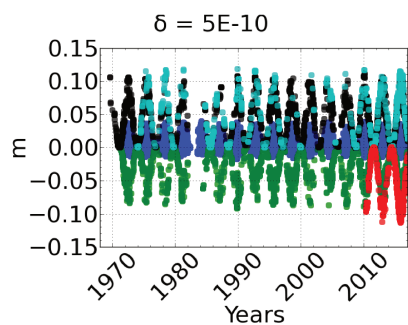
S_{4,4}, Moon
