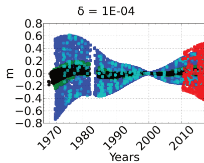
\omega_{c,y}, Moon(t=0)
