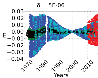
\omega_{c,x}, Moon(t=0)
