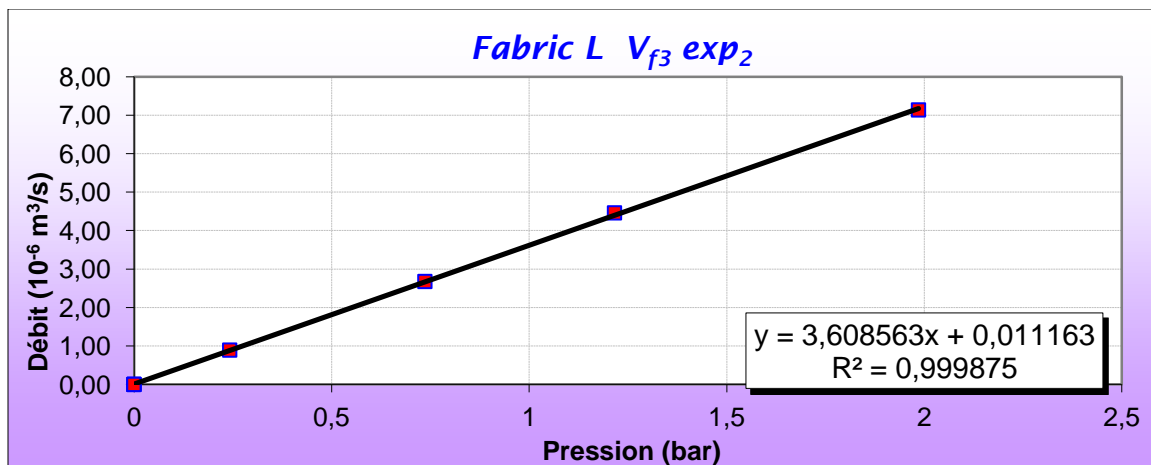
Appendix 2 Figure 31 Through-thickness permeability experiment Fabric L ( V_{f3} exp 1 ).
