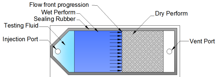
Figure 25 Principle of unidirectional in-plane permeability measurements.
