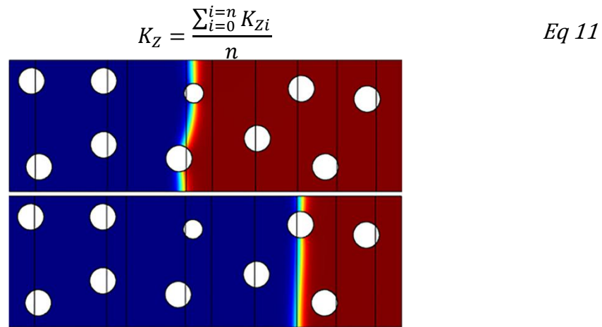
Figure 18 Flow front observed at two different positions for 0.89 porosity unit cell.
