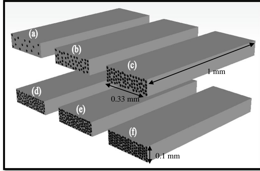
Figure 13 Selected porosities for transversal flow simulation (a): 0.9, (b): 0.7, (c):0.5, (d): 0.44, (e): 0.3, and (f):0.23
