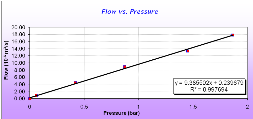
Figure 36 (for V_F = 49.67\% ). R^2 shows the degree of correlation between successive applied flow and corresponding pressures, a higher R^2 value means a more reliable experiment.
