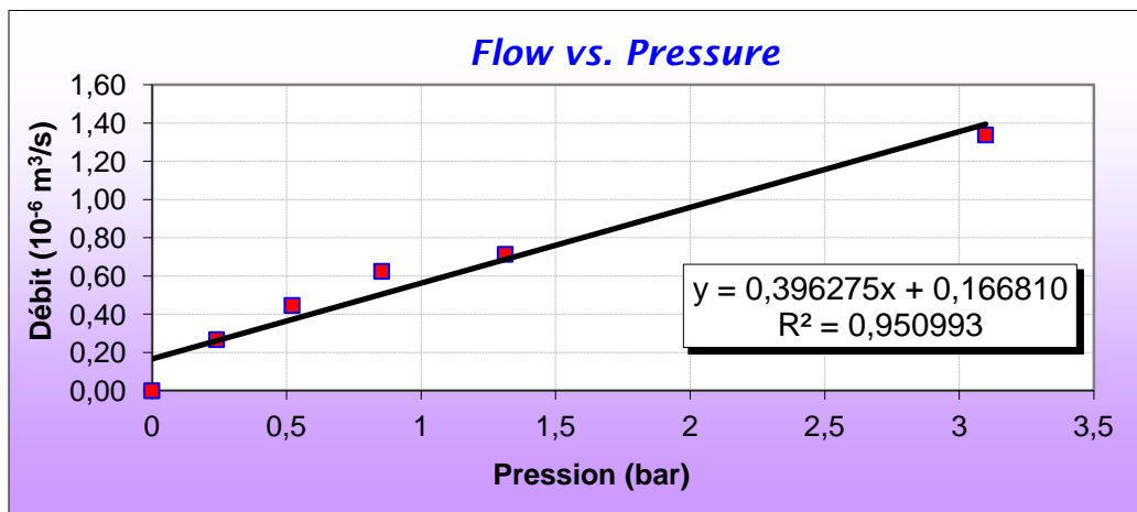
Figure 41 Fabric H through-thickness permeability measurement ( V_{fl} , exp_1 )
