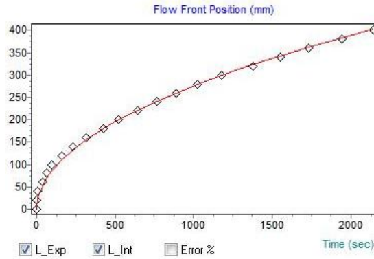
Figure 28 Flow front position as a function of time in a test at 0^\circ .
