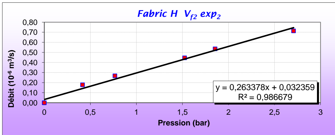
Appendix 2 Figure 11 Through-thickness permeability experiment Fabric H ( V_{f2} \text{ exp}_2 ).
