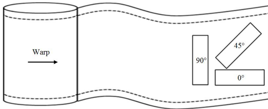
Figure 20 Fiber orientation in the roll
