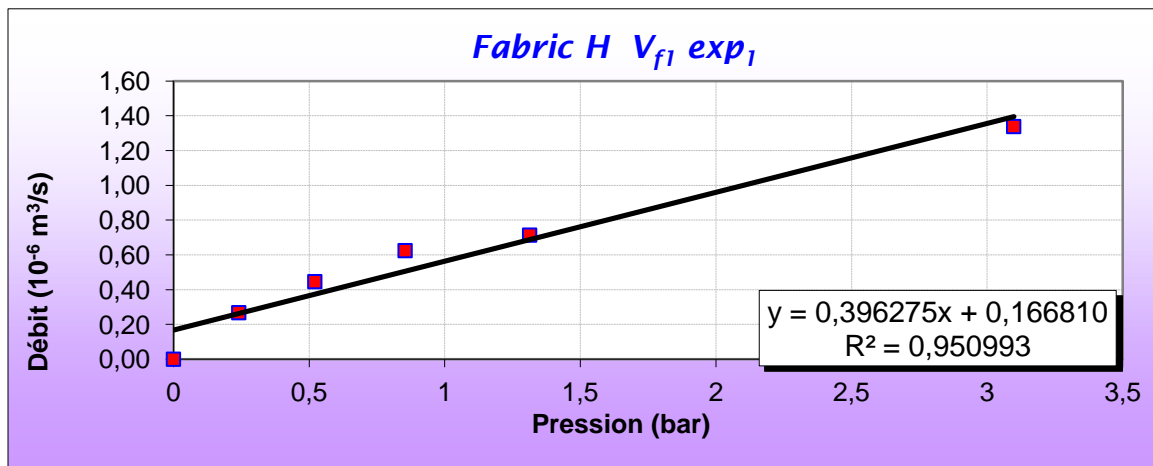
Appendix 2 Figure 8 Through-thickness permeability experiment Fabric H ( V_{f1} exp 1 ).
