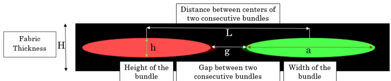
Figure 82 Textiles dimensions.
