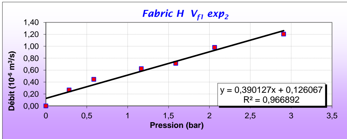
Appendix 2 Figure 9 Through-thickness permeability experiment Fabric H ( V_{f1} \text{ exp}_2 ).
