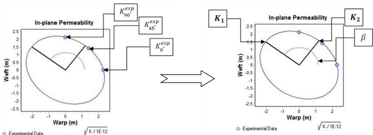
Figure 31 Permeability ellipse for a fabric at V_f= 50.7\% .
