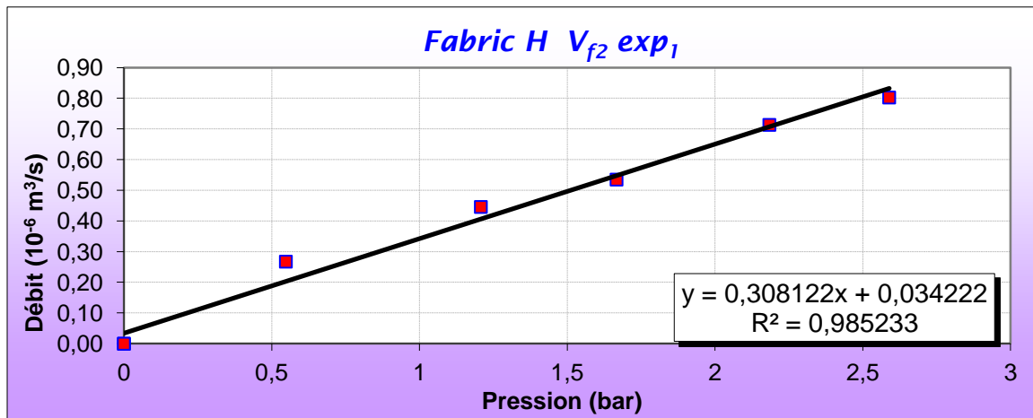
Appendix 2 Figure 10 Through-thickness permeability experiment Fabric H ( V_{f2} \text{ exp}_1 ).
