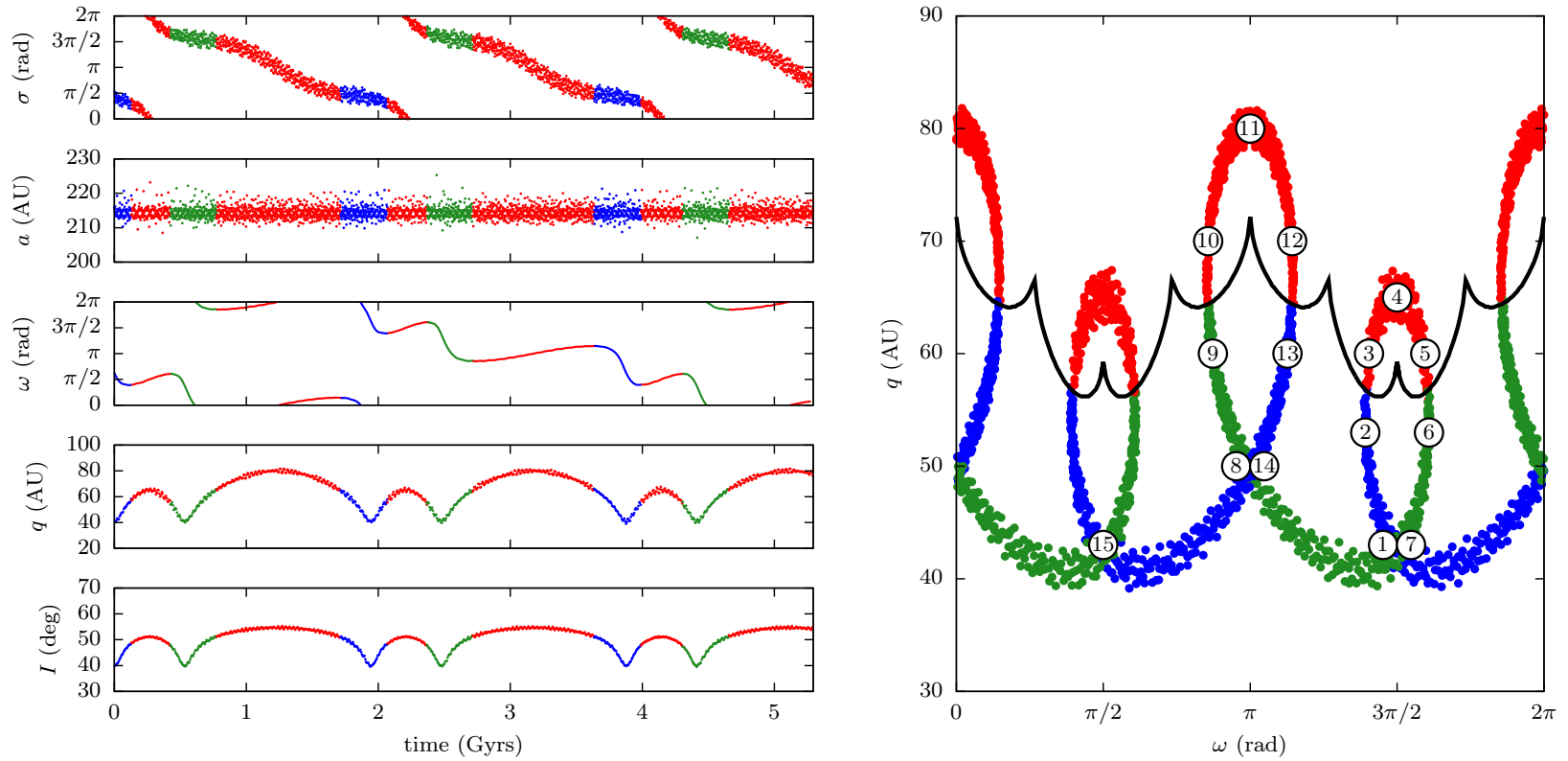
Figure 4.7 – Numerical integration of the unaveraged system for the resonance 1:19 with Neptune. On the right, the trajectory is projected in the plane (\omega, q) , where the secular discontinuity line is added in black. Visible on the left panel, the oscillations of the semi-major axis are essentially due to the motion of the Sun around the barycentre of the Solar System: in the averaged system, the secular shift of the resonance centre ranges only from 214.775 AU to 214.777 AU. The colour code is chosen according to the geometry of the semi-secular phase space: when it contains two resonance islands, the trajectory is plotted in green (right island) or blue (left island). In the red portions, there is only one resonance island. The numbers refer to Fig. 4.8, where the geometry of the semi-secular phase space is shown.
