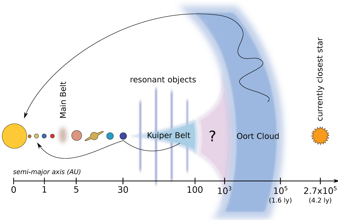
Figure 1.2 – Current dynamical structure of the Solar System as it is considered today. The bodies sizes are not to scale. The horizontal axis represents the semi-major axes of the orbits, and the vertical placement gives an idea of the inclinations. The arrows symbolise the creation of long-period comets, Centaurs and Halley-type comets. The latter two are produced from trans-Neptunian and Oort Cloud objects through close encounters with the planets.
