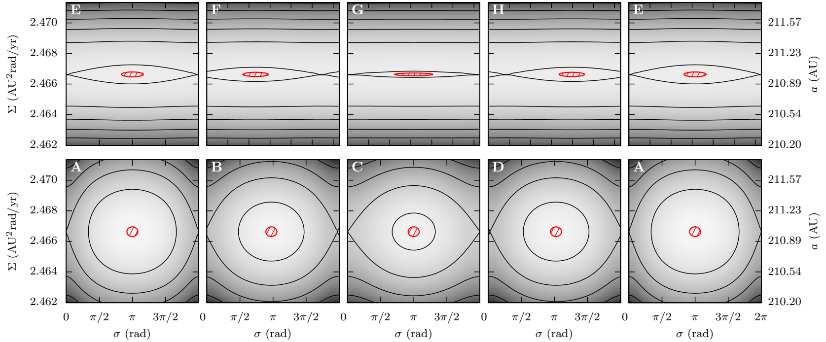
Figure 3.13 – Level curves of the semi-secular Hamiltonian \mathcal{K} , for (U, u) fixed according to the points A-H of Fig. 3.11. The trajectory enclosing the surface 2\pi J is shown in red and the semi-major axis corresponding to \Sigma is given on the right. The centre is perfectly at \sigma = \pi for the points (A, C, E, G) but slightly shifted for (B, F) and (D, H) symmetrically on the left and on the right. For the points E-H, the \Sigma -width of the resonance island is very narrow because of the high perihelion distance (see Fig. 3.11), which makes the red surface to flatten.
