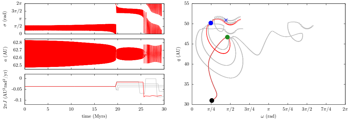
Figure 4.14 – Numerical integration of the two-degree-of-freedom semi-secular system. The initial conditions (origin of the time and black spot on the right) are taken according to the level curves plotted in Fig. 4.13c. On the right, the evolution of the couple (U, u) is drawn (with q instead of U , obtained by inverting Eq. 3.56). Several initial phases for (\sigma, \Sigma) were tried, leading to secular trajectories diverging at the first separatrix crossing (grey curves). Among them, the red trajectory is in agreement with our backward reconstruction: its second transition occurs on the blue spot, and it passes near the current position of 2015 FJ 345 (to be compared with the level curves from Fig. 4.13). On the left, the evolution of the couple (\sigma, \Sigma) is represented for the red trajectory (with a instead of \Sigma ). The two separatrix crossings, leading to a change of oscillation island, are easily noticeable. The bottom graph presents the evolution of the area 2\pi J for all the trajectories plotted on the right, showing the divergence at the first transition. Even if 2\pi J is plotted as a continuous line, please remember that its definition changes after each transition (different resonance island).
