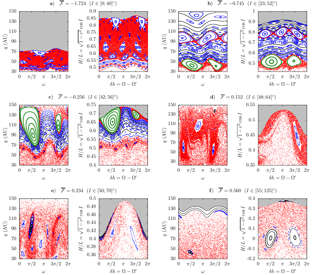
Figure 5.15 – Poincaré maps for an inclined perturber. The constant semi-major axis of the particle is a = 150 AU. Every section in the (\omega, q) plane is made for \delta h = \pi/2 and \delta \dot{h} < 0 . Every section in the (\delta h, H) plane is made for \omega = \pi/2 , with \dot{\omega} > 0 for (a,b,c,d,e) and \dot{\omega} < 0 for f.
