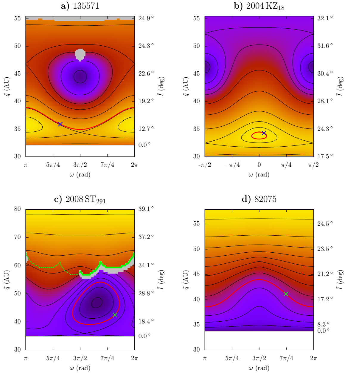
Figure 4.12 – Phase portraits of the objects affected by secular libration islands. On the graph a , the object 135571 is the only one found to have a retrograde circulation of \omega . On the graph b , the secular evolution of 2004 KZ 18 inside the mean-motion resonance makes \omega oscillate around 0. On the graph c , there are two distinct regions according to the topology of the semi-secular phase-space, since the resonance of 2008 ST 291 is of type 1:k . Below the green line, the resonance island is doubled (as in Fig. 4.10c,d) resulting in asymmetric level curves. Above the green line, only one resonance island remains (as in Fig. 4.10a,b) and the level curves are symmetric. If the line is crossed, there can be either a discontinuity (thick green line) if the particle is located in the vanishing island, or a smooth transition (dotted green line) if it is located in the persisting island.
