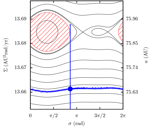
Figure 4.15 – Semi-secular phase portrait of 2014 FZ 71 . On the right axis, the values of a corresponding to \Sigma are shown. The blue crosses come from the filtered output of the full non-averaged numerical integration (same as Fig. 4.10), with the current position of 2014 FZ 71 on the big spot. For comparison, the 1-sigma error bar of the (osculating) orbital solution is added. The uncertainty is compatible with the red hatched area inside the resonance, from which we get a possible value of the parameter J .
