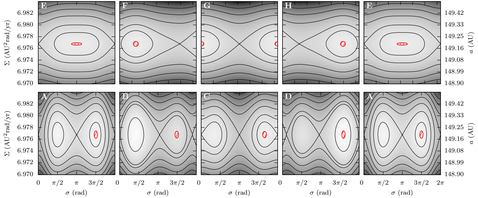
Figure 3.21 – Level curves of the semi-secular Hamiltonian \mathcal{K} , for (U, u) fixed according to the points A-H of Fig. 3.20. The trajectory enclosing the surface 2\pi J is shown in red, and the semi-major axis corresponding to \Sigma is given on the right. Only one resonance island is left for the points E-H because they correspond to a high perihelion distance (see Fig. 3.20).
