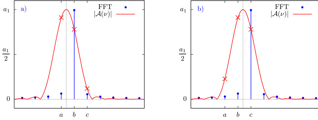
Figure C.11 – Bracketing of the maximum of the amplitude function \mathcal{A}(\nu) starting from a FFT: a) bad bracketing because g(b) < g(a) ; b) suitable bracketing.
