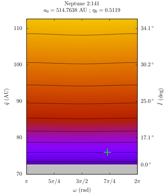
Figure 4.18 – Level curves of the secular Hamiltonian for the resonance 2 : 141 with Neptune, which is located near the semi-major axis of Sedna. The value chosen for a_0 is indicated above the figure as well as the parameter \eta_0 corresponding to the elements of Sedna. This graph is plotted for J = 0 and the green cross shows the current position of Sedna in the plane (\omega, q) .
