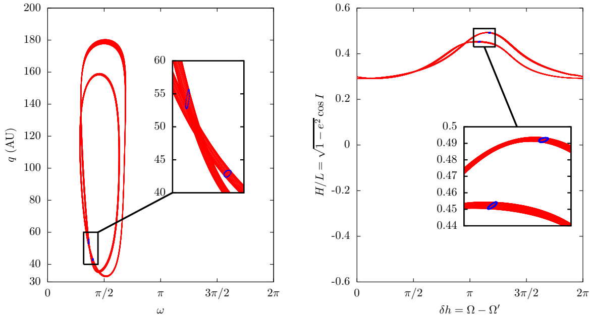
Figure 5.16 – Complete trajectory producing the tiny blue points in the panel e of Fig. 5.17 ( a = 200 AU). This is a quasi-periodic orbit featuring the secondary resonance 2:1 between \delta\dot{h} and the libration frequency of the resonant angle 1:1 between \delta\dot{h} and the libration frequency of \omega . On each graph, blue points are added when the trajectory crosses the sections (same as Fig. 5.17). Enlarged views show the classic rounded shapes formed by the section crossing points around the periodic trajectory. According to the resonance involved, the fixed points are 2 on both sides.
