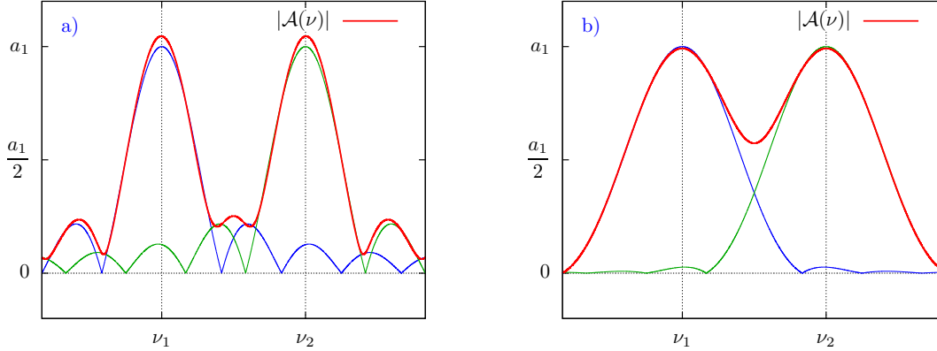
Figure A.2 – Norm of the amplitude function in the case of two sinusoidal terms: a) without the Hanning window; b) with the Hanning window. The curves obtained for the two terms taken separately are drawn in blue and green.
