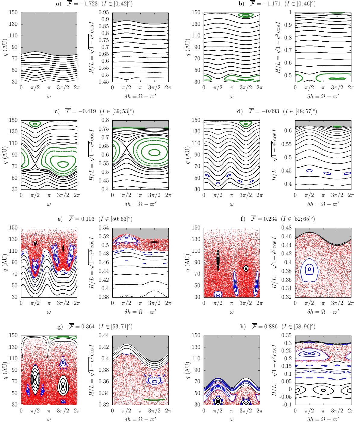
Figure 5.6 – Poincaré maps for a planar perturber. The constant semi-major axis of the particle is a = 150 AU. Every section in the (\omega, q) plane is made for \delta h = \pi/2 and \delta h < 0 . Every section in the (\delta h, H) plane is made for \omega = \pi/2 , with \dot{\omega} > 0 for (a–g) and \dot{\omega} < 0 for h. In the panel e, the libration island of \omega around \pi/2 appears only as a 1:1 resonance between the libration frequency of \omega and the circulation frequency of \delta h (small black island at \delta h = 3\pi/2 ). We used black lines, though, to stress that \omega itself oscillates around \pi/2 , but please note that \delta h actually circulates, despite the closed black curves drawn on the right.
