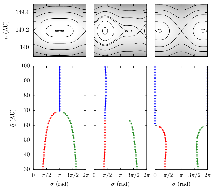
Figure 3.23 – Position of the two resonance centres with respect to the perihelion distance (same resonance and parameters as Fig. 3.20). The left centre is plotted in red, the right one in green, and blue is used when only one resonance centre remains. The fixed value of \omega is equal to 0 (left column), \pi/4 (middle column) and \pi/2 (right column). On the top, the overall phase portrait is shown for a value of \tilde{q} just below the transition ( \tilde{q} = 69 AU on the left, 63 AU on the middle and 59 on the right). For \omega between 0 and \pi/2 (middle column), the left resonance island is not affected by the vanishing right island: it becomes smoothly the single remaining resonance island. The roles are exchanged for \omega between \pi/2 and \pi (not shown).
