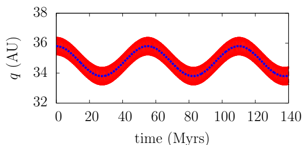
Figure 2.2 – Typical evolution of a dynamical quantity (here the perihelion distance) in a quasi-integrable perturbed two-body problem. The red curve represents the osculating trajectory obtained by numerical integration. Its “thickness” is made of fast small-amplitude oscillations. The blue curve is the corresponding secular trajectory.
