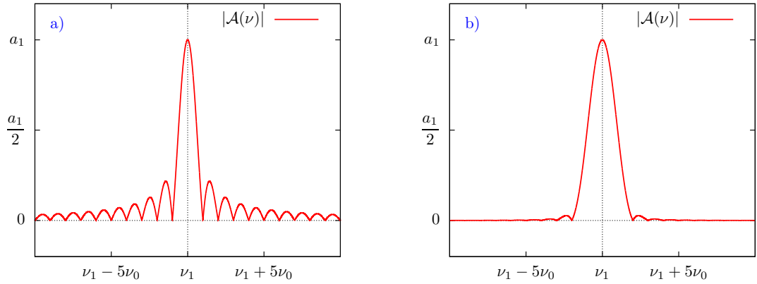
Figure A.1 – Norm of the amplitude function in the case of only one sinusoidal term: a) without the Hanning window; b) with the Hanning window.
