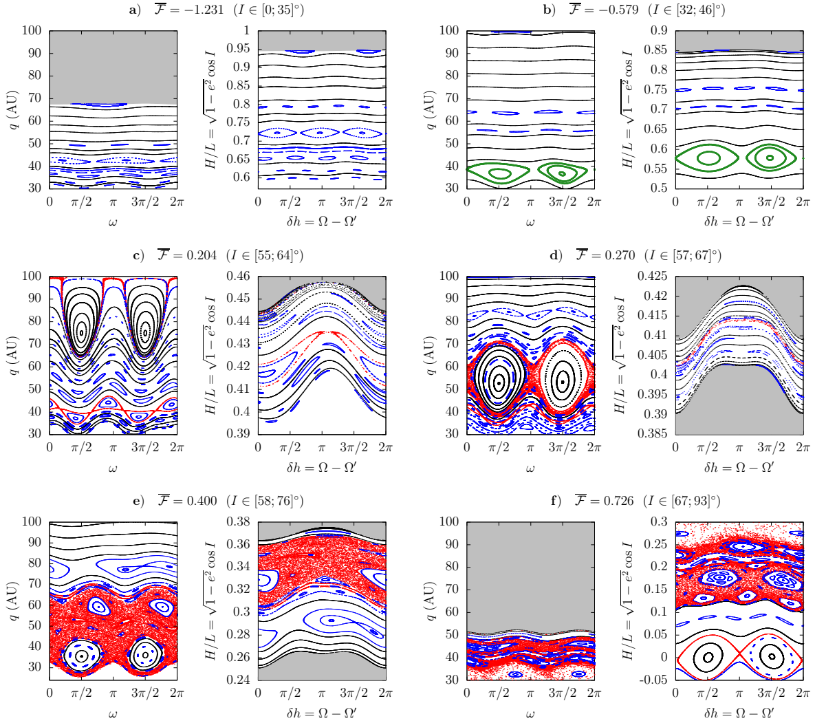
Figure 5.13 – Poincaré maps for an inclined perturber. The constant semi-major axis of the particle is a = 100 AU. Every section in the (\omega, q) plane is made for \delta h = \pi/2 and \dot{\delta h} < 0 . Every section in the (\delta h, H) plane is made for \omega = \pi/2 , with \dot{\omega} > 0 for (a,b,c) and \dot{\omega} < 0 for (d,e,f). The panels (c,d,e) show the shift of the fixed points for \omega at I \approx 63^\circ for nearby Hamiltonian values. The surrounding chaotic sea is very wide when the islands are near the semi-major axis of Neptune (panel e). Resonances between \omega and \delta h are very numerous at all ranges of inclination. In the panels e and f, a zoom-in view reveals a very complex pattern of secondary resonances spreading in a fractal-like way.
