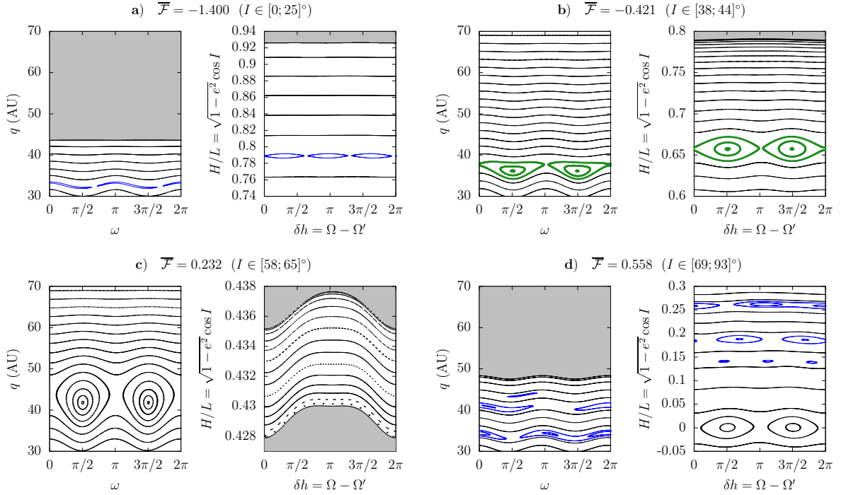
Figure 5.12 – Poincaré maps for an inclined perturber. The constant semi-major axis of the particle is a = 70 AU. Every section in the (\omega, q) plane is made for \delta h = \pi/2 and \delta h < 0 . Every section in the (\delta h, H) plane is made for \omega = \pi/2 , with \dot{\omega} > 0 for (a,b) and \dot{\omega} < 0 for (c,d). The panel a features the resonance 2\omega + 3\delta h . The panels b and d feature the resonances \omega + \delta h and \omega - \delta h , respectively, with two different fixed points and horseshoe-type orbits. In the panel d , the resonances \omega - 2\delta h and \omega - 3\delta h are also visible.
