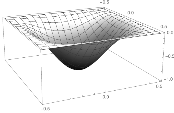
Figure 8.4 – In dimension 2, a typical choice for the pinning potential is e.g. \tilde{h}^0(x) := -\cos(\pi x_1)^2 \cos(\pi x_2)^2 for x \in Q = [-\frac{1}{2}, \frac{1}{2}]^2 .
