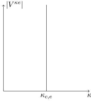
Figure 8.3 – In the Bean and Kim-Anderson models, the exact velocity law typically given by Figure 8.1 is replaced by this simplified law.
