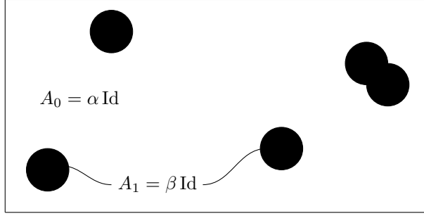
Figure 1.1 – Clausius-Mossotti model of dispersed spherical inclusions.
