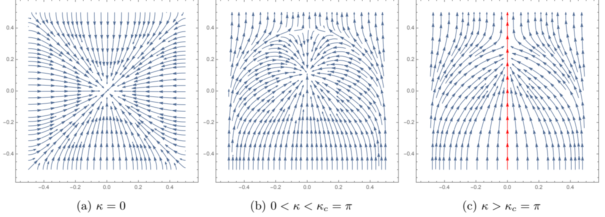
Figure 8.5 – In dimension d = 2 , for the typical example of pinning potential \tilde{h}^0 given in Figure 8.4, with \alpha = 1 , \beta = 0 , we plot the stream lines of the vector field -\Gamma^{(0,\kappa)} for growing values of \kappa . The assumptions of Proposition 8.9.11 are clearly seen to be satisfied: for \kappa < \kappa_c = \pi there is a unique stable fixed point, while for \kappa > \kappa_c = \pi the stable fixed point gives way to a periodic orbit with image \mathcal{O} = \{0\} \times [-1/2, 1/2] .
