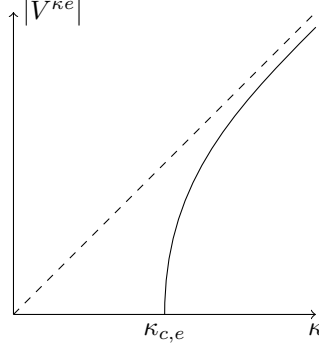
Figure 8.1 – Typical forcing-velocity characteristics exhibiting a stick-slip velocity law.
