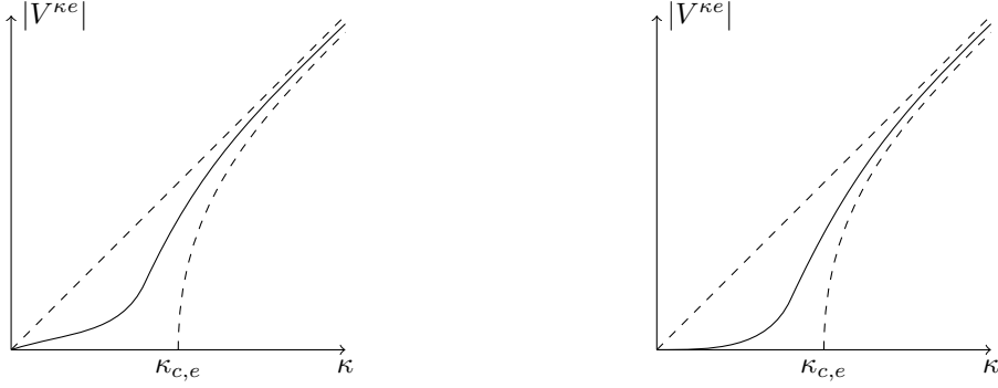
(a) Subcritical regimes: (linear) ohmic velocity law in the low-forcing limit.
