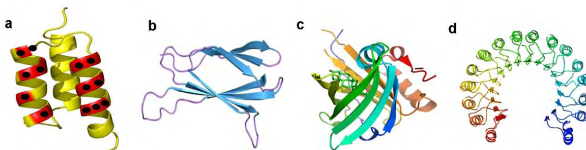
Fig IV.1: Different protein backbones used as scaffolds for the generation of protein-binding agents, a) three-helix bundle Affibodies b) The tenth fibronectin* type III domain classified as monobodies c) 3D structure model of an anticalins (ribbon) in complex with digitoxigenin and d) Leucine-rich repeat protein, a porcine ribonuclease inhibitor.
