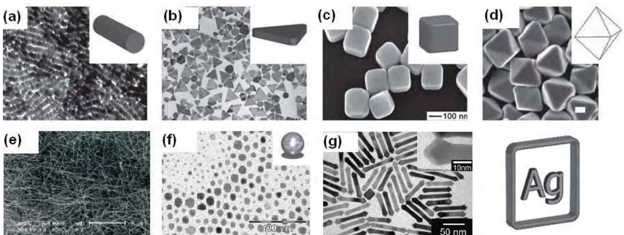
Fig I.4: Anisotropic nanostructures of Ag. (a) Nanorods (b) triangular (c) cubic (d) bi pyramidal (e) nanowires (f) spherical nanoparticles and (g) bimetallic rods with sharp tips 55,57 . Image is extracted from the reference Nanoscale , 2011, 3, 1304.
