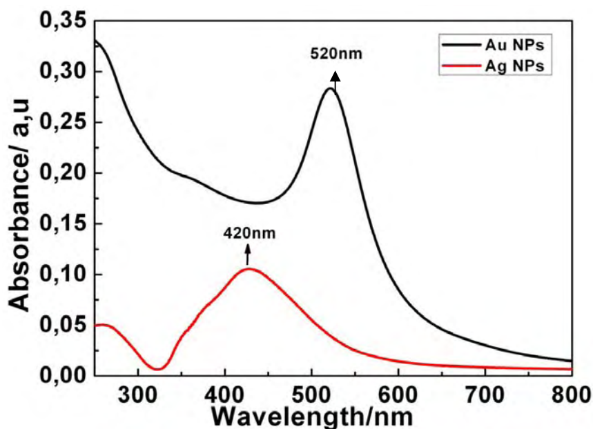
Fig II.2: UV-Vis absorption spectra of as synthesized Au and Ag nanoparticles.
