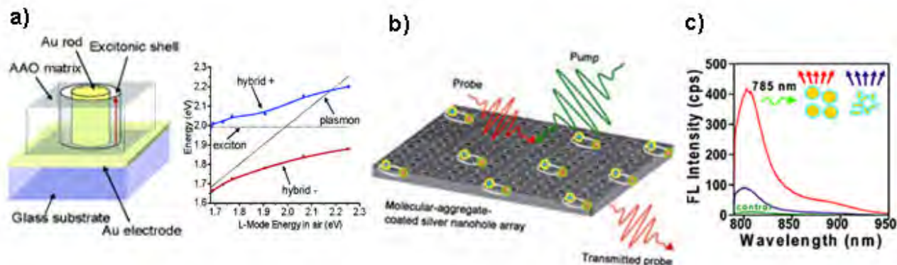
Fig 1.9: Schematic illustration and experimental data depicting different approaches employed to study metal enhanced fluorescence. a) Assembly of aligned Au nanorods supported by a transparent substrate and energy diagram showing the anti crossing of the plasmonic (diagonal solid black line) and the excitonic (horizontal dotted black line). 88 b) Diagram illustrating J-aggregated molecules onto a metallic nanostructure fabricated by perforating a 100 nm thick silver film with a hexagonal array of holes 230 nm in diameter. The dynamics of coupled exciton-SPP hybrid modes is studied in a transient absorption experiment. 92 c) Fluorescence spectra showing enhancement by Au nanoshells and nanorods on conjugation with conjugation of HSA_IR800 protein-fluorophore complex to nanoshells (NSs) and nanorods (NRs). 91
