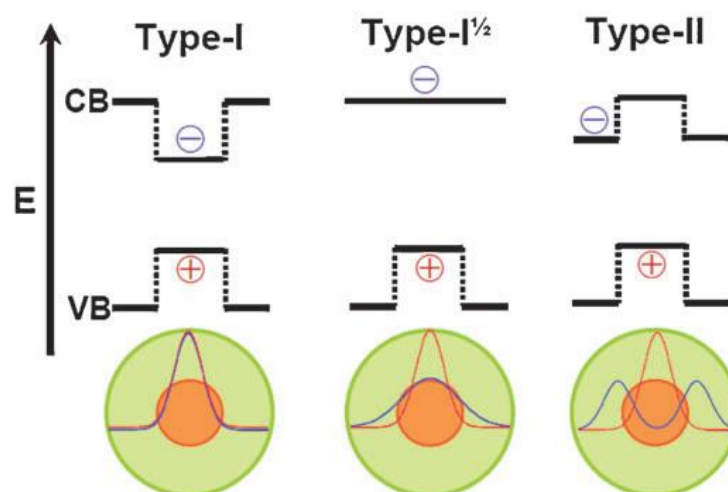
Figure 1.10 Schematic representation of the three-limiting charge carrier localization regimes in core-shell quantum dots. Adapted from reference [17]. Courtesy of M. Vis and A.G.M. Brinkman (Utrecht University, Netherlands).
