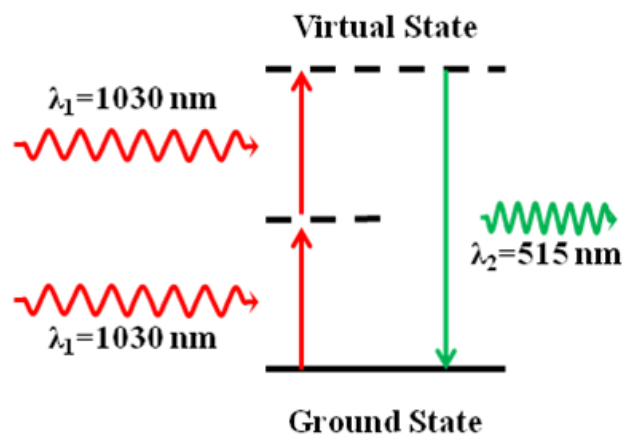
Figure 6.2 Second harmonic generation principle: depending of its non-linear optical properties a material can be excited by absorbing consecutively two photons of the same energy thus resulting in the emission of a photon whose energy is doubled.
