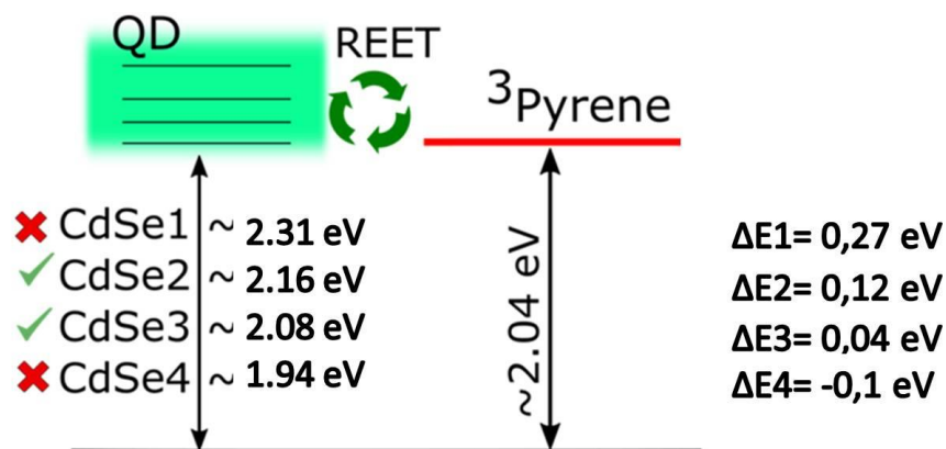
Figure 5.40 Schematic representation of the energy levels involved in the interaction with the lowest excited triplet state of 1-PCA.
