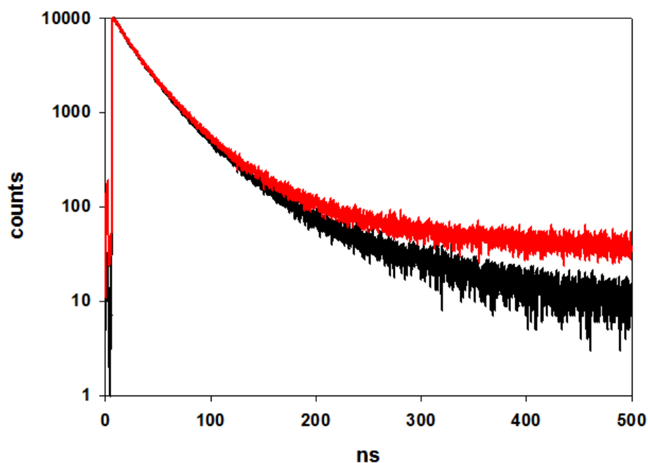
Figure 5.28 Comparison between the luminescence decay of CdSe3-1PCA in deaerated (red decay) and air-equilibrated (black decay) heptane.
