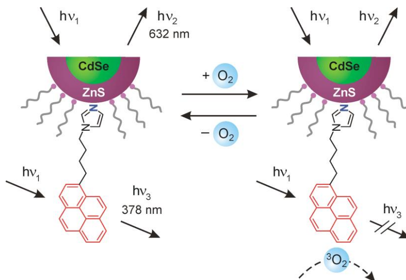
Figure 1.15 Schematic representation of the oxygen sensor consisting of CdSe-ZnS QDs decorated with an imidazole-based surfactant bearing a pyrenyl unit. Adapted from reference [92]. Copyright Springer 2016.
