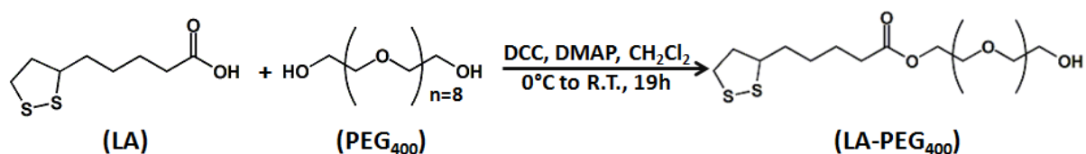
Scheme 2.5 Synthetic route for preparing PEG 400 -tagged lipoic acid.
