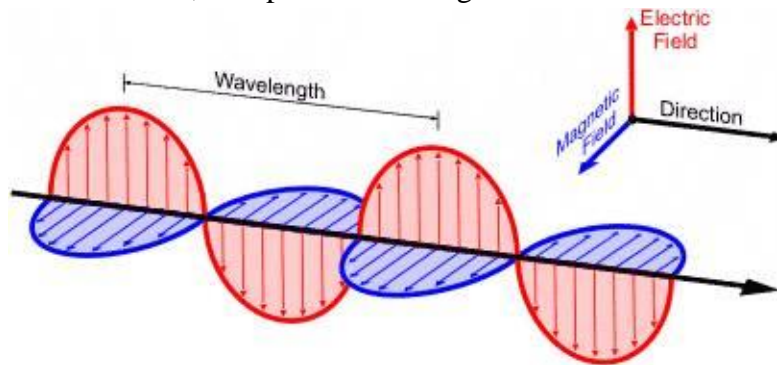
Figure 4.1 Representation of light as an electromagnetic radiation.
