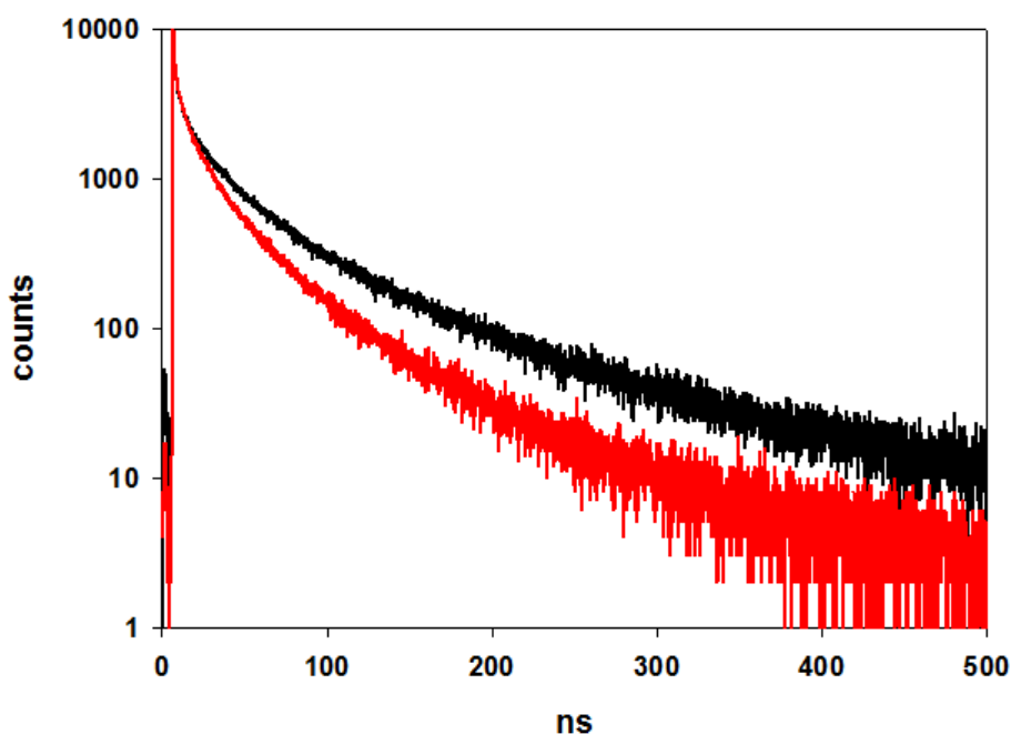
Figure 5.36 Luminescence lifetimes of CdSe 1 -1PCA (red decay) and CdSe 1 (black decay). The decays are recorded in deaerated heptane by exciting selectively QDs at 405 nm. The time scale is 500 ns while the 10000 counts detected at 540 nm are reported in logarithmic scale.
