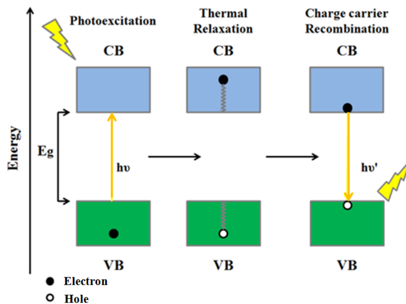
Figure 1.5 Schematic representation of the photoluminescence process in bulk materials.
