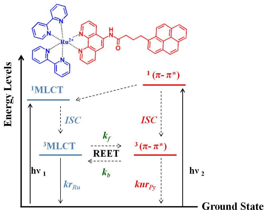
Figure 5.7 Schematic representation of REET occurring after selectively exciting the polypyridyl ruthenium (II) complex or the pyrenyl moiety.
