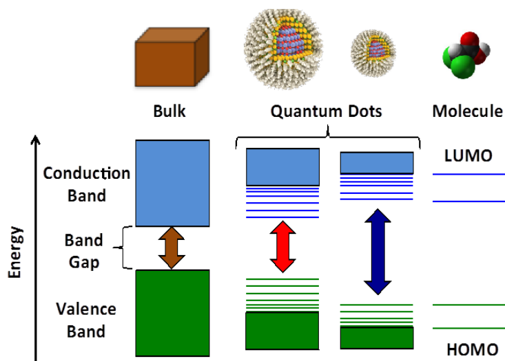
Figure 1.4 Comparison between bulk materials, QDs and general molecules in terms of electronic energy.
