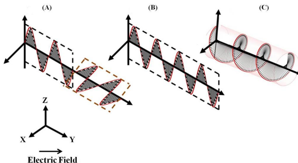
Figure 4.3 Schematic representation of unpolarized light (A), linearly polarized light (B) and circularly polarized light (C).
