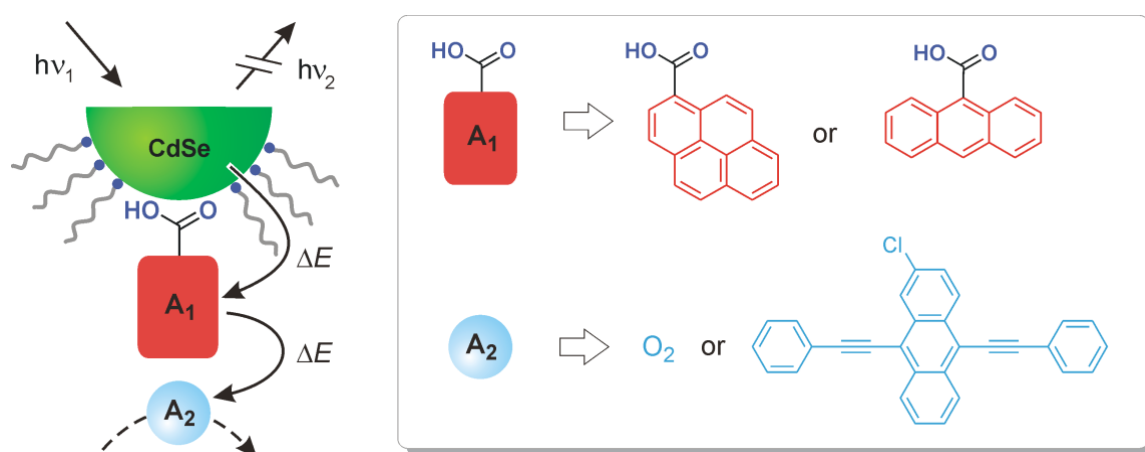
Figure 5.6. Schematic representation of nanohybrids composed of CdSe QDs and surface-adsorbed organic molecules acting as triplet energy acceptors ( A_1 ). Triplet-triplet energy transfer from the organic ligands to secondary molecular acceptors ( A_2 ) freely diffusing in solution is also shown. Adapted from reference [11]. Copyright Springer 2016.
