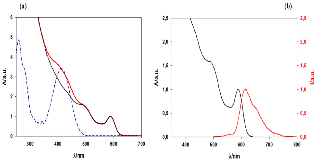
Figure 5.15 (a) Normalized absorption spectra of CdSe-4ZnS decorated with LAPEG 400 (black line), LAPEG 400 /LA-NAP (red line) and only LA-NAP (dashed blue line) in MeOH. (b) Normalized absorption spectra of LAPEG 400 decorated CdSe-4ZnSQ Ds in MeOH (black line) and triplet emission spectrum of LA-NAP (red line) recorded in CHCl 3 / CH 2 Cl 2 (1:1, v/v) at 77 K by exciting at 410 nm (time delay = 0.04 ms; gate = 2 ms; cycle = 20 ms; flash count = 1).
