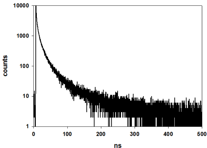
Figure 5.12 Luminescence lifetime of CdSe-4ZnS functionalized with LA-PEG 400 recorded in deaerated MeOH by exciting QDs at 405 nm. The time scale is 500 ns while the 10000 counts detected at 615 nm are reported in logarithmic scale.
