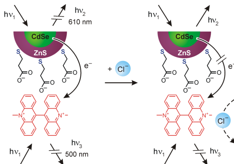
Figure 1.14. Schematic representation of \text{Cl}^- sensing occurring in CdSe-ZnS QDs and lucigenin based chemosensor. Adapted from reference [92]. Copyright Springer 2016.
