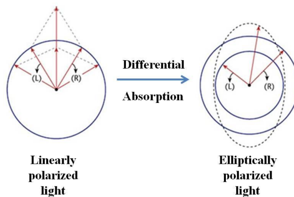
Figure 4.4 Schematic representation of the elliptical distortion of the polarization plane of the linearly polarized light due to the differential absorption of its component R and L.
