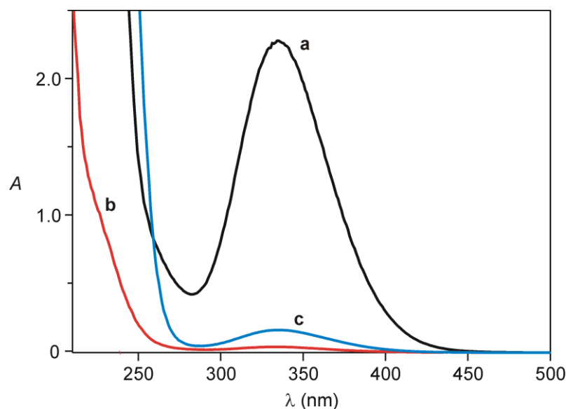
Figure 3.4. Absorption spectrum of 1.6 \times 10^{-2} M solution of LA in MeOH before (a) and after (b) treatment with BER. (c) Absorption spectrum recorded after treating the mixture in (b) with NaOH (2 equivalents with respect to LA) and 30 minutes of stirring.
