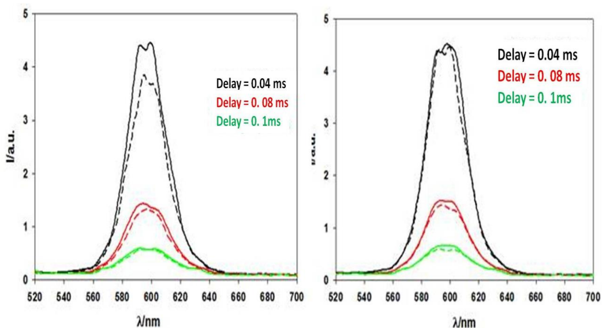
Figure 5.27 Phosphorescence emission spectra recorded at different time delays of CdSe3-1PCA (dashed lines) and CdSe3 (solid lines) on the left.
