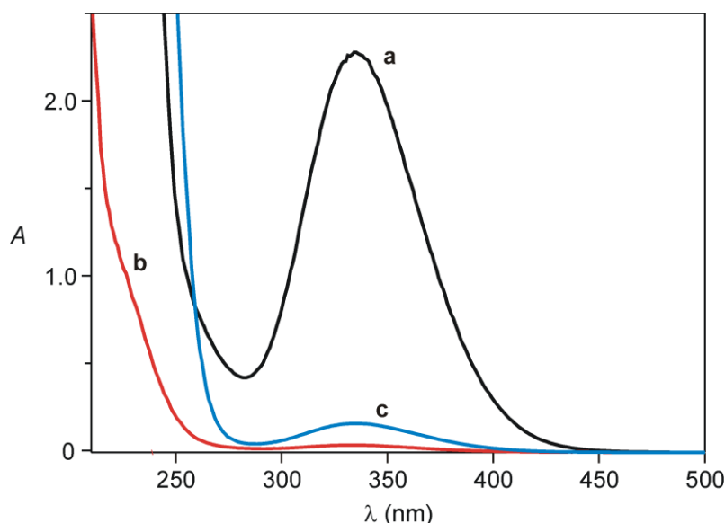
Figure 3.4. Absorption spectrum of 1.6 \times 10^{-2} M solution of LA in MeOH before (a) and after (b) treatment with BER. (c) Absorption spectrum recorded after treating the mixture in (b) with NaOH (2 equivalents with respect to LA) and 30 minutes of stirring.
