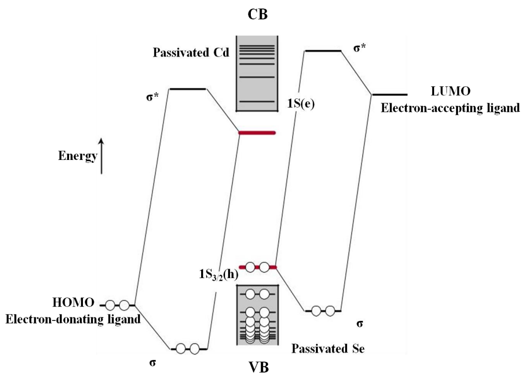
Figure 1.7 Schematic representation of electronic energy states of CdSe nanocrystals. Adapted from reference [30]. Copyright Nature Publishing Group 2016.
