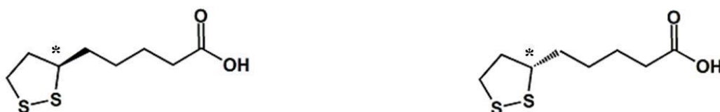
Figure 4.9 The two enantiomers of lipoic acid: the R-(+) on the left and the S-(-) on the right.
