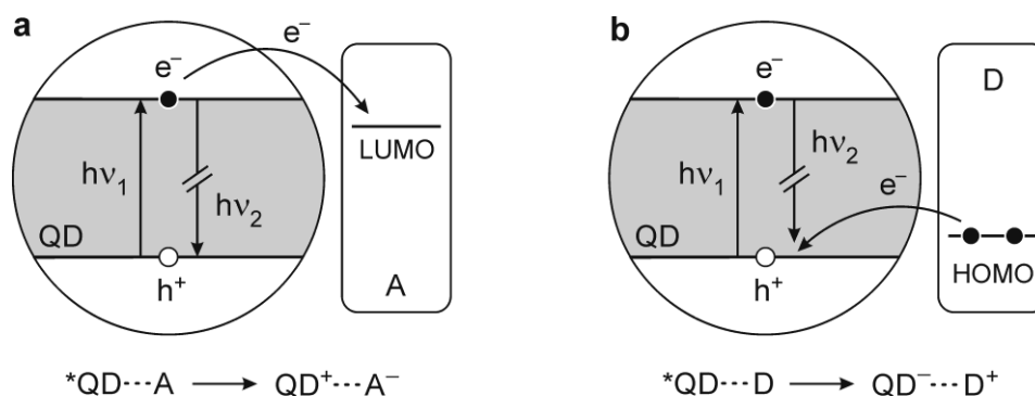
Figure 1.12 Schematization of the PET occurring (a) from the photoexcited QD to an electron acceptor A, and (b) from an electron donor D to a photoexcited QD. Adapted reference [92]. Copyright Elsevier 2014.
