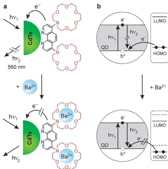
Figure 1.13 Schematic representation (a) and simplified energy-level diagram (b) of the luminescent sensing of \text{Ba}^{2+} ions with CdTe QDs functionalized with 1,10-phenanthroline-azacrown ether ligands. Adapted from reference [92]. Copyright Springer 2016.
