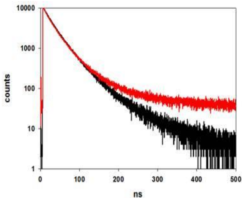
Figure 5.22 Luminescence lifetimes of CdSe3-1PCA (red decay) and CdSe3 (black decay) recorded in deaerated heptane by exciting selectively QDs at 405 nm. The time scale is 500 ns while the 10000 counts detected at 600 nm are reported in logarithmic scale.
