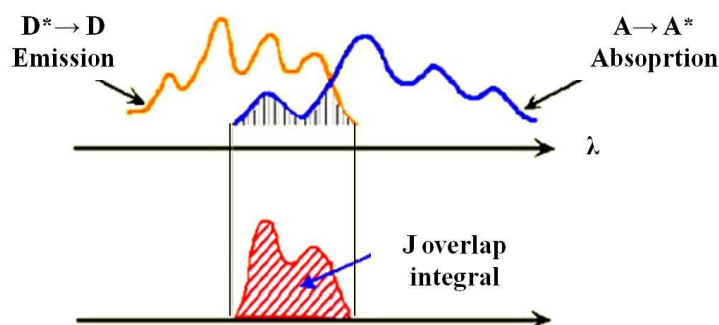
Figure 5.1 Schematic representation of J integral.
