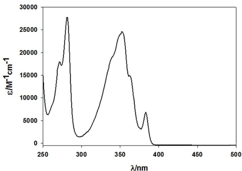
Figure 5.21 Molar Absorption Spectrum of 1-PCA recorded in THF.
