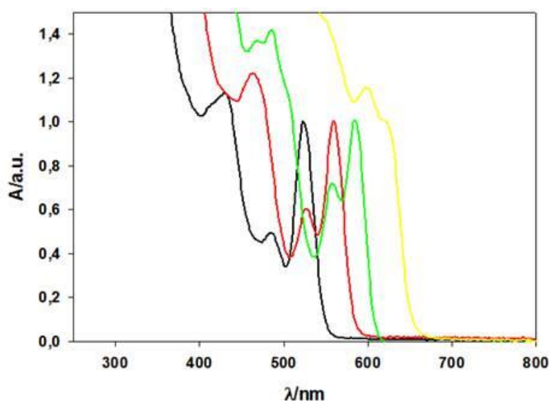
Figure 5.19 Normalized absorption spectra of CdSe 1 (black line), CdSe 2 (red line), CdSe 3 (green line) and CdSe 4 (yellow line) recorded in heptane.
