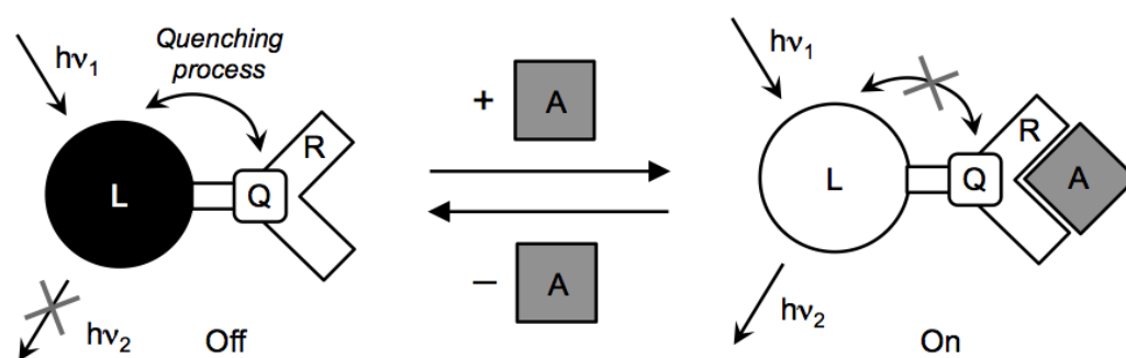
Figure 1.11 Scheme of the analyte-modulated 'turn on' photoluminescence response in a luminophore-quencher-receptor multicomponent chemosensor. Adapted from reference [92]. Copyright Springer 2016.
