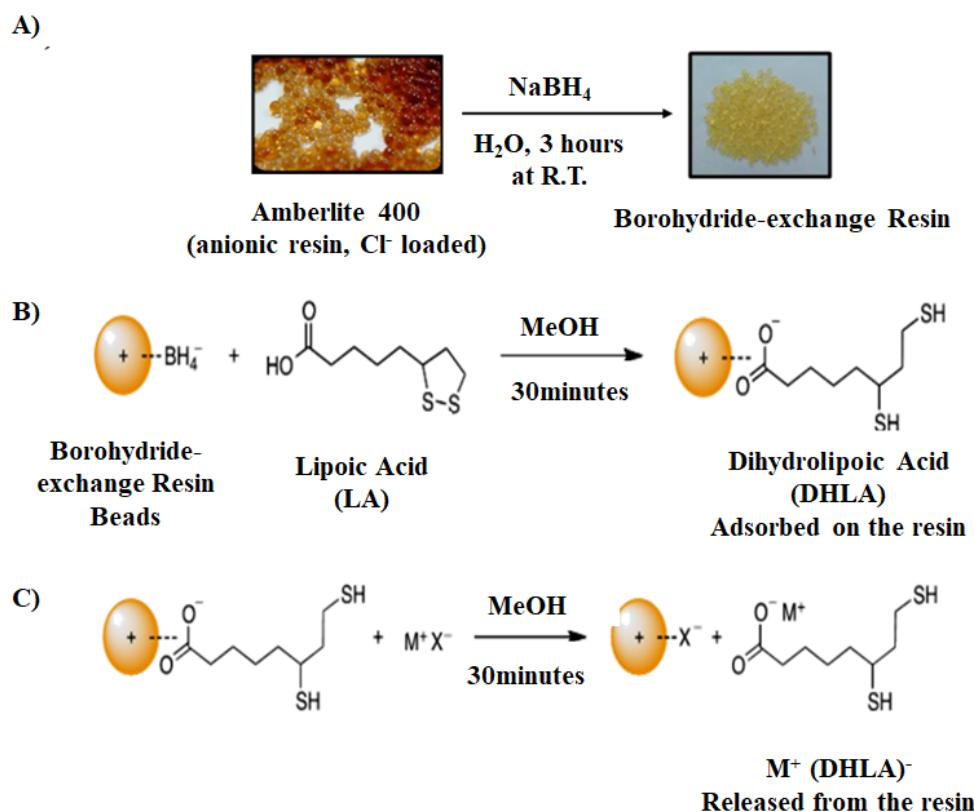
Scheme 3.1 Preparation of resin (a). Reduction of lipoic acid with a borohydride exchange resin (b). Extraction of dihydrolipoic acid from the resin beads (c). †1
