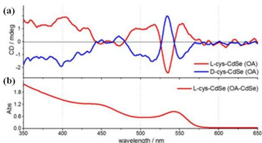
Figure 4.7 (a) CD spectrum of CdSe coated by L-Cysteine (red line) and D-Cysteine (blue line). (b) Isotropic absorption of CdSe QDs coated by L-Cysteine. Adapted from reference [25]. Copyright American Chemical Society 2011.
