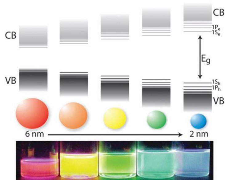
Figure 1.6 Schematic representation of size-dependent luminescence of QDs. Adapted from reference [17]. Copyright Philips Research Laboratories (Netherlands).
