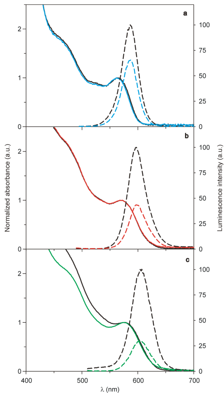
Figure 3.6. (a) Absorption (full line) and emission ( \lambda_{\text{exc}} = 485 nm; dashed line) spectra of TOP/TOPO CdSe-3ZnS QDs (sample 4 in Table 1) in \text{CHCl}_3 (black) and DHLA ^- Na ^+ capped in \text{H}_2\text{O} (blue). (b) Absorption (full line) and emission ( \lambda_{\text{exc}} = 480 nm; dashed line) spectra of TOP/TOPO CdSe-5ZnS QDs (sample 5 in Table 1) in \text{CHCl}_3 (black) and DHLA ^- Na ^+ capped in \text{H}_2\text{O} (red). (c) Absorption (full line) and emission ( \lambda_{\text{exc}} = 450 nm; dashed line) spectra of TOP/TOPO CdSe-3ZnS QDs (sample 7 in Table 1) in \text{CHCl}_3 (black) and DHLA-PEG _{400} capped in \text{H}_2\text{O} (green).
