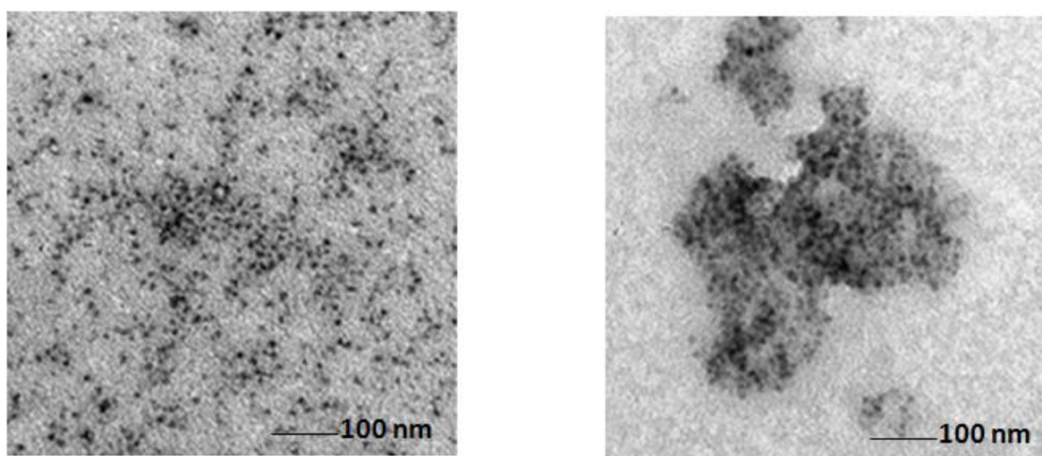
Figure 3.8. TEM images of CdSe-4ZnS QDs (sample 6 in Table 1) before (on the left) and after (on the right) ligand exchange with DHLA - Na + .
