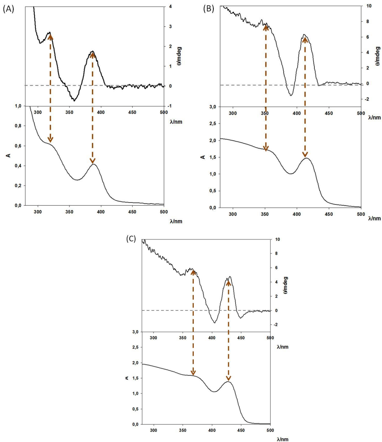
Figure 4.12 CD (at the top) and Isotropic (at the bottom) Absorption Spectra of CdS QDs samples 1 (A); 2 (B) and 3 (C).
