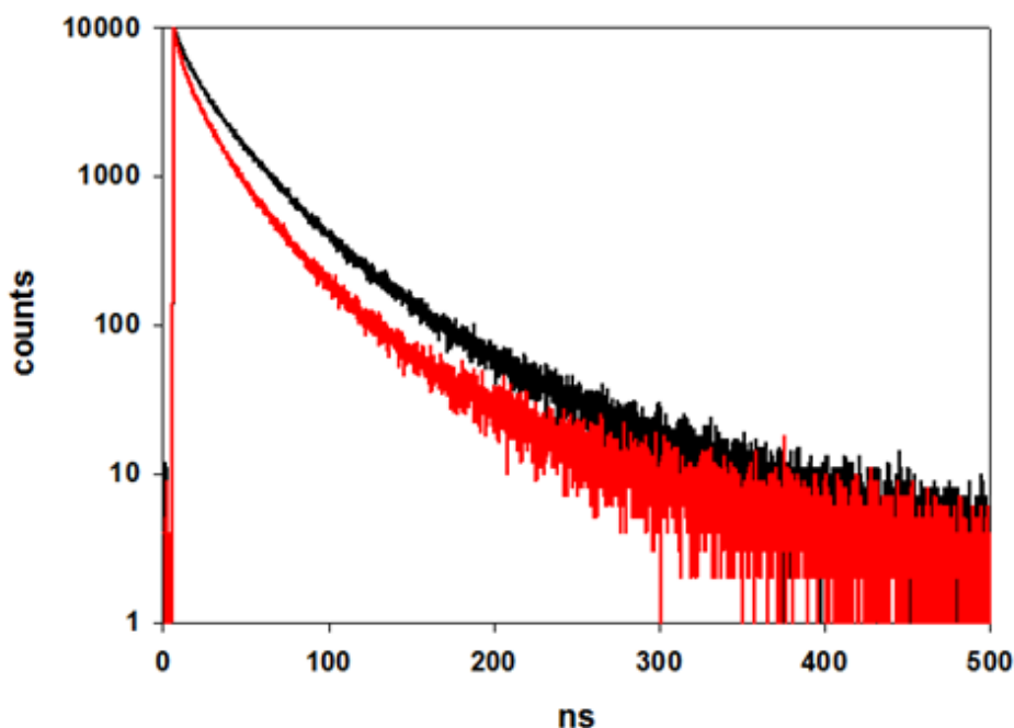
Figure 5.33 Luminescence lifetimes of CdSe2-1PCA (red decay) and CdSe2 (black decay) recorded in air-equilibrated heptane by exciting selectively QDs at 405 nm. The time scale is 500 ns while the 10000 counts detected at 570 nm are reported in logarithmic scale.
