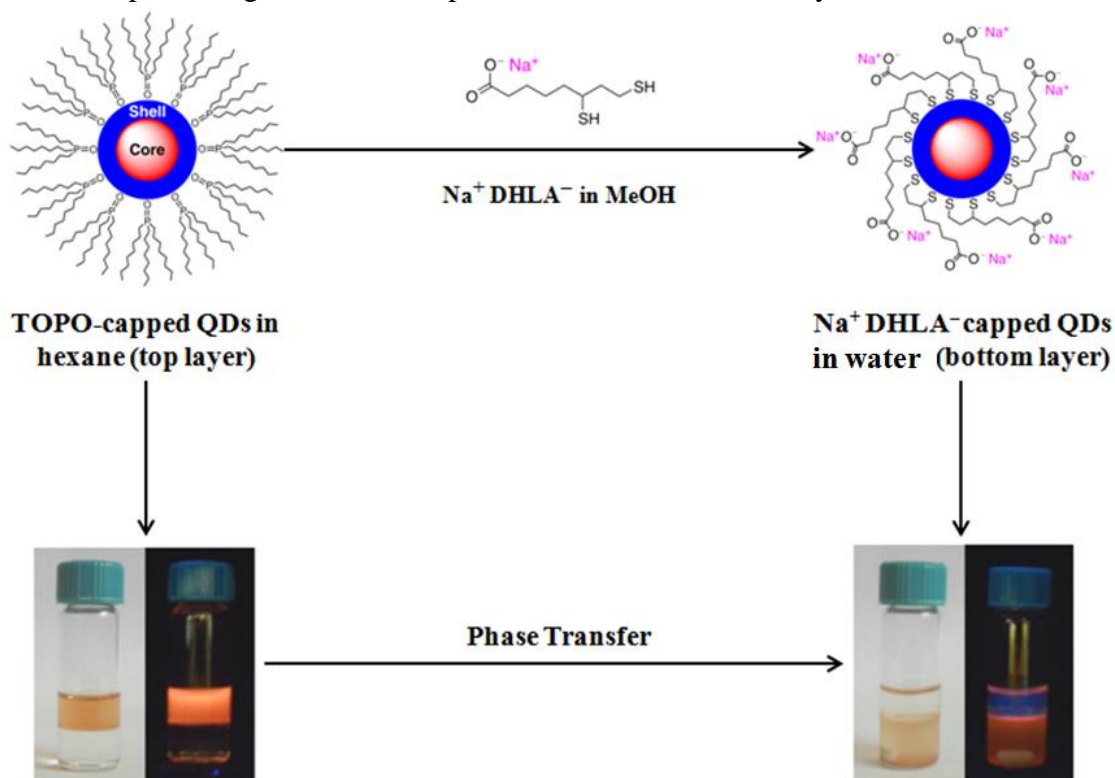
Figure 3.5. Phase transfer of hydrophobic QDs driven by ligand exchange with DHLA - ligands.
