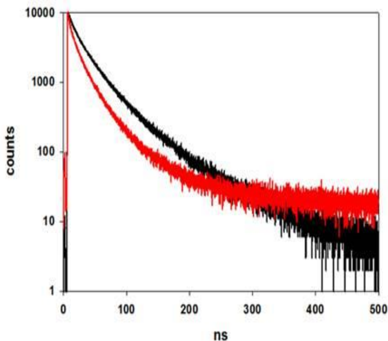
Figure 5.30 Luminescence lifetimes of CdSe2-1PCA (red decay) and CdSe2 (black decay) recorded in deaerated heptane by exciting selectively QDs at 405 nm. The time scale is 500 ns while the 10000 counts detected at 570 nm are reported in logarithmic scale.
