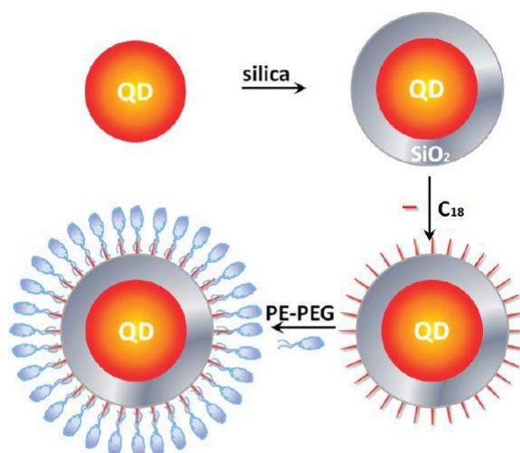
Figure 3.2 Scheme of the incorporation of a QD into SiO 2 -PE-PEG sphere. Adapted from reference [45]. Copyright American Chemical Society 2010.
