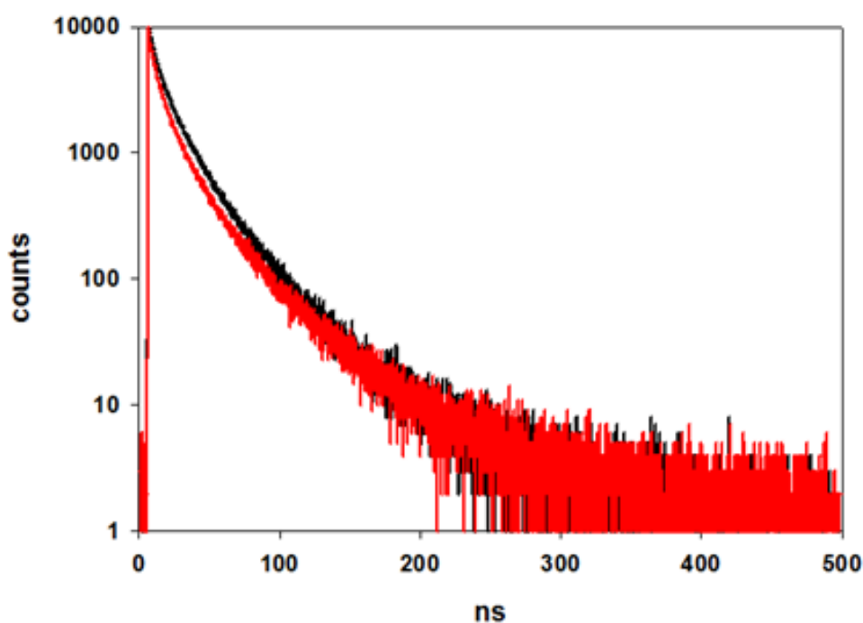
Figure 5.39 Luminescence lifetimes of CdSe4-1PCA (red decay) and CdSe4 (black decay). The decays are recorded in air-equilibrated heptane by exciting selectively QDs at 405 nm. The time scale is 500 ns while the 10000 counts detected at 636 nm are reported in logarithmic scale.
