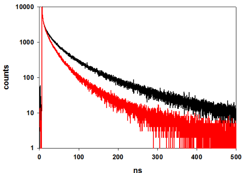
Figure 5.38 Luminescence lifetimes of CdSe1-1PCA (red decay) and CdSe1 (black decay). The decays are recorded in air-equilibrated heptane by exciting selectively QDs at 405 nm. The time scale is 500 ns while the 10000 counts detected at 540 nm are reported in logarithmic scale.
