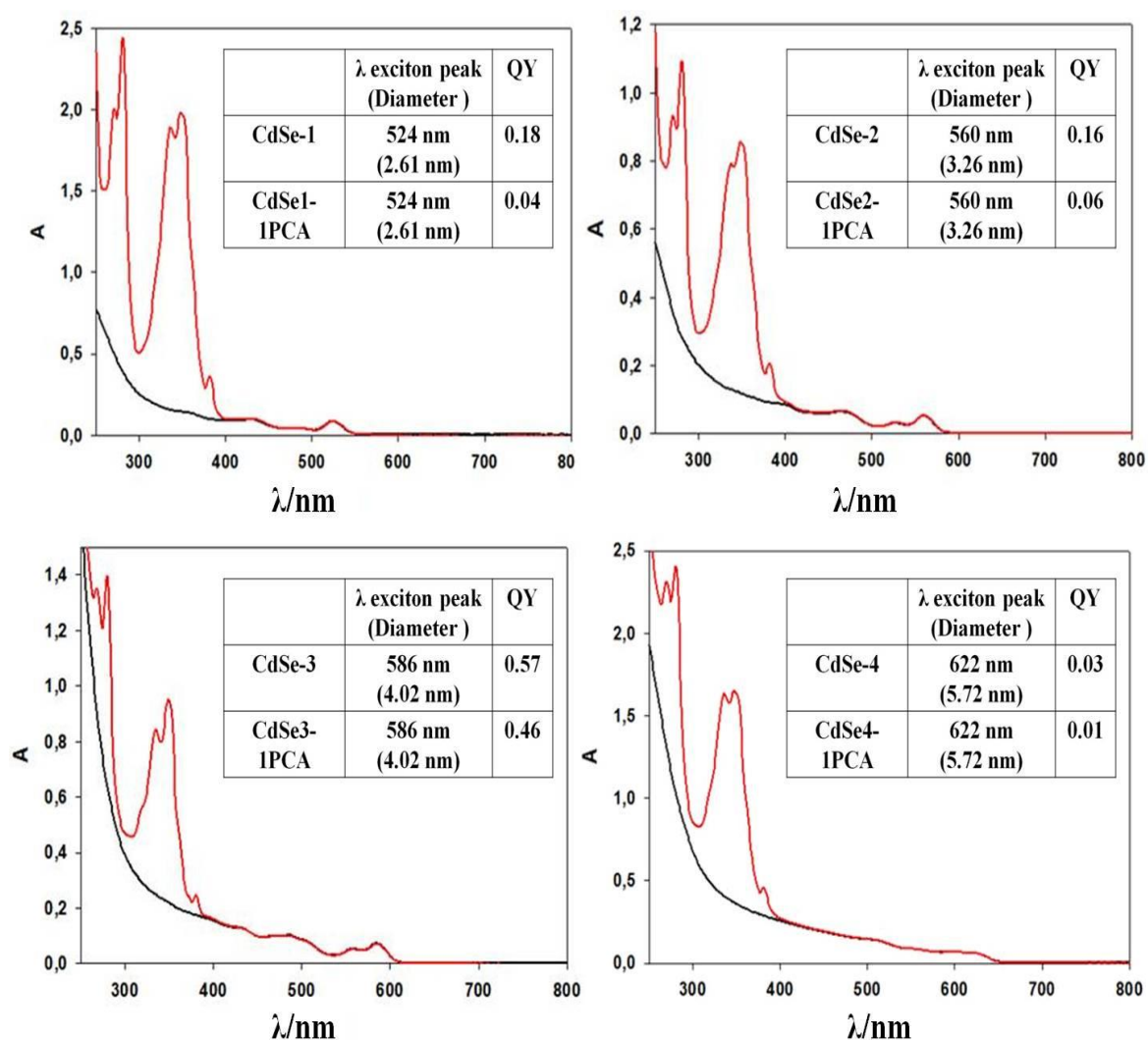
Figure 5.20 Absorption spectra of CdSe QDs before (black lines) and after (red lines) functionalization with 1-PCA, recorded with same absorbance value at the exciton peak. In the insets the photophysical and dimensional properties of each sample, with and without 1-PCA, are reported.
