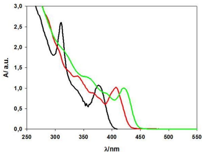
Figure 4.11 Normalized absorption spectra of CdS QDs samples 1 (black line), 2 (red line), 3 (green line) recorded in \text{CHCl}_3 .
