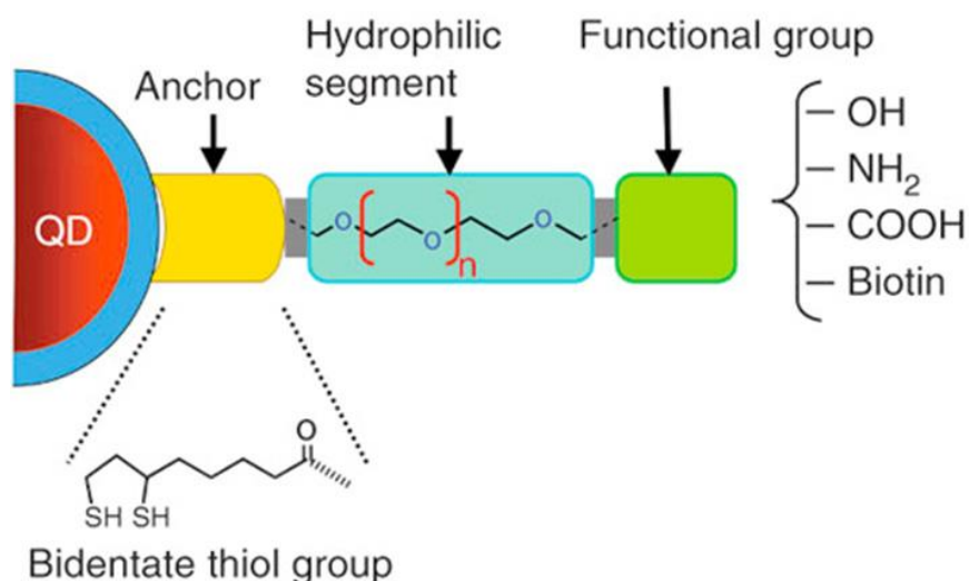
Figure 3.3. Modular design of a QD coated with hydrophilic ligands based on DHLA-PEG and bearing different terminal functional groups. Adapted from reference [69]. Copyright American Chemical Society 2007.
