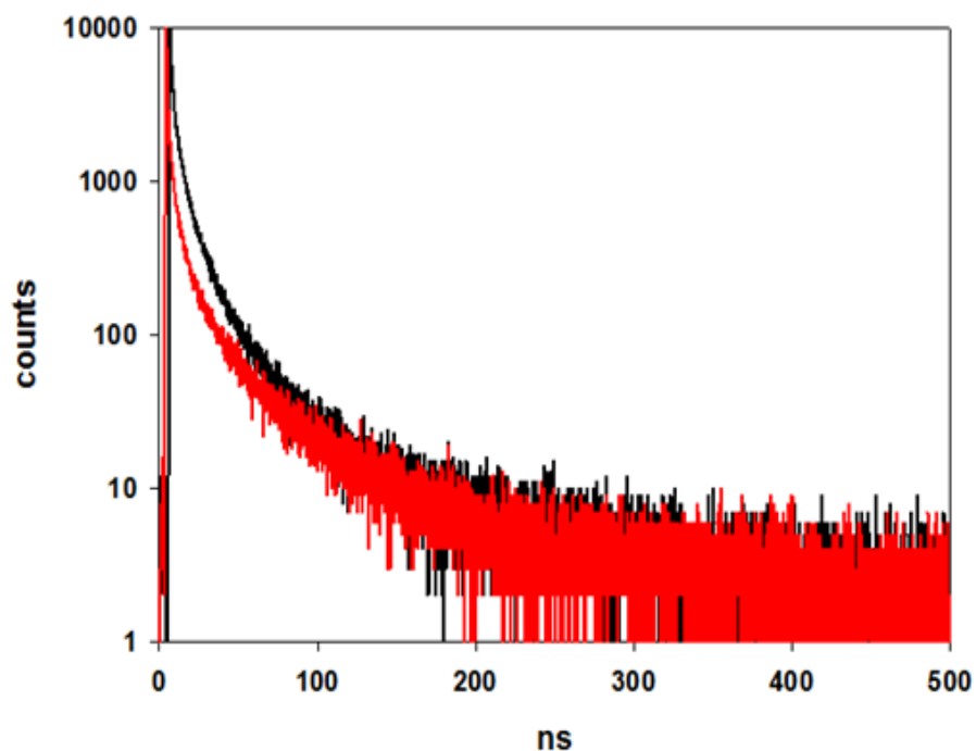
Figure 5.14 Luminescence lifetimes of CdSe-4ZnS decorated with LAPEG 400 (black decay), LAPEG 400 /LA-Ru (red decay) recorded in deaerated MeOH by exciting selectively QDs at 600 nm. The time scale is 500 ns while the 10000 counts detected at 615 nm are reported in logarithmic scale.
