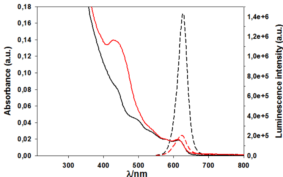
Figure 6.4 Absorption (full lines) and luminescence (dashed lines) spectra of TOPO/TOP capped QDs in hexane (black) and LAPEG 400 /LARu coated QDs (red). Luminescence spectra are recorded by exciting at 460 nm.
