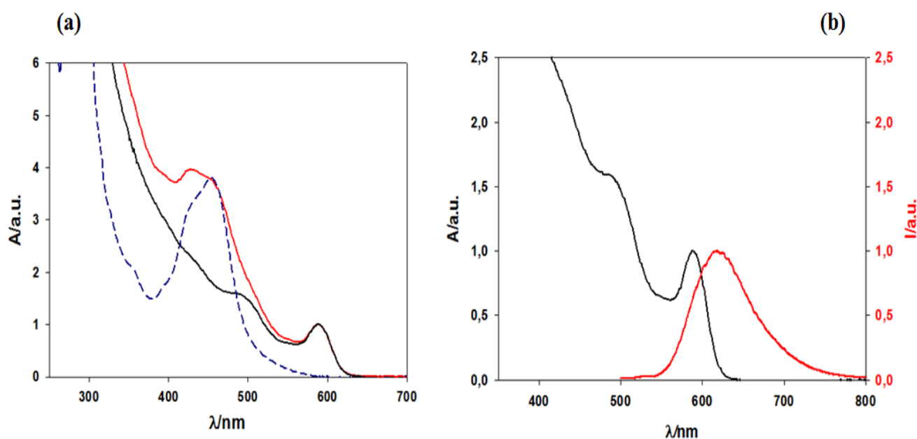
Figure 5.13 (a) Normalized absorption spectra of CdSe-4ZnS decorated with LAPEG 400 (black line), LAPEG 400 /LA-Ru (red line), and only LA-Ru (dashed blue line) in MeOH. (b) Normalized absorption spectra of LAPEG 400 decorated CdSe-4ZnS QDs in MeOH (black line) and triplet emission spectrum of LA-Ru (red line) recorded in MeOH by exciting at 450 nm.
