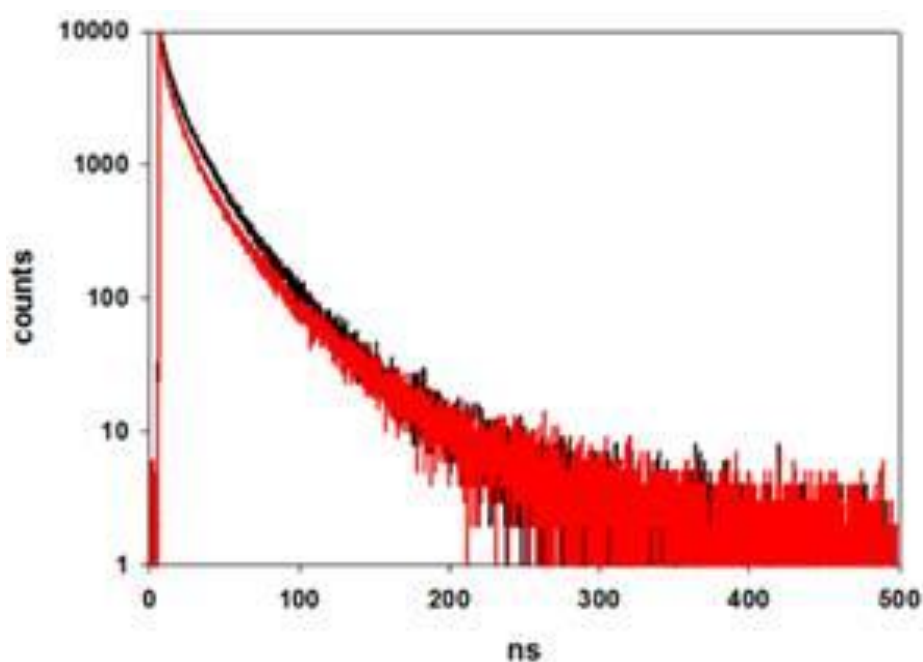
Figure 5.37 Luminescence lifetimes of CdSe4-1PCA (red decay) and CdSe4 (black decay). The decays are recorded in deaerated heptane by exciting selectively QDs at 405 nm. The time scale is 500 ns while the 10000 counts detected at 636 nm are reported in logarithmic scale.
