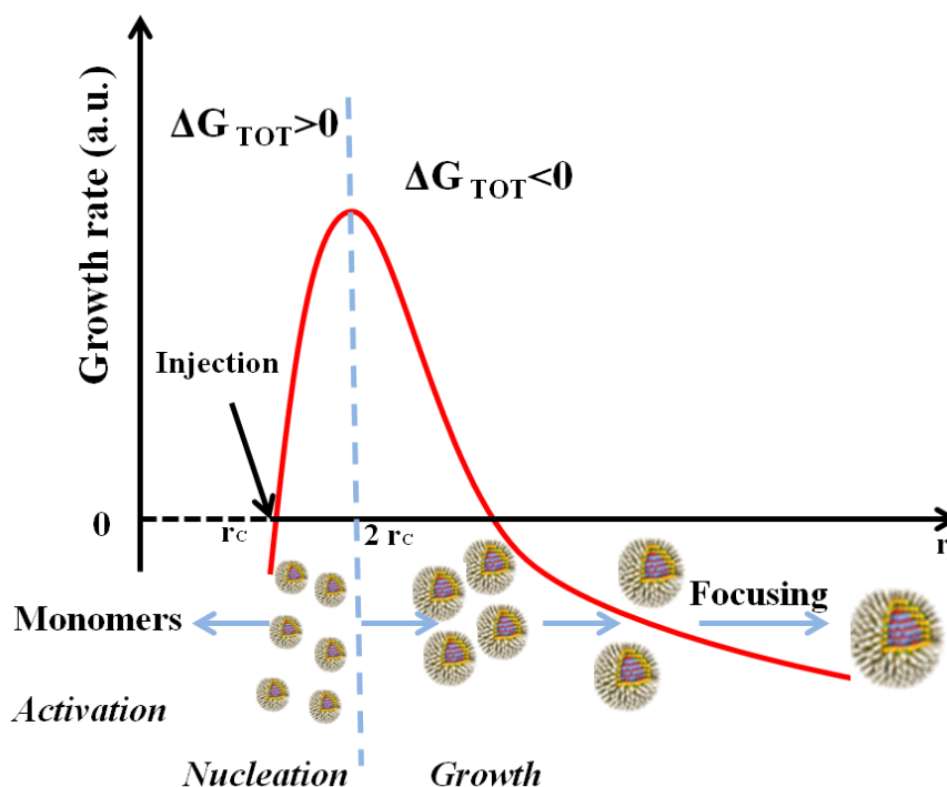
Figure 1.8 Schematic representation of the regimes of the hot injection method.
