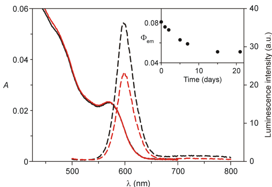
Figure 3.9. Absorption (full lines) and emission ( \lambda_{exc} = 480 nm; dashed lines) spectra of CdSe-5ZnS QDs (sample 5 in Table 1, 130 nM) capped with DHLA - Na + in water, freshly prepared (black) and after 21 days of storage at 5°C (red). The inset shows the evolution of the luminescence quantum yield over time.
