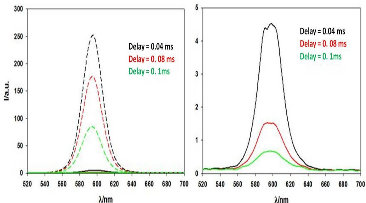
Figure 5.24 Phosphorescence emission spectra recorded at different time delays of CdSe3-1PCA (dashed lines) and CdSe3 (solid lines) on the left.
