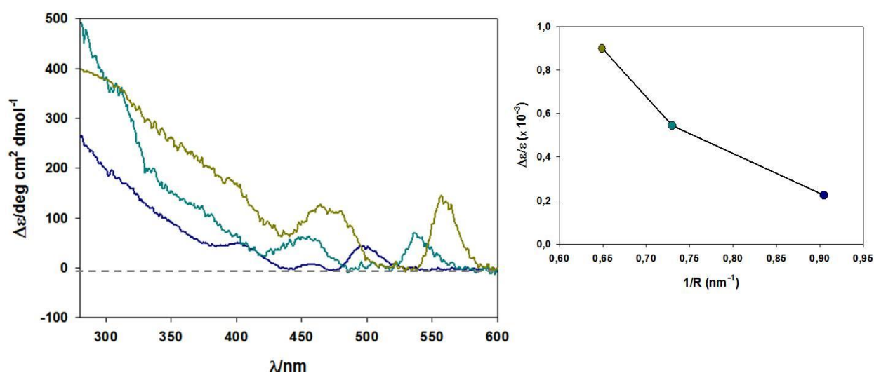
Figure 4.17 Differential Absorption Coefficient Spectra of CdSe QDs samples 1 (dark blue line), 2 (dark cyan line) and 3 (dark yellow line). In the inset the dissymmetry factor is reported as function of the size of QDs.
