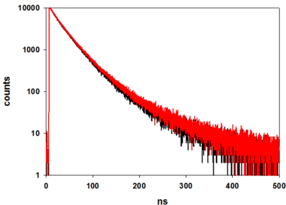
Figure 5.29 Comparison between the luminescence decay of CdSe3 in deaerated (red decay) and air-equilibrated (black decay) heptane.
