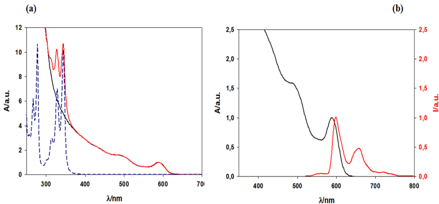
Figure 5.17 (a) Normalized absorption spectra of CdSe-4ZnS decorated with LAPEG 400 (black line), LAPEG 400 /LA-PYR (red line) and only LA-PYR (dashed blue line) in MeOH. (b) Normalized absorption spectra of LAPEG 400 decorated CdSe-4ZnSQ Ds in MeOH (black line) and triplet emission spectrum of LA-PYR (red line) recorded in CHCl 3 / CH 2 Cl 2 (1:1, v/v) at 77 K by exciting at 410 nm (time delay = 0.04 ms; gate = 2 ms; cycle = 20 ms; flash count = 1).
