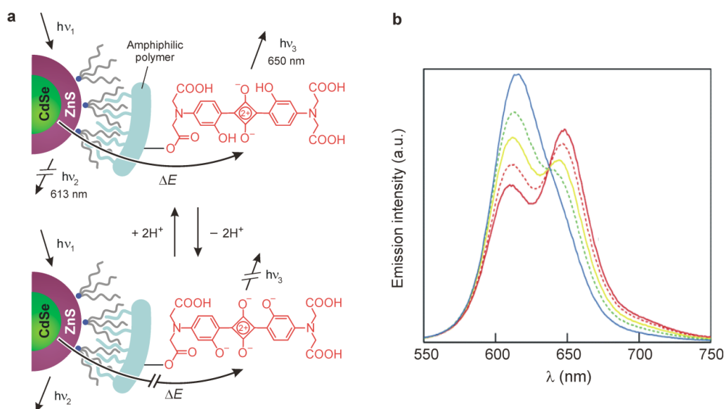
Figure 5.3 (a) Scheme of a luminescent pH sensor composed of CdSe-ZnS QDs functionalized with a pH-sensitive squaraine. (b) Emission spectra of the QD-squaraine conjugate at different pH values (H 2 O, \lambda_{exc} = 380 nm): 6.0 (red solid line); 7.0 (orange dotted line); 8.0 (yellow solid line); 9.0 (green dotted line); 10 (blue solid line). Adapted by permission from reference [4]. Copyright Springer 2016.
