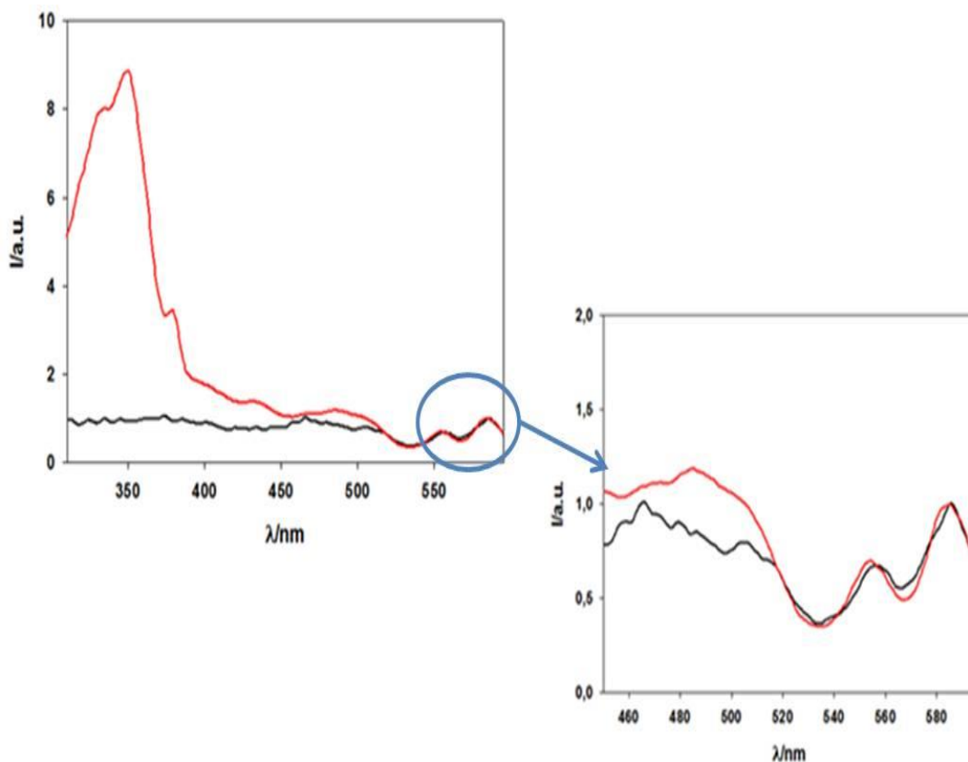
Figure 5.25 Phosphorescence excitation spectra of CdSe3-1PCA (red line) and CdSe3 (black line). The spectra are recorded in the same experimental conditions: 600 nm as emission wavelength, delay time 0.04 ms, gate 2 ms, cycle 20 ms, flash count 1.
