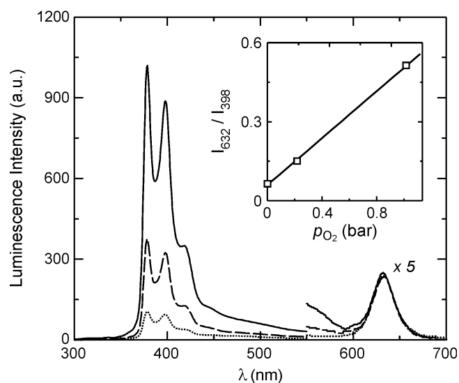
Figure 1.16 Luminescence spectra of the QD-pyrene nanohybrids in chloroform as a function of the O 2 pressure: 0 (—), 0.213 (---) and 1.013 (·····) bar. The spectra have been recorded by exciting at 275 nm. The inset shows the linear correlation between the ratiometric photoluminescence response (calculated as the QD-to-pyrene emission intensity ratio) and the O 2 partial pressure. Adapted from reference [100]. Copyright RSC Publishing 2011.
