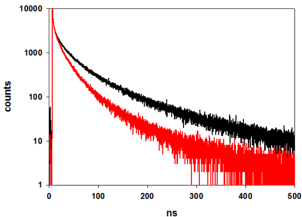
Figure 5.38 Luminescence lifetimes of CdSe1-1PCA (red decay) and CdSe1 (black decay) The decays are recorded in air-equilibrated heptane by exciting selectively QDs at 405 nm. The time scale is 500 ns while the 10000 counts detected at 540 nm are reported in logarithmic scale.
