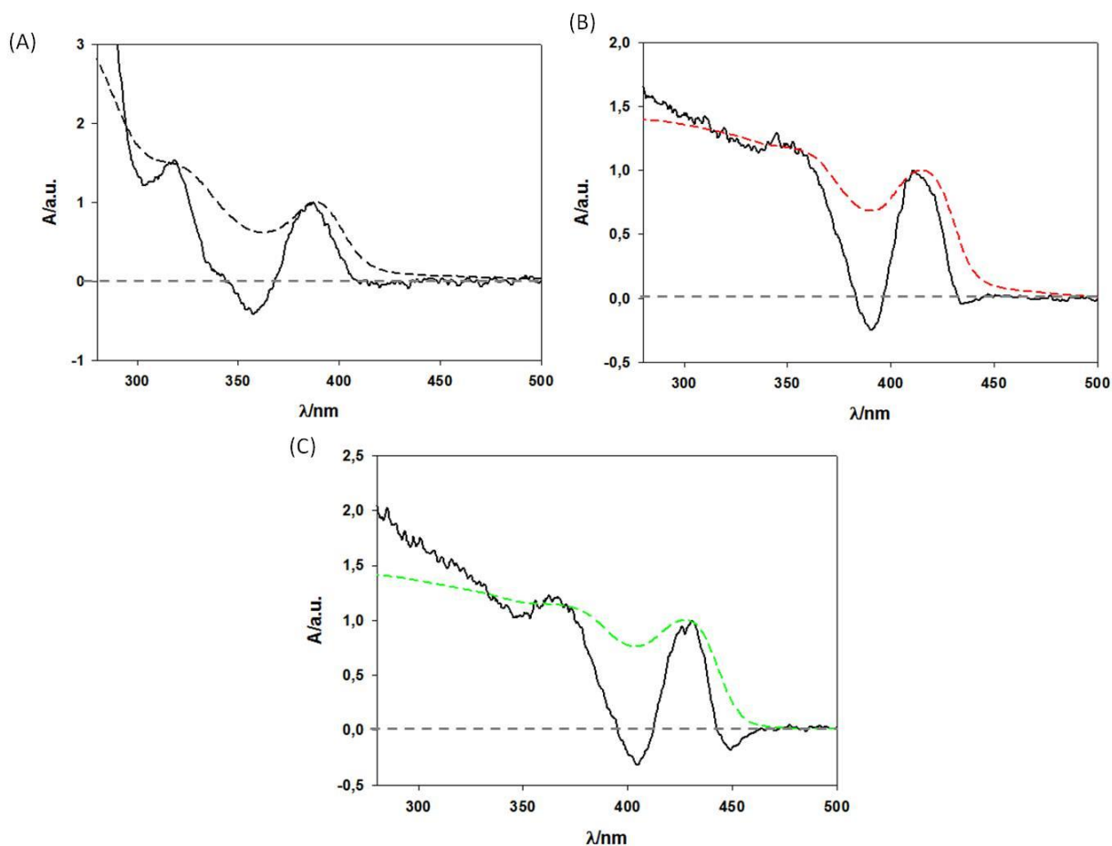
Figure 4.13 Normalized CD (black solid line) and isotropic spectra (dashed lines) at the first exciton transition of CdS samples 1 (A), 2 (B) and 3 (C).
