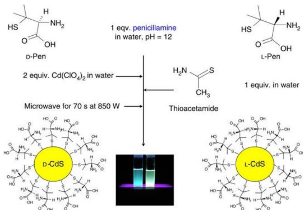
Figure 4.8 Schematic representation of the synthesis of chiral CdS QDs. Adapted from reference [29]. Copyright Nature Publishing Group 2015.
