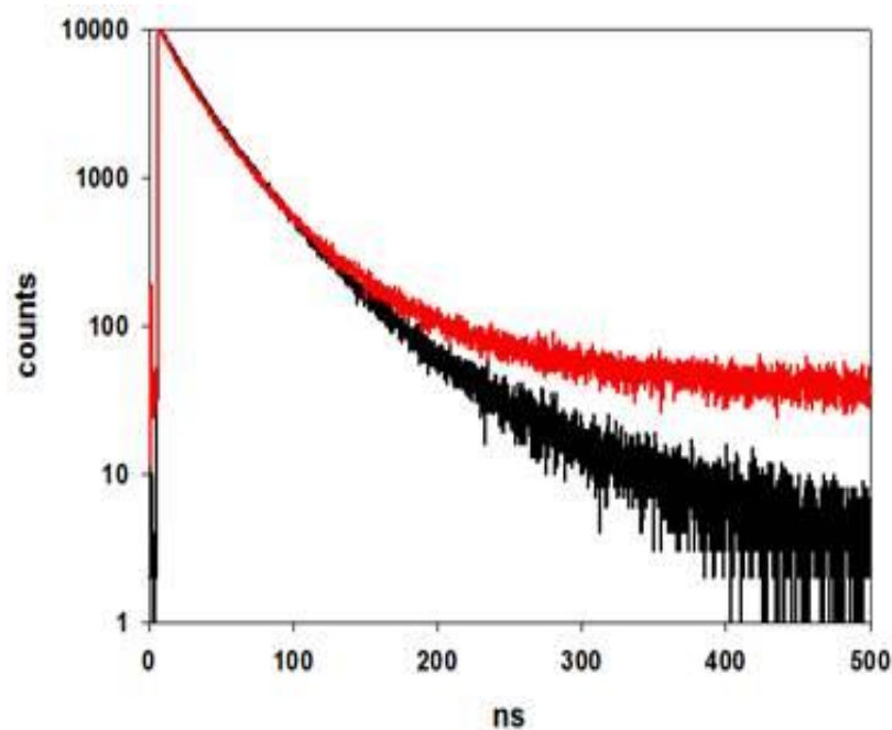
Figure 5.22 Luminescence lifetimes of CdSe3-1PCA (red decay) and CdSe3 (black decay) recorded in deaerated heptane by exciting selectively QDs at 405 nm.
