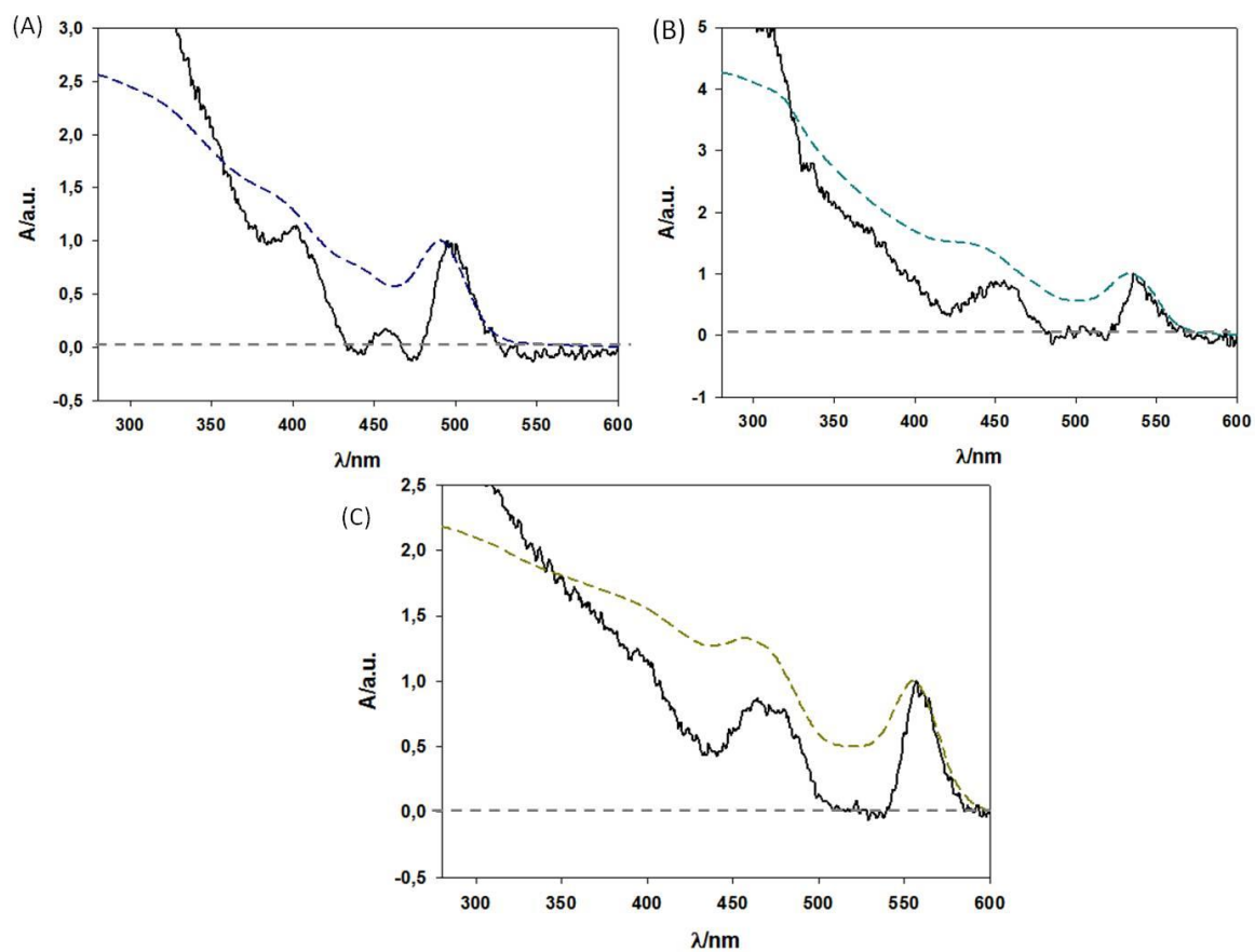
Figure 4.16 Normalized CD (black solid line) and isotropic spectra (dashed lines) at the first exciton transition of CdSe samples 1 (A), 2 (B) and 3 (C).
