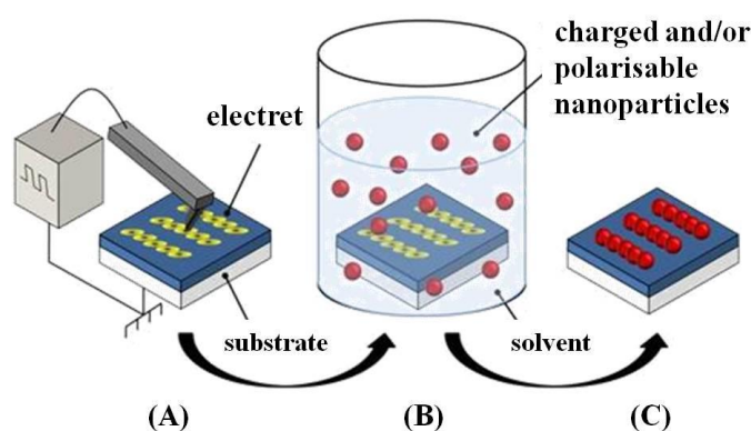
Figure 6.1 Schematic representation of AFM nano-xerography: (A) electrical charge injection by AFM in a thin film, (B) dipping in a colloidal solution of charged and/or polarizable nanoparticles, (C) directed assembly of nanoparticles on the charged patterns.
