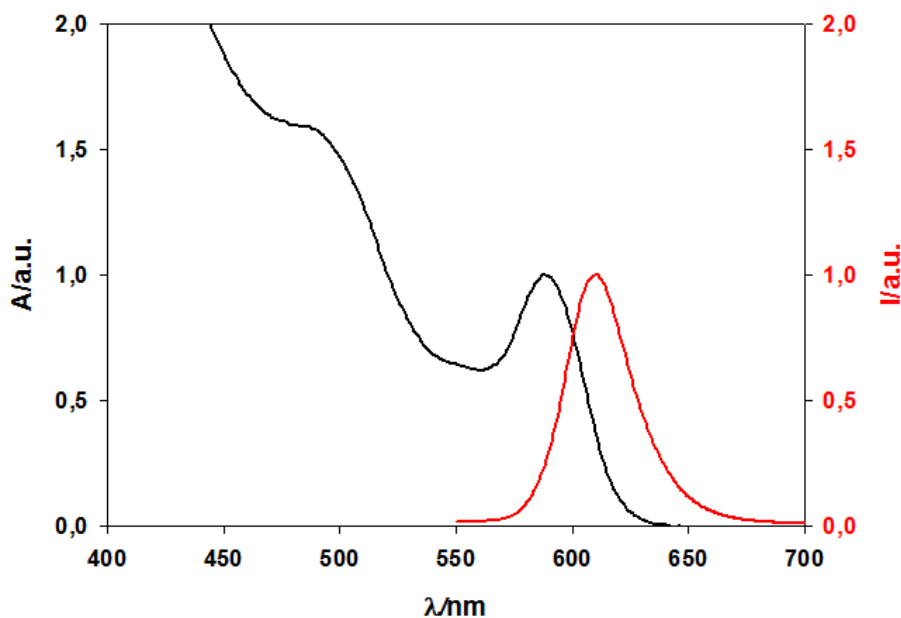
Figure 5.11 Normalized absorption (black line) and emission (red line) spectra in MeOH of CdSe-4ZnS QDs functionalized with LA-PEG 400 .
