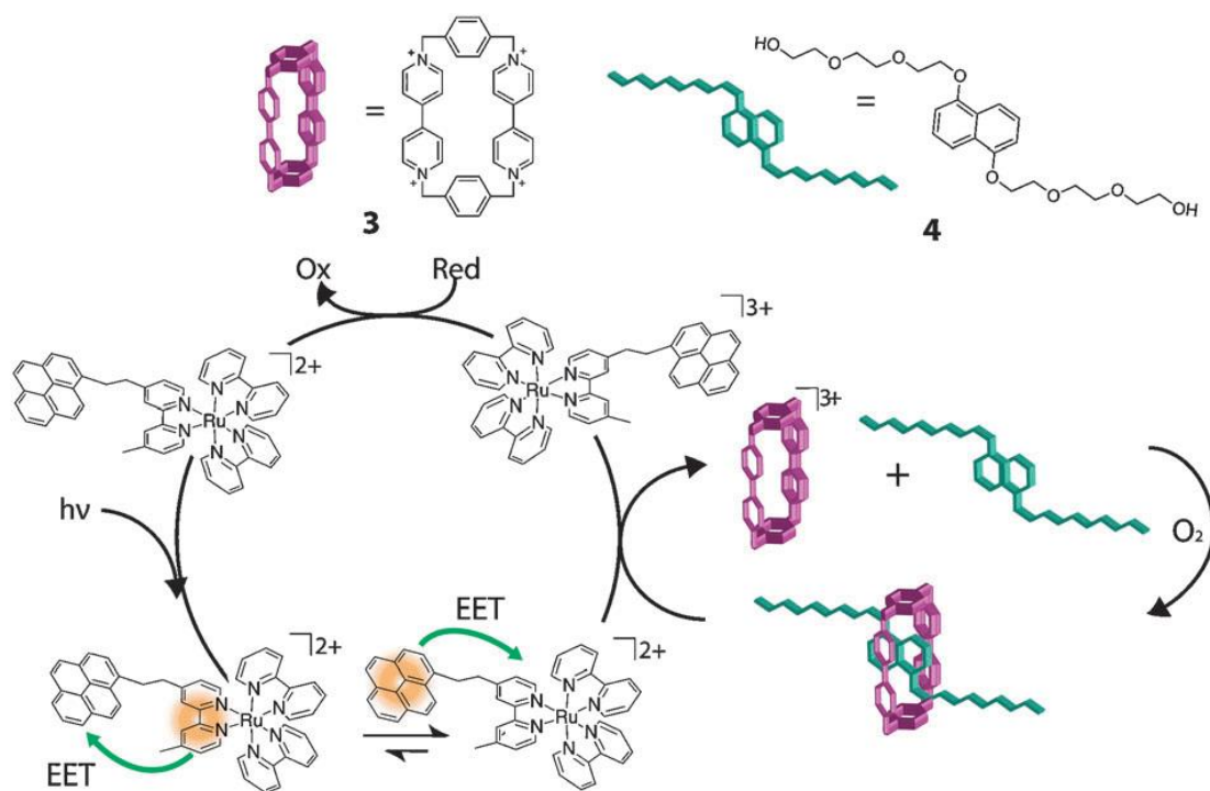
Figure 5.8 Schematic representation of REET occurring in photocatalytic electron pumping driving a molecular piston. The irradiation of a suitable external photosensitizer, in the presence of a sacrificial reductant, induces reduction and disassembly of the pseudorotaxane, while reassembly of the molecular piston is restored in the presence of oxygen. Adapted from reference [20]. Copyright RSC publishing 2012.
