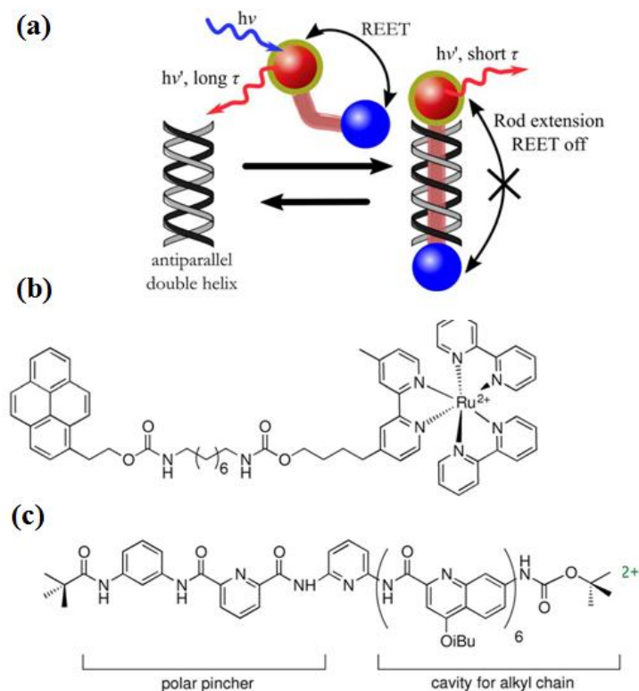
Figure 5.9 Modulation of REET in a dynamic foldaxane (a); molecular structures of molecular thread (b) and foldamer (c), which dimerizes in solution giving (c) 2 . Adapted from reference [21]. Copyright Wiley-VCH 2016.
