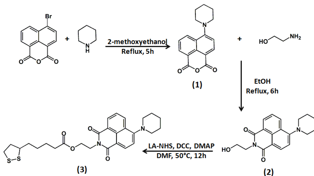
Scheme 2.3 Synthetic route for preparing LA-NAP.
