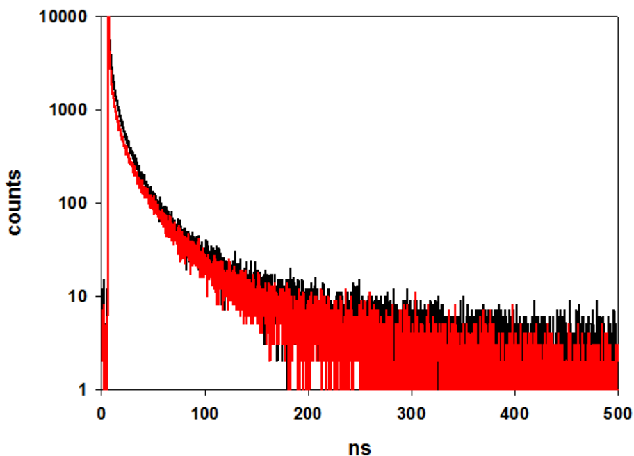
Figure 5.16 Luminescence lifetimes of CdSe-4ZnS decorated with LAPEG 400 (black decay), LAPEG 400 /LA-NAP (red decay) recorded in deaerated MeOH by exciting selectively QDs at 600 nm. The time scale is 500 ns while the 10000 counts detected at 615 nm are reported in logarithmic scale.
