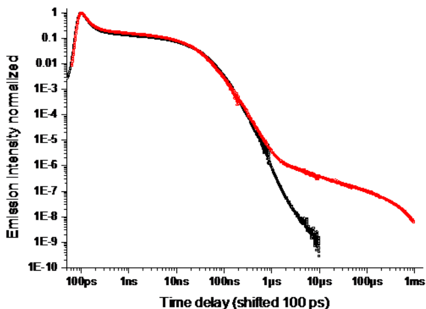
Figure 5.31 Emission decay of CdSe2 (black line) and CdSe2-1PCA (red line) in deaerated heptane; recorded with a streak camera and by exciting at 465 nm.
