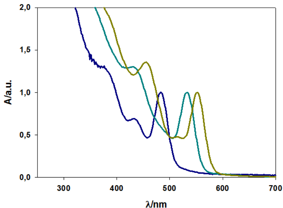
Figure 4.10 Normalized absorption spectra of CdSe QDs samples 1 (dark blue line), 2 (dark cyan line) and 3 (dark yellow line) recorded in \text{CHCl}_3 .
