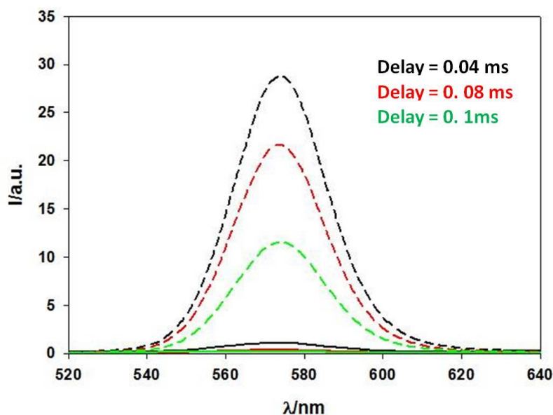
Figure 5.32 Phosphorescence emission spectra recorded at different time delays of CdSe2-1PCA (dashed lines) and CdSe2 (solid lines). All the spectra have been recorded in deaerated heptane and by exciting selectively QDs at 500 nm. Other instrumental conditions are: gate 2 ms; cycle=20 ms; flash count=1.
