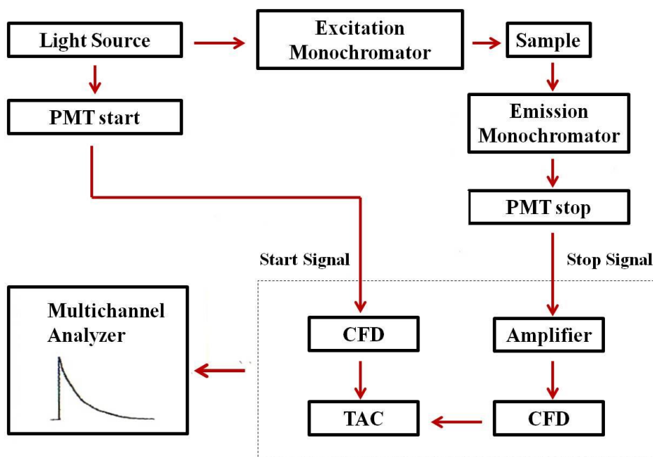
Figure 2.1 Schematization of TCSPC instrumentation.
