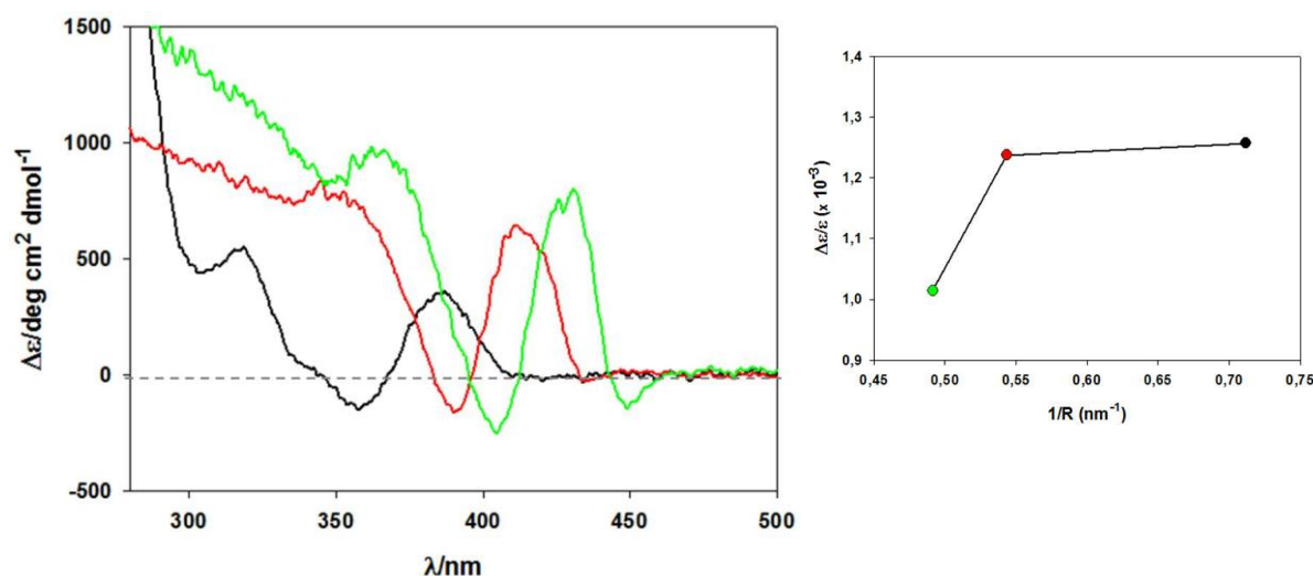
Figure 4.14 Differential Absorption Coefficient Spectra of CdS QDs samples 1 (black line), 2 (red line) and 3 (green line). In the inset the dissymmetry factor is reported as function of the size of QDs.
