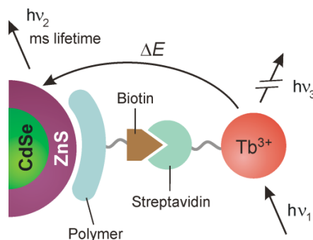
Figure 5.4 A nano hybrid consisting of a surface-biotinylated QD bound to a terbium complex-streptavidin conjugate. Upon light excitation of the lanthanide complex in the UV, energy is transferred to the QD, thus resulting in luminescence quenching of Tb and the appearance of a long-lived QD luminescence with millisecond decay times. Adapted by permission from reference [6]. Copyright Springer 2016.
