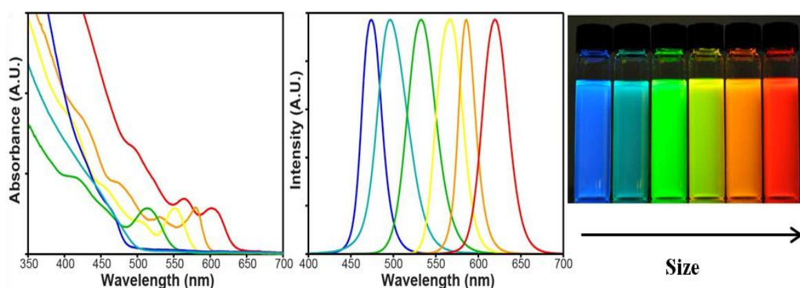
Figure 1.9 Schematic representation of the absorption and luminescence spectra of high-quality CdSe QDs of different size.
