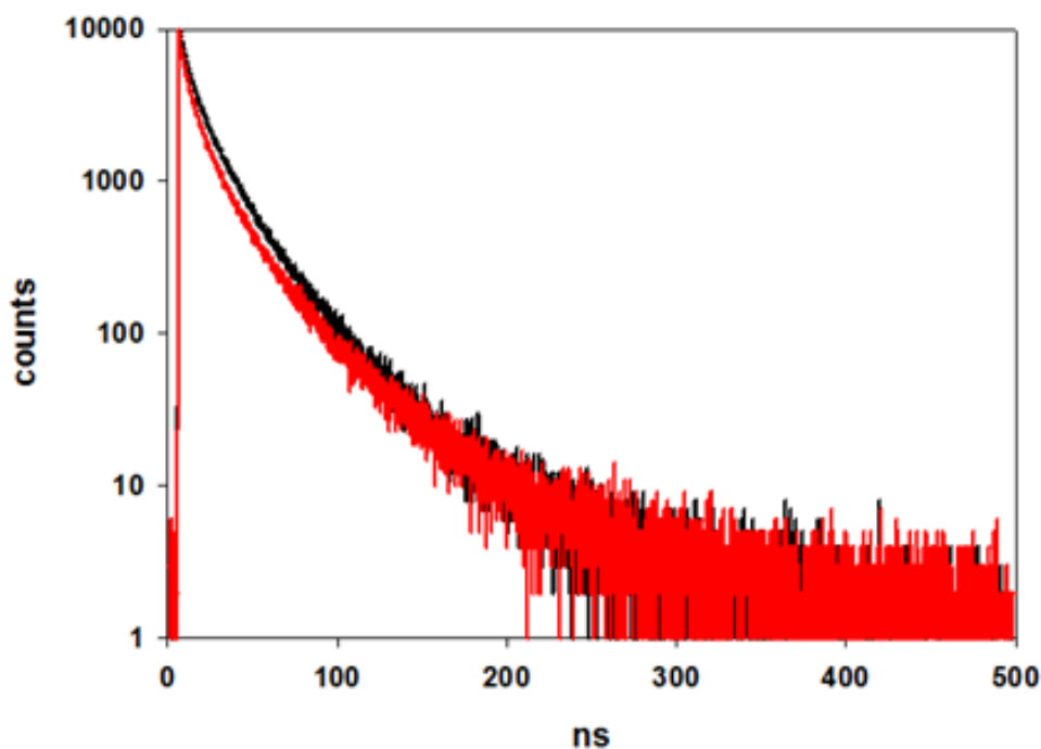
Figure 5.39 Luminescence lifetimes of CdSe4-1PCA (red decay) and CdSe4 (black decay). The decays are recorded in air-equilibrated heptane by exciting selectively QDs at 405 nm. The time scale is 500 ns while the 10000 counts detected at 636 nm are reported in logarithmic scale.
