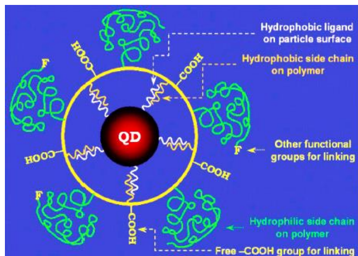
Figure 3.1. Schematic representation of an amphiphilic polymer-coated QD. Adapted from reference [33]. Copyright American Chemical Society 2007.
