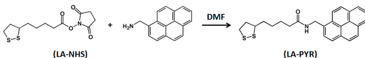
Scheme 2.2 Synthetic route for preparing LA-PYR.
