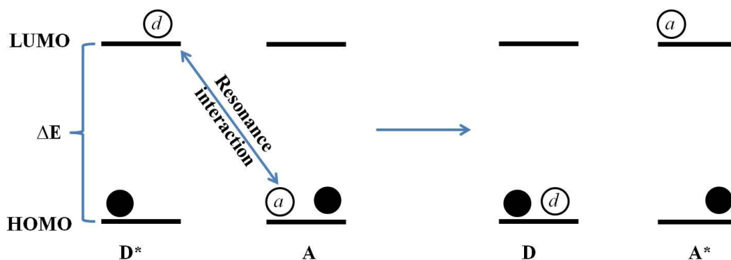
Figure 5.2 Schematic representation of Coulombic mechanism of energy transfer.
