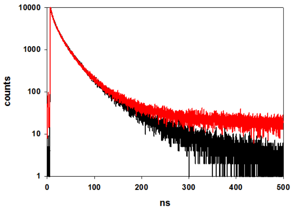
Figure 5.34 Comparison between the luminescence decay of CdSe 2 -1PCA in deaerated (red decay) and air-equilibrated (black decay) heptane.
