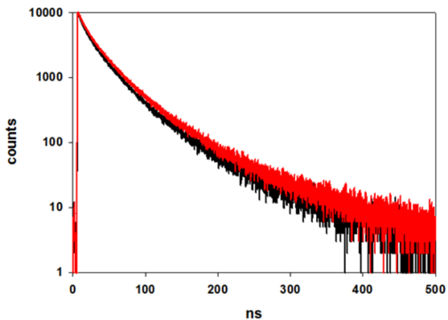
Figure 5.35 Comparison between the luminescence decay of CdSe 2 in deaerated (red decay) and air-equilibrated (black decay) heptane.
