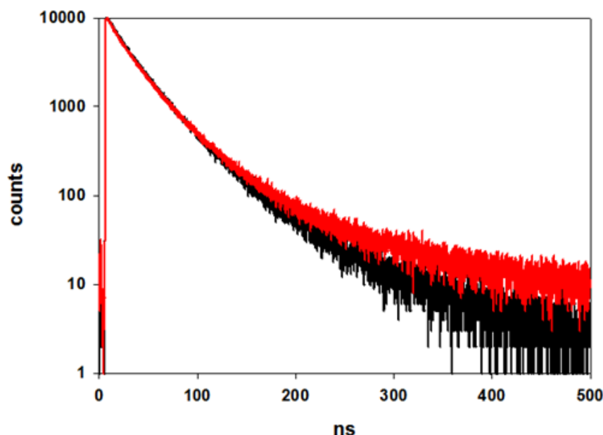
Figure 5.26 Luminescence lifetimes of CdSe3-1PCA (red decay) and CdSe3 (black decay) recorded in air-equilibrated heptane by exciting selectively QDs at 405 nm. The time scale is 500 ns while the 10000 counts detected at 600 nm are reported in logarithmic scale.
