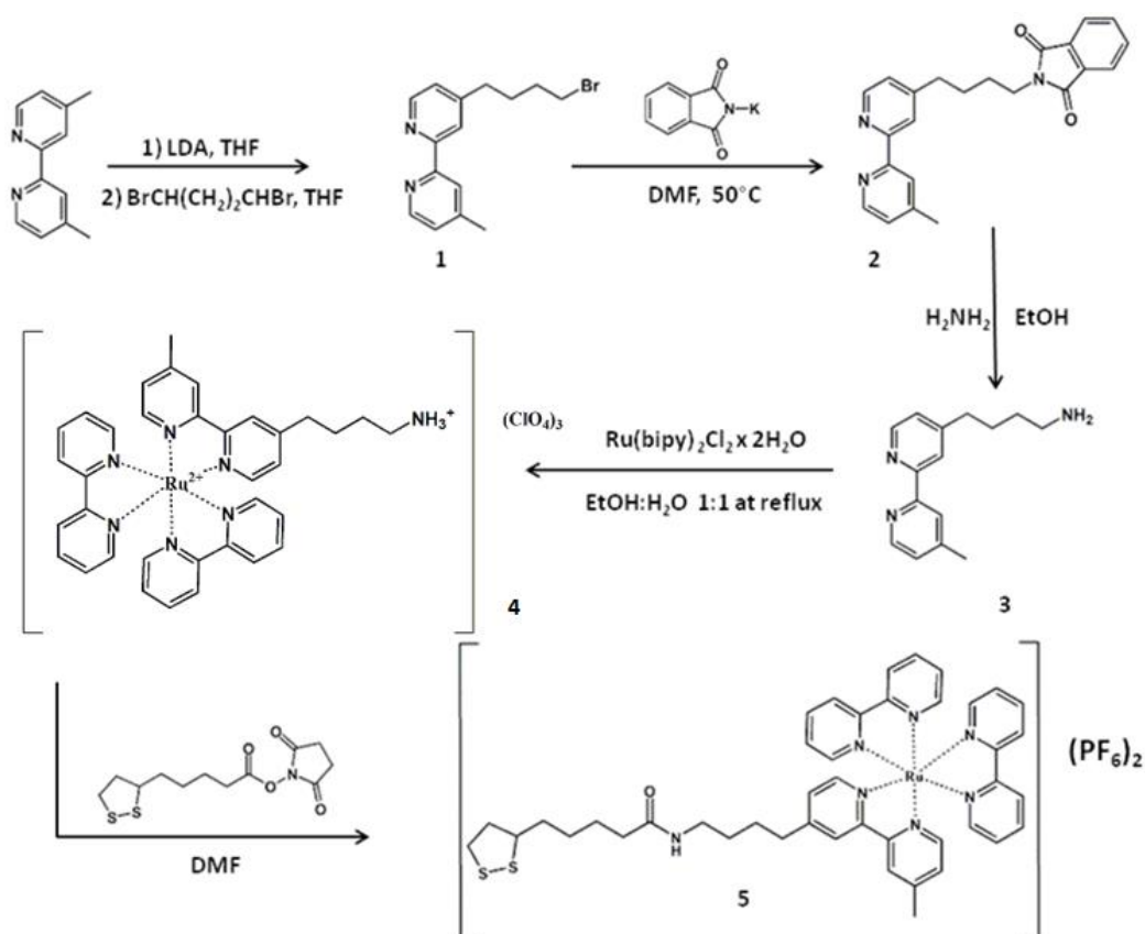
Scheme 2.4 Synthetic route for preparing LA-Ru.
