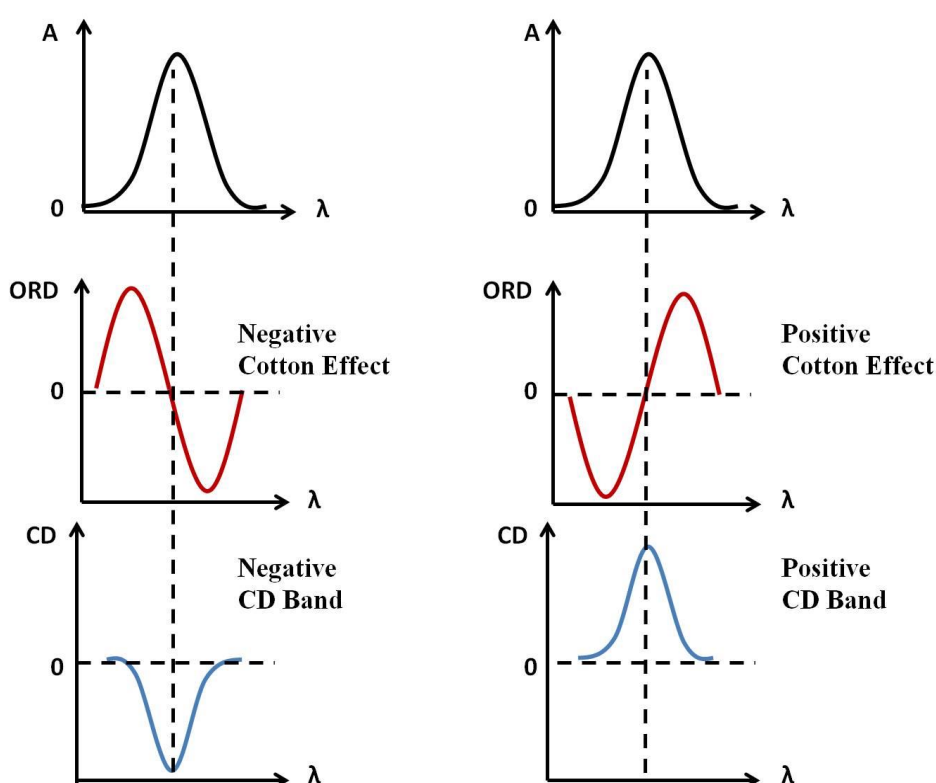
Figure 4.6 Relationships between the isotropic absorption (at the top), the optical rotation dispersion (in the middle) and circular dichroism (at the bottom) bands.
