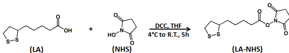
Scheme 2.1 Synthetic route for preparing the activated ester of lipoic acid (LA-NHS).
