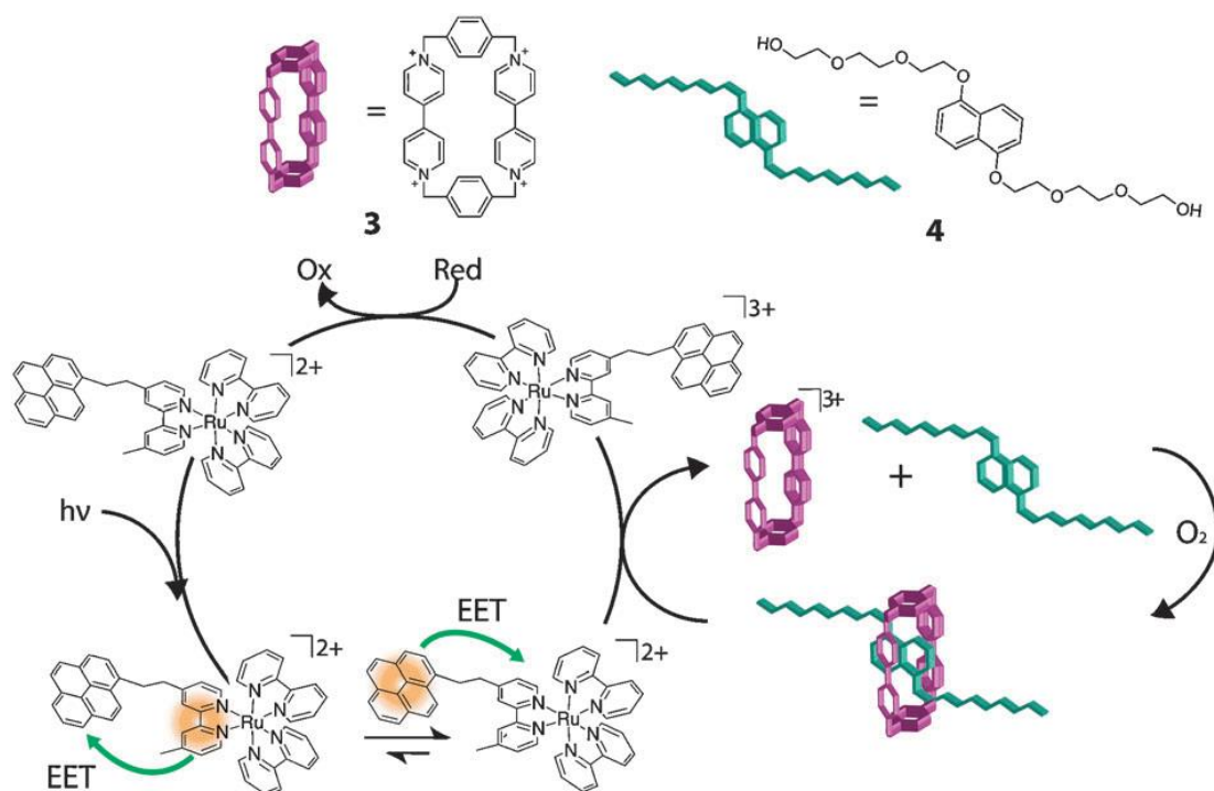
Figure 5.8 Schematic representation of REET occurring in photocatalytic electron pumping driving a molecular piston. The irradiation of a suitable external photosensitizer, in the presence of a sacrificial reductant, induces reduction and disassembly of the pseudorotaxane, while reassembly of the molecular piston is restored in the presence of oxygen. Adapted from reference [20]. Copyright RSC publishing 2012.
