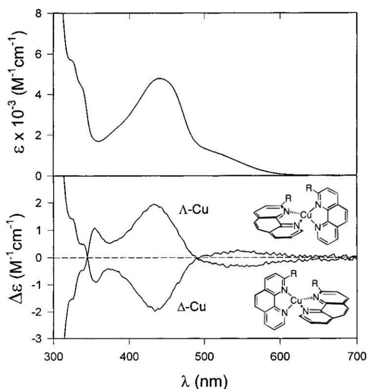
Figure 4.5 Absorption (top) and circular dichroism (bottom) spectra of \Lambda and \Delta [\text{Cu}(2\text{-R-phen})]^+ in \text{CH}_2\text{Cl}_2 solution at 298 K. Adapted from reference [8]. Copyright American Chemical Society 1998.
