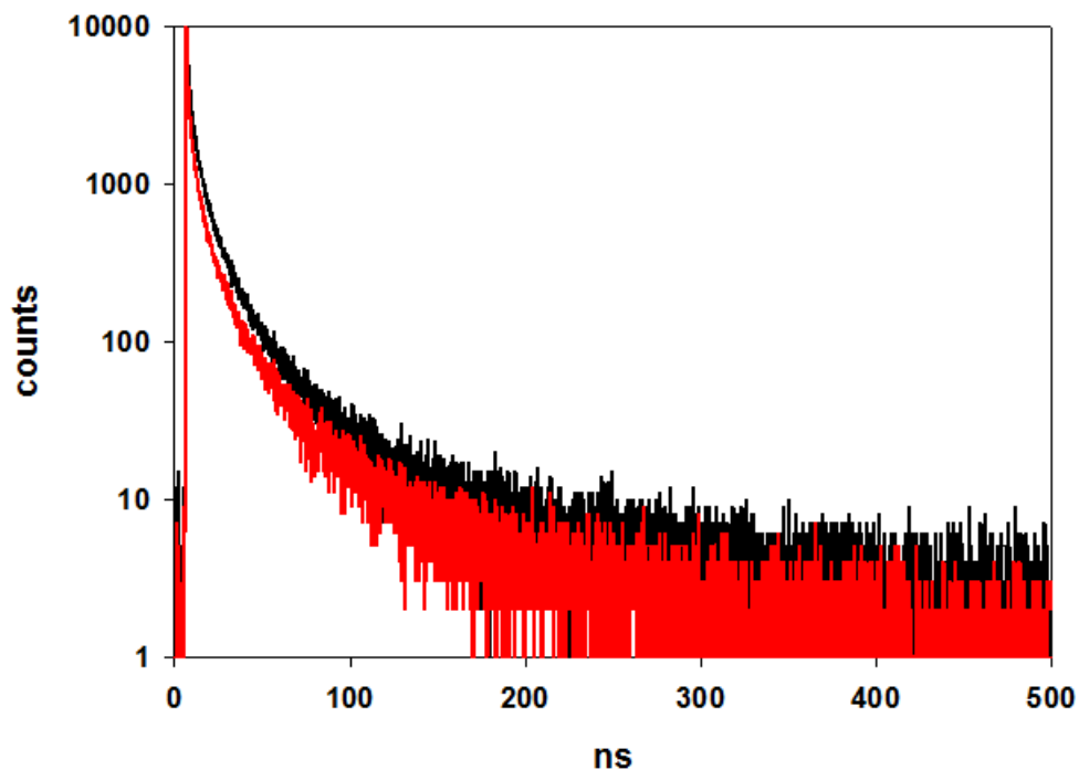
Figure 5.18 Luminescence lifetimes of CdSe-4ZnS decorated with LAPEG 400 (black decay), LAPEG 400 /LA-PYR (red decay) recorded in deaerated MeOH by exciting selectively QDs at 405 nm. The time scale is 500 ns while the 10000 counts detected at 615 nm are reported in logarithmic scale.
