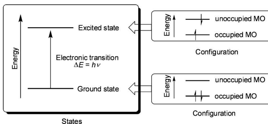
Figure 4.2 Schematic representation of an electronic transition. Adapted from reference [7]. Copyright Royal Society of Chemistry 2012.
