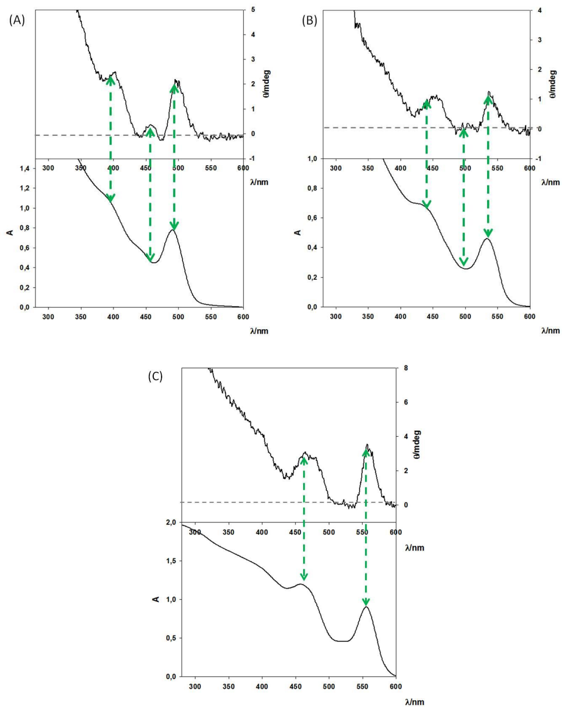
Figure 4.15 CD (at the top) and Isotropic (at the bottom) Absorption spectra of CdSe QDs samples 1 (A); 2 (B) and 3 (C).
