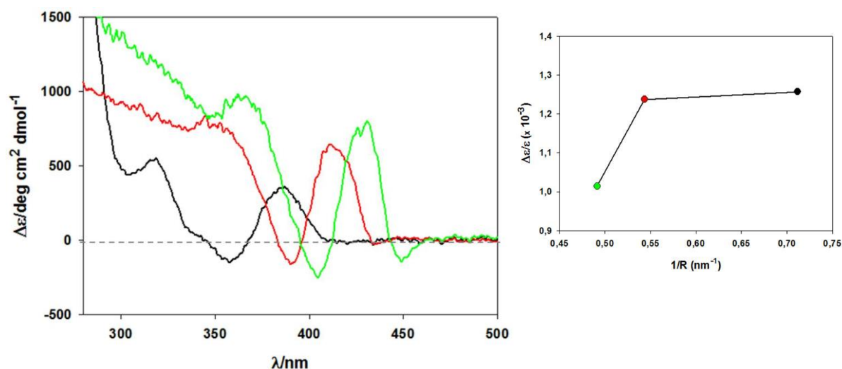
Figure 4.14 Differential Absorption Coefficient Spectra of CdS QDs samples 1 (black line), 2 (red line) and 3 (green line). In the inset the dissymmetry factor is reported as function of the size of QDs.
