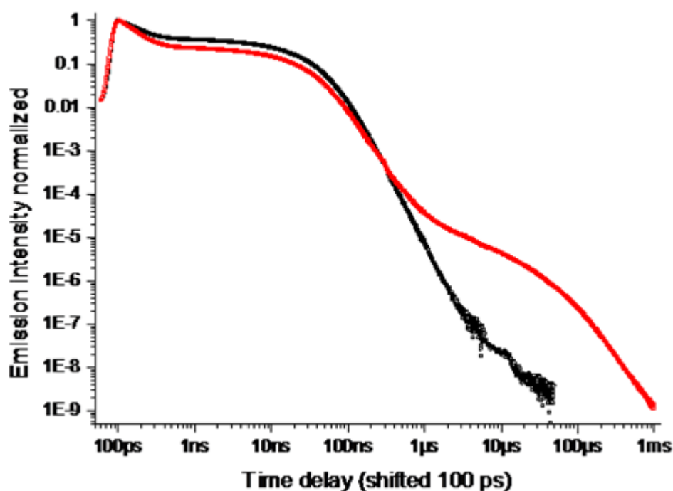
Figure 5.23 Emission decay of CdSe3 (black line) and CdSe3-1PCA (red line) in deaerated heptane; recorded with a streak camera and by exciting at 465 nm.
