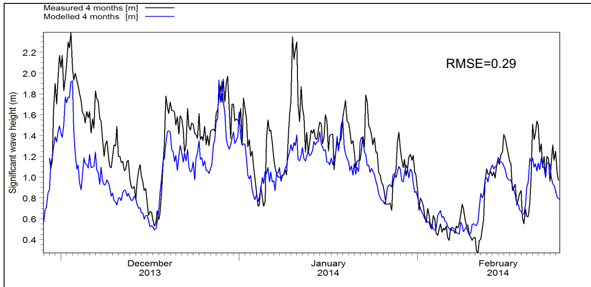
Figure 3.5: Comparison between measured and modelled significant wave height at AWAC measurement points in 12 m water depth (see Figure 2.2 for location).
