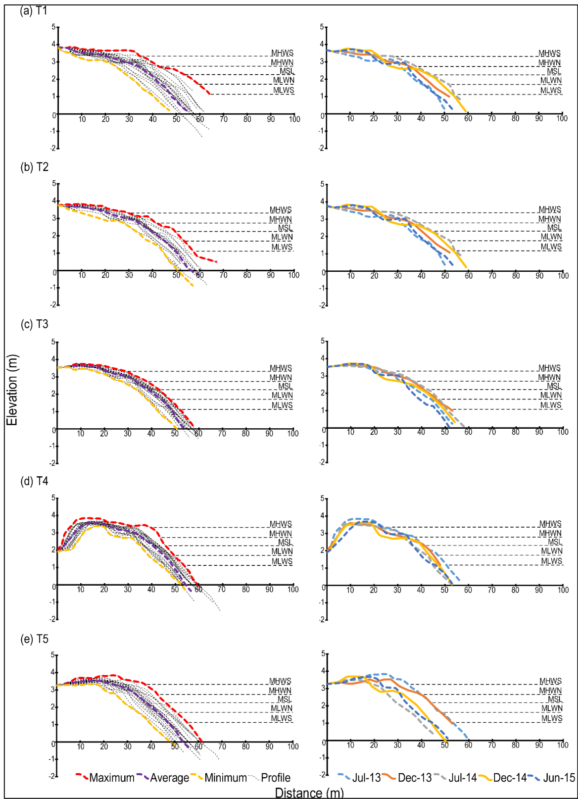
Figure 5.2ii: Pengkalen Maras (B2) beach profile surveyed from July 2013 until June 2015; transects on left and right show profiles over two years and during monsoonal seasons, respectively; (a) Transect 1, (b) Transect 2, (c) Transect 3, (d) Transect 4, and (e) Transect 5.
