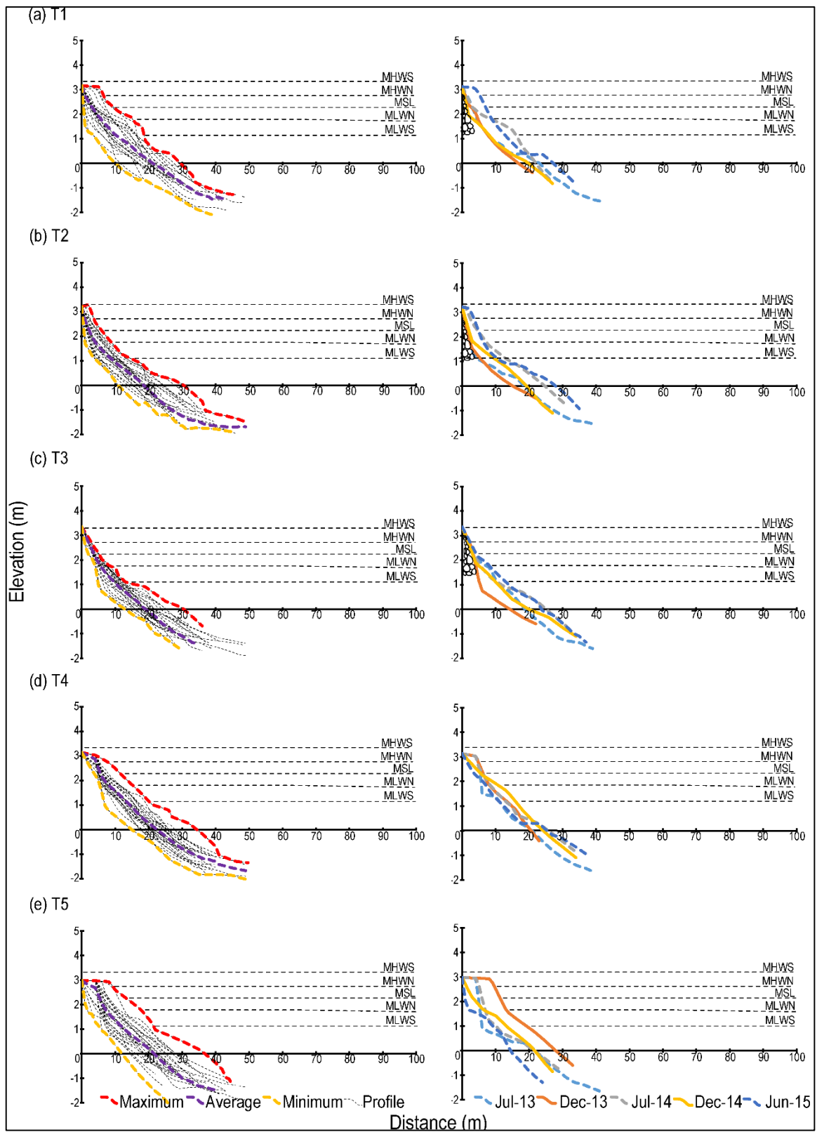
Figure 5.2vi: Kuala Ibai (B6) beach profile surveyed from July 2013 until June 2015; transects on left and right show profiles over two years and during monsoonal seasons, respectively; (a) Transect 1, (b) Transect 2, (c) Transect 3, (d) Transect 4, and (e) Transect 5.
