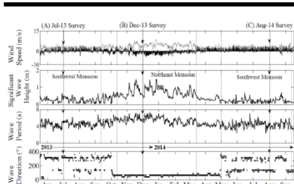
Figure 5. Wind and wave modelled from July 2013 to September 2014: (A) wind speed and direction; (B) significant wave height; (C) wave period; and (D) wave direction. Arrow line represents a profile survey: (A) July 2013; (B) December 2013; and (C) August 2014.
