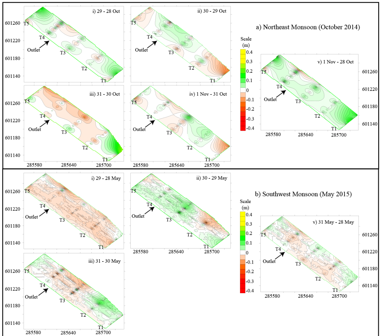
Figure 6.6: The DEM of the bed level change during a) October 2014 and b) Southwest 2015 at B2: Pengkalan Maras beach.
