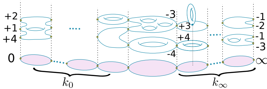
FIGURE 1. Example of relative stable map.
