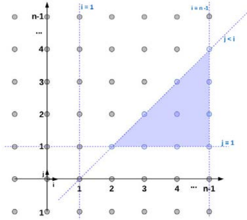
Figure 4.2: Iteration domain
