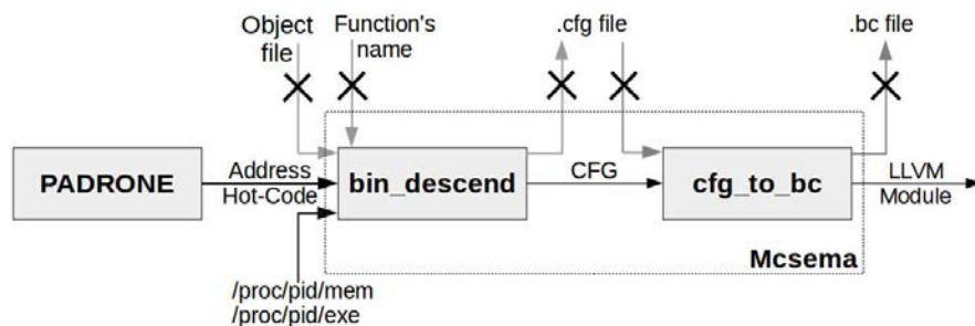
Figure 4.10: Integration of Padrone with McSema
