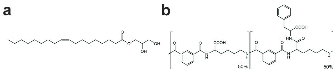
Figure 5.8: The chemical structures of a) Monoolein (MO) and b) Poly(L-lysine- iso -phthalamide) chain grafted with phenylalanine (PP50).
