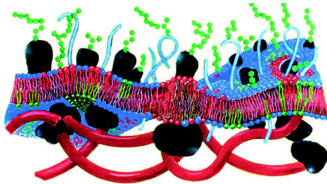
Figure 2.1: Model of the plasma membrane of a eukaryotic cell. The cell membrane displays lateral heterogeneity, lipid domains, and thickness variations. Adapted from [12].
