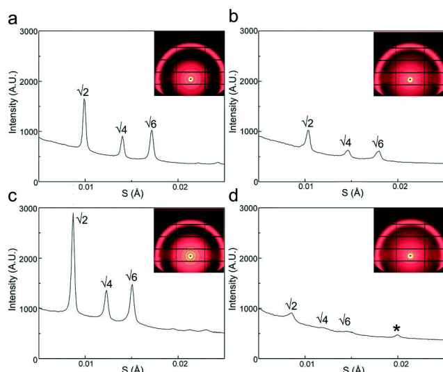
Fig. 3 1-D diffraction plots of intensity vs. scattering parameter S = q/2\pi for MO-cubosomes doped with 10 wt% PP50 polymer. (a) Cubosomes at pH 7.5 (lattice parameter a = 143.0 \pm 0.1 Å, peak positions: 100.8 Å, 71.4 Å, 58.2 Å); (b) cubosomes at pH 5.5 (lattice parameter a = 137.3 \pm 0.4 Å, peak positions: 96.6 Å, 68.5 Å, 55.8 Å); (c) cubosomes with polymer at pH 7.5 (lattice parameter a = 163.2 \pm 0.1 Å, peak positions: 114.9 Å, 81.6 Å, 66.8 Å); (d) cubosomes with polymer at pH 5.5 (lattice parameter a = 167.2 \pm 0.1 Å, peak positions: 116.7 Å, 84.2 Å, 68.5 Å, 50 Å). The peak indicated by * corresponds to a spacing of 50 Å.
