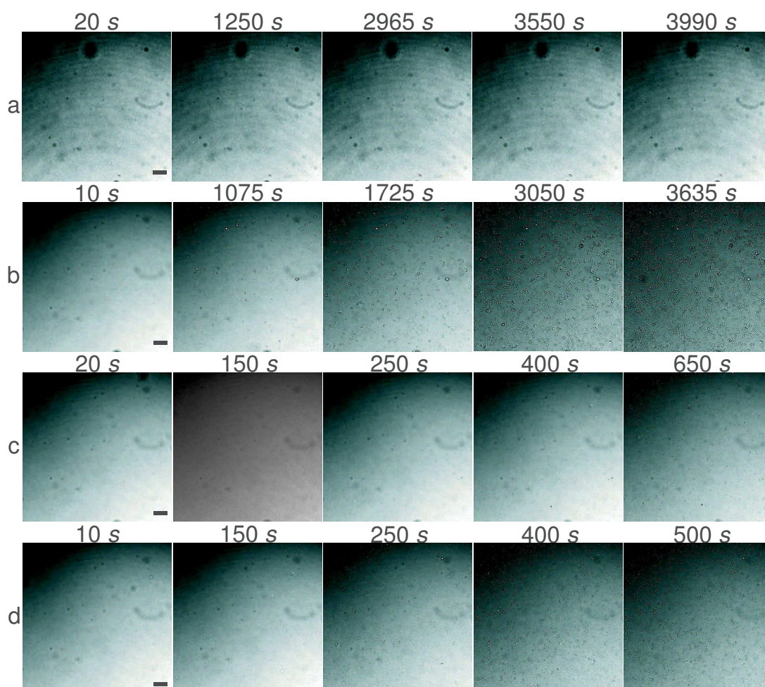
Figure A.1: Bright field images of DOPC SLB marked with DiI at various \alpha -CD concentrations: a) 5 mM b) 10 mM c) 15 mM d) 20 mM. There is a 120 s lag time between the injection of \alpha -CD into the measuring chamber and the beginning of the microscopy acquisition.
