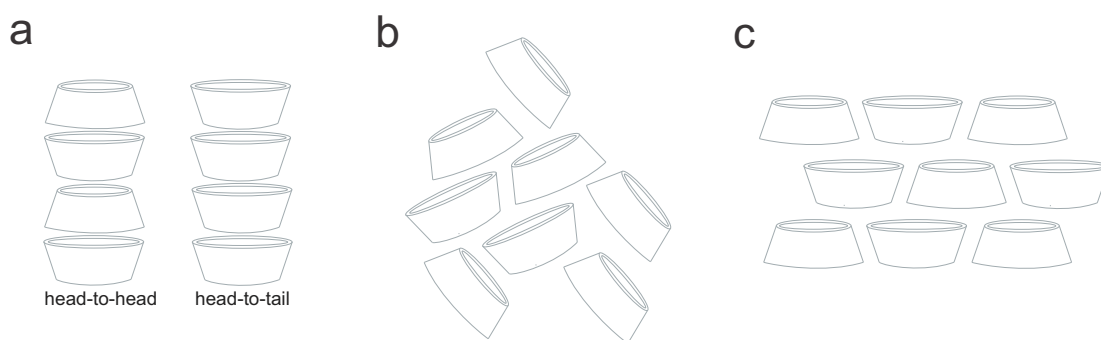
Figure 4.2: Alignment of cyclodextrin rings in complex crystal structures: a) channel b) cage c) layer.
