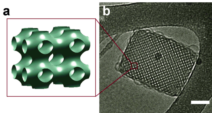
Figure 5.7: a) Graphical picture of an inverse cubic phase with primitive type structure Im3m b) Cryo-TEM image of a monoolein cubosome stabilized with 5 wt % Pluronic F127. Scale bar, 100 nm.
