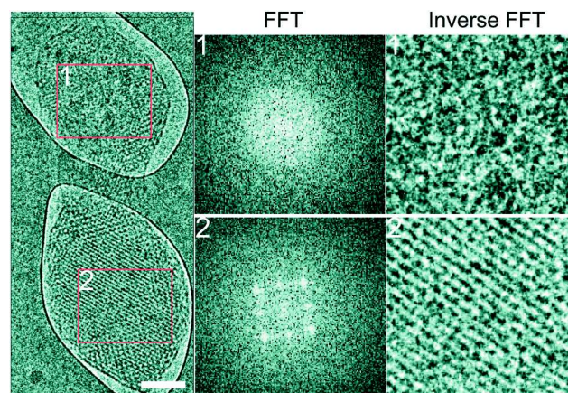
Fig. 5 Cryo-TEM images of a single cubosome at pH 5.5 with incorporated polymer. The red boxes represent the areas used for FFT calculations. Scale bar, 100 nm. ( a = 156.0 \text{ \AA} ). (1) Upper part of particle; (2) lower part of particle.
