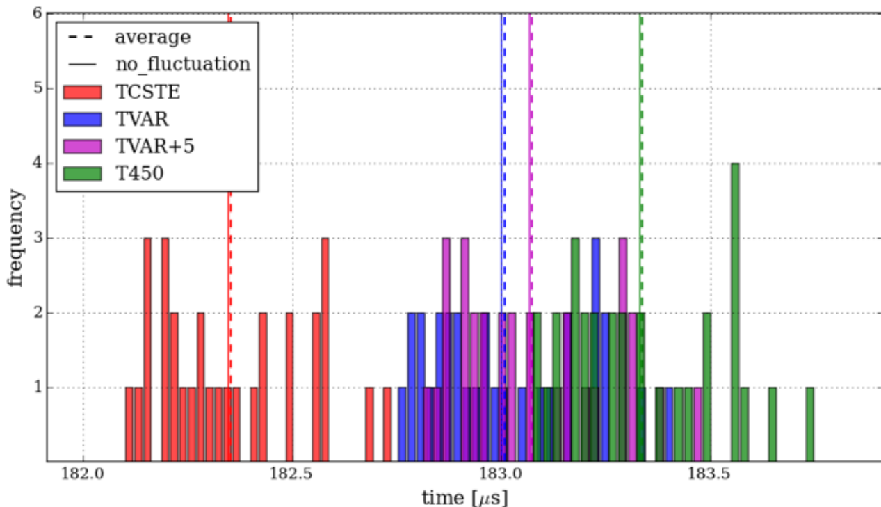
Figure 3.10 Distributions of variation of times of flight resulting from temperature fluctuations for each of the 120 temperature profiles considered, i.e. the 30 random profiles superimposed to each of the four static temperature profiles.
