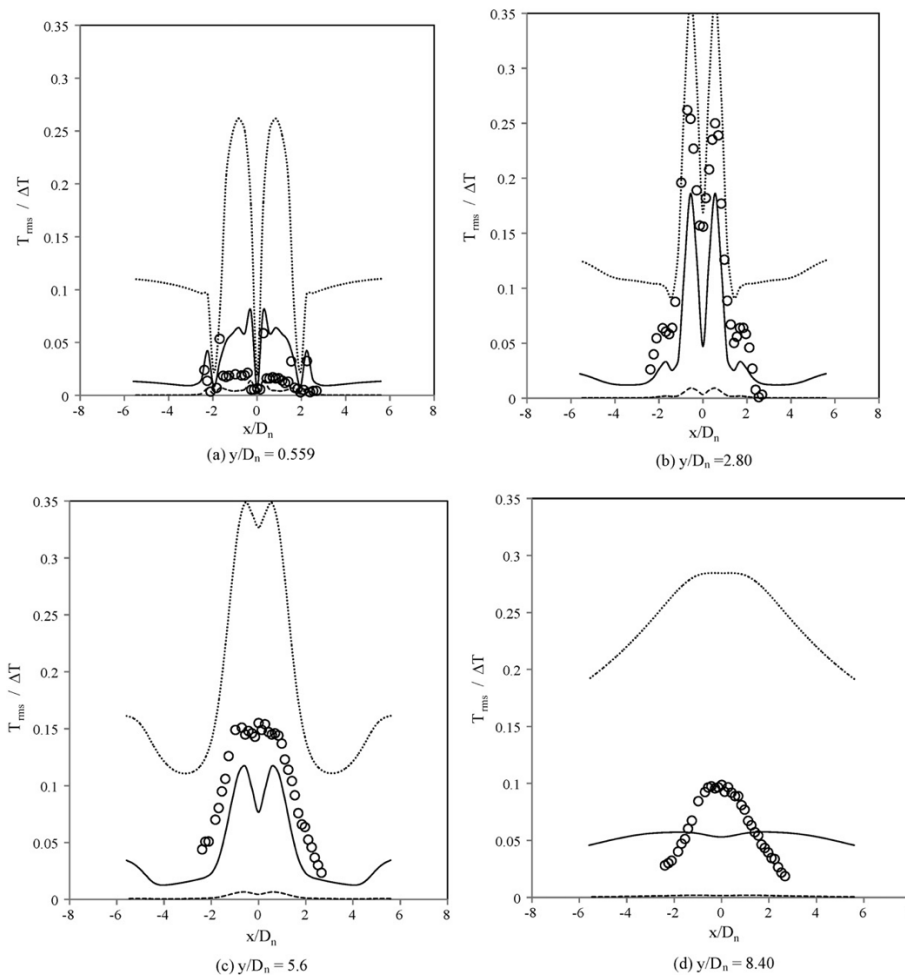
Figure 4.2 Comparison of normalized root mean square of temperature, taken from Durve et al. (2010).
