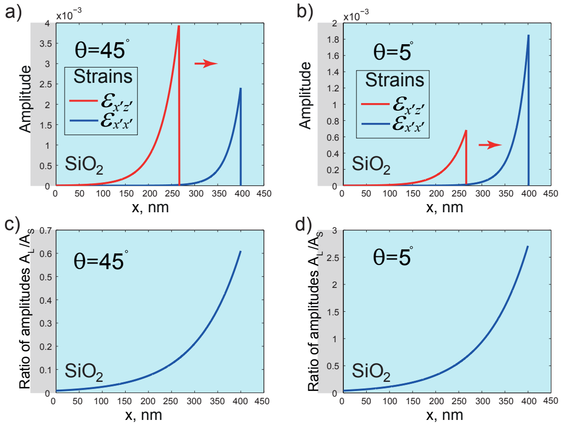
Fig. 2.19: Spatial profiles of longitudinal \epsilon_{x'x'}(x^*, t) and shear \epsilon_{x'z'}(x^*, t) strains at a) \theta = 45 deg and b) \theta = 5 deg. Ratio of the longitudinal A_L and shear A_S strain amplitudes at c) \theta = 45 deg and d) \theta = 5 deg.
