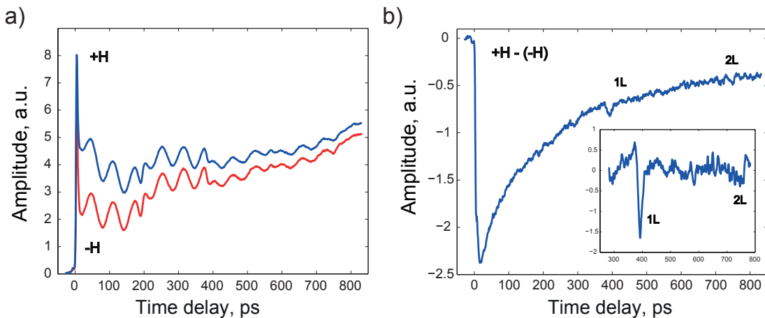
Fig. 2.35: a) Transient time resolved reflectivity signals recorded in a 300 nm TbFe_2/1000 nm SiO_2 multi-layer sample of in-plane static magnetization at two out-of-plane magnetic field orientations \pm H . b) Differential signal +H - (-H) with subtracted background (the inset). P-polarized probe beam with 800 nm wavelength is obliquely incident to the surface. The inset shows the detection of longitudinal echoes.
