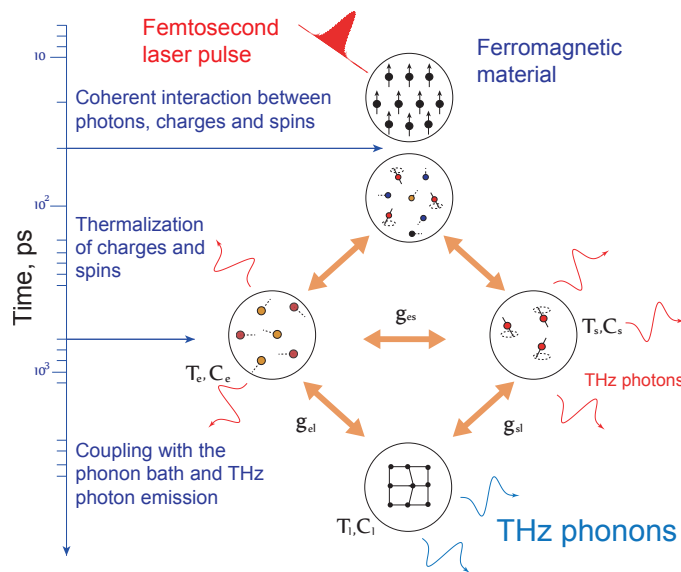
Fig. 1.2: Scheme of the interaction of a laser pulse and the spin state of a magnetic material [23].
