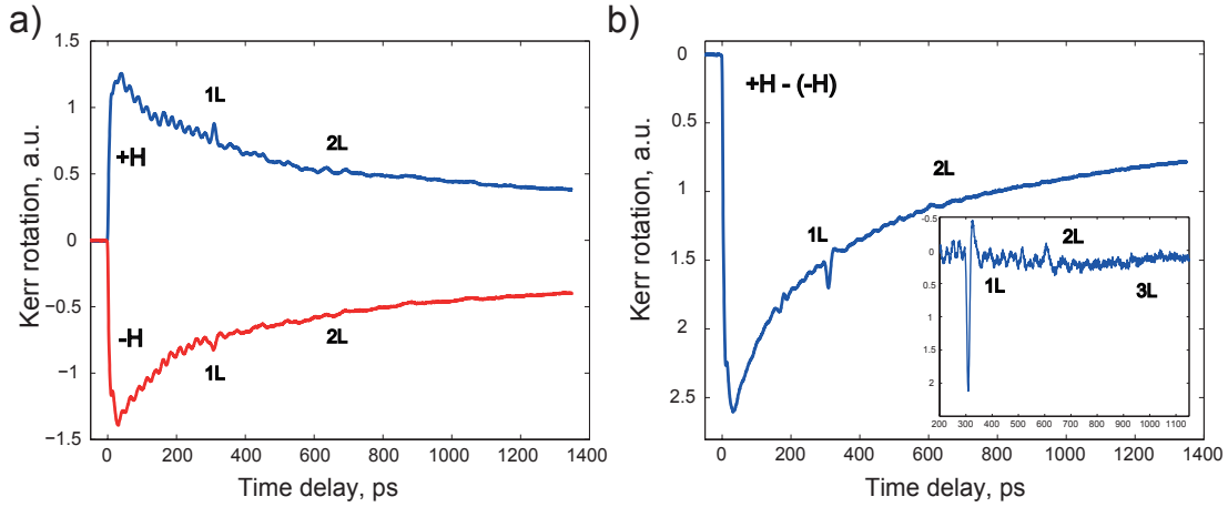
Fig. 2.34: a) Transient time resolved pump-probe MOKE signals recorded in a 300 nm TbFe_2/775 nm SiO_2 multi-layer sample of in-plane static magnetization at two out-of-plane magnetic field orientations \pm H . b) Differential signal +H - (-H) with subtracted background (the inset) reveals only the presence of longitudinal acoustic waves generated in the 300 nm Terfenol layer. Probe of 400 nm wavelength is normal incident to the surface.
