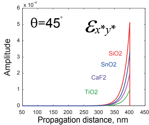
Fig. 2.44: \varepsilon_{x'y'} shear strain amplitude as a function of acoustic delay line material.
