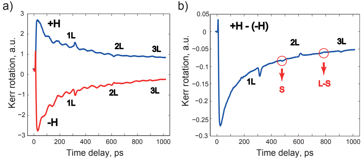
Fig. 2.22: a) Transient time resolved pump-probe MOKE signals recorded in a 300 nm TbFe_2/775 nm SiO_2 multi-layer sample of in-plane static magnetization at two out-of-plane DC magnetic field orientations \pm H=7 kOe. b) Differential signal +H - (-H) reveals the presence of longitudinal (L) and shear (S) acoustic echoes.
