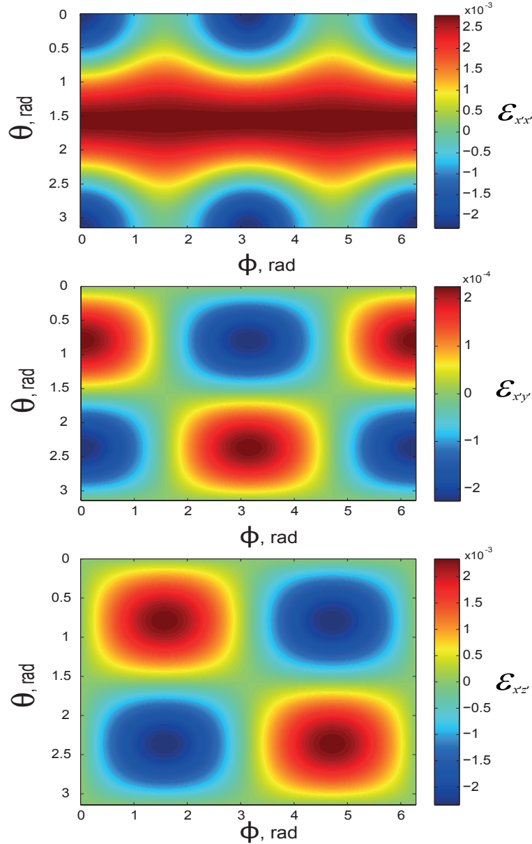
Fig. 2.11: Angular dependence of the longitudinal \varepsilon_{x'x'} and shear \varepsilon_{x'y'} , \varepsilon_{x'z'} strain amplitudes on \theta out-of-plane magnetization tilt angle and \phi - azimuthal angle of \vec{M} projection on y'z' plane of the in-plane magnetized films.
