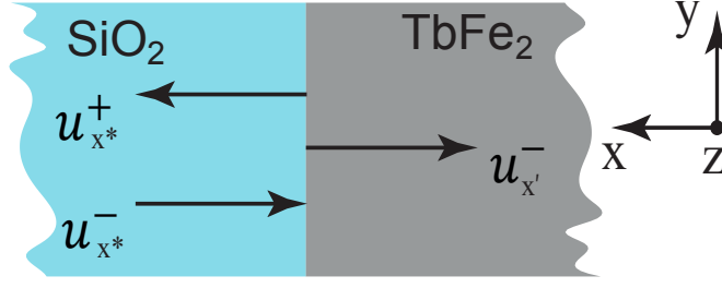
Fig. 2.41: Incident and reflected strain waves at the SiO_2/TbFe_2 interface along the x direction.
