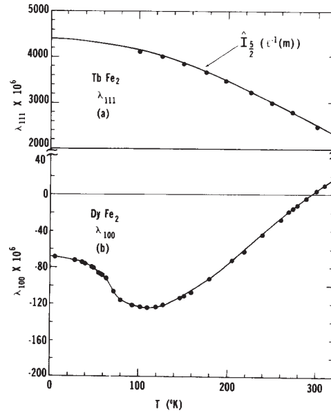
Fig. 2.16: Temperature dependence of a) TbFe_2 and b) DyFe_2 magnetostriction coefficients \lambda_{[111]} , \lambda_{[100]} , respectively [95].
