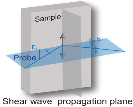
Fig. 1.7: Illustration of shear acoustic waves detection conditions.
