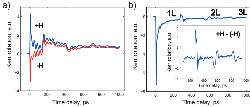
Fig. 2.25: a) Transient time resolved pump-probe MOKE signals recorded in a 50 nm TbFe_2/700 nm SiO_2 multi-layer sample of in-plane static magnetization at two out-of-plane magnetic field orientations \pm H . b) Differential signal +H - (-H) with subtracted background reveals only the presence of longitudinal acoustic waves generated in the 50 nm Terfenol layer.
