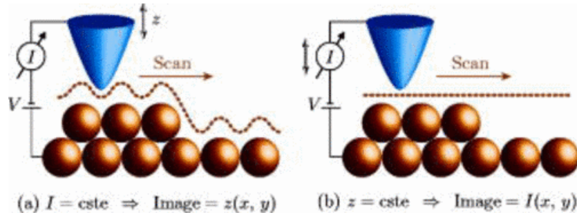
Figure 2.2: Left: Illustration of the constant-current imaging mode: the tip height follows the surface to keep a constant tunneling current. Right: Illustration of the constant-height imaging mode. Variations of the current are measured during a constant-height scan. From Ref. 30.
