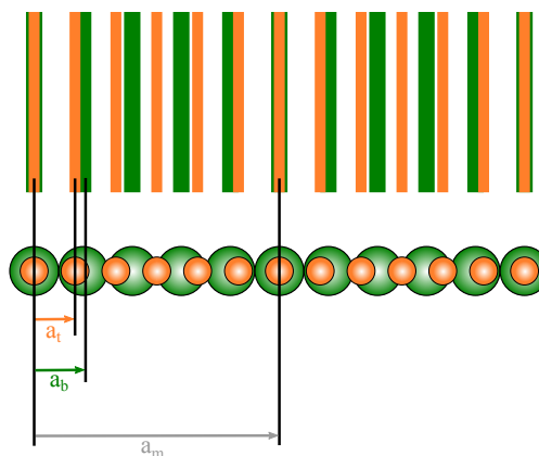
Figure 1.9: Mismatched 1D lattices : top layer in orange, bottom layer in green. The bottom part is a ball model of the atomic lattices whereas the top part shows the same lattices but with lines to make the 1D moiré pattern visually appear. The beating matches the moiré periodicity (see text)
