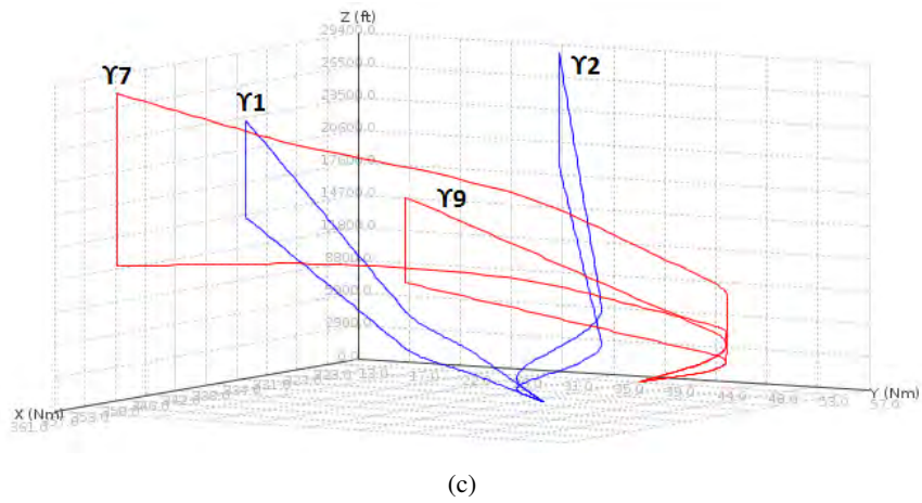
Figure 6.26: Test Zurich airport: SA method simulation results. (a) Illustration in the horizontal plane. (b) Fictitious obstacles for route deviation. (c) Illustration of \gamma_1 , \gamma_2 , \gamma_7 and \gamma_9 in 3D.
