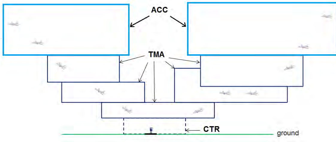
Figure 1.6: Controlled airspace structure.
