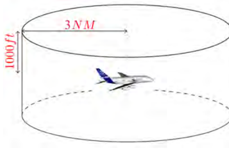
Figure 1.10: Standard separation norm in a TMA.
