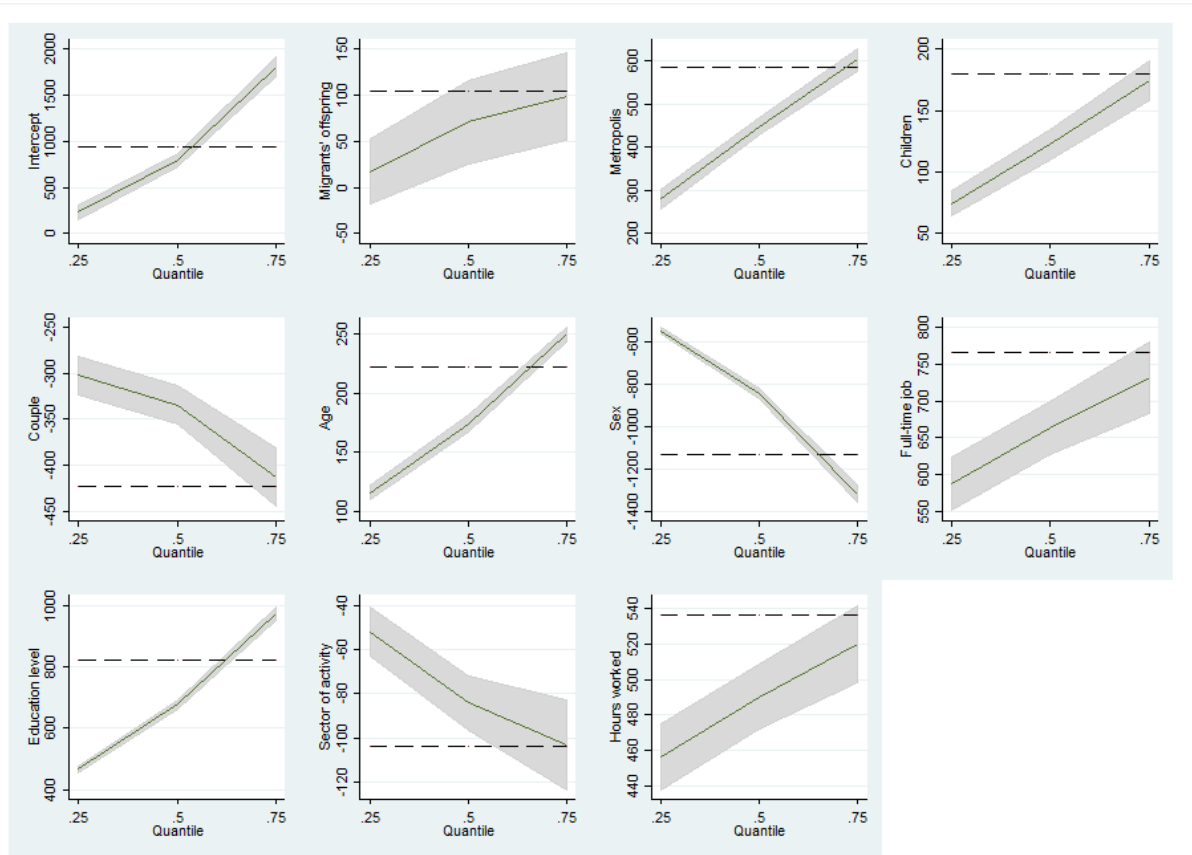
Figure 3.9. Quantile regressions on the wage distribution in the United States: estimation of the coefficients
