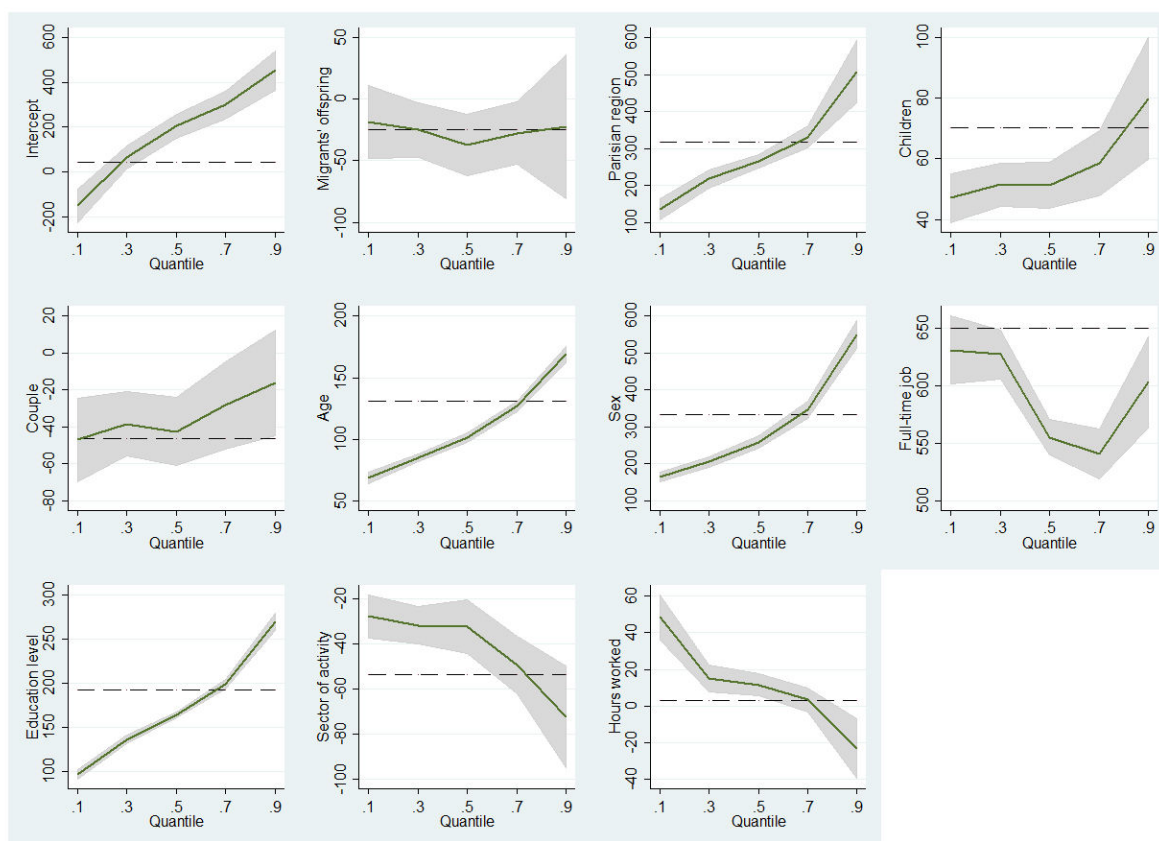
Figure 3.A.1. Quantile estimations (on the quintiles) of the French sample
