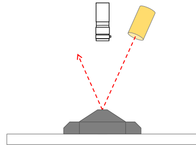
Figure 3.3: Bright field lighting
