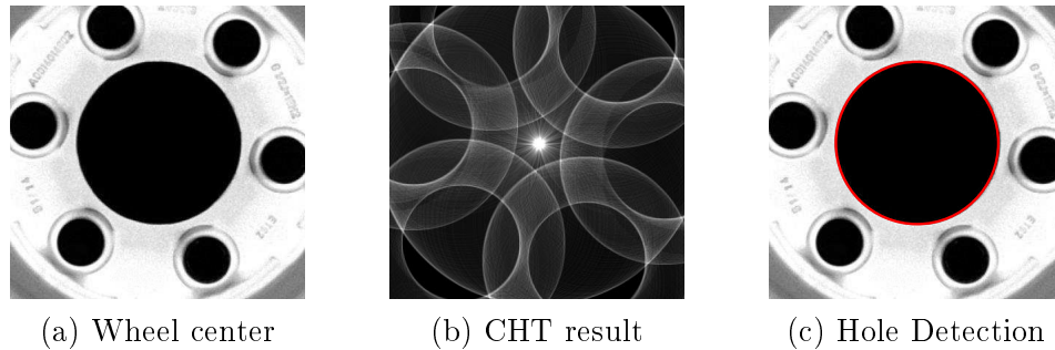
Figure 4.4: Illustration of steps for pilot hole detection
