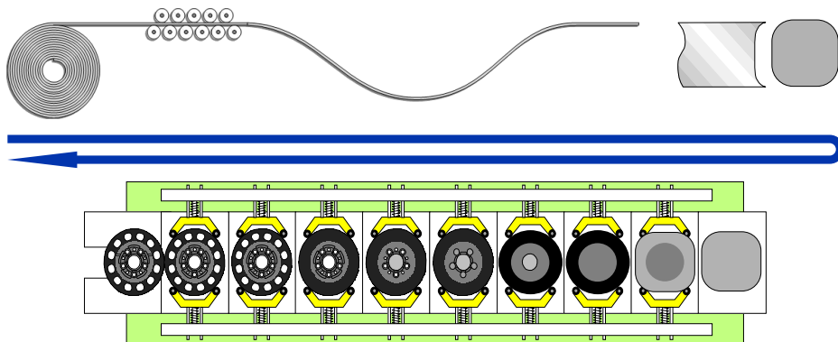
Figure 2.2: Illustration of the disc stamping process
