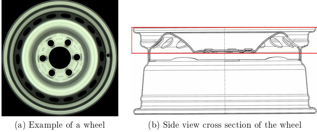
Figure 3.1: An example of a wheel to be inspected with an illustration of its design
