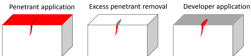
Figure 2.7: Principle of the penetrant testing technique
