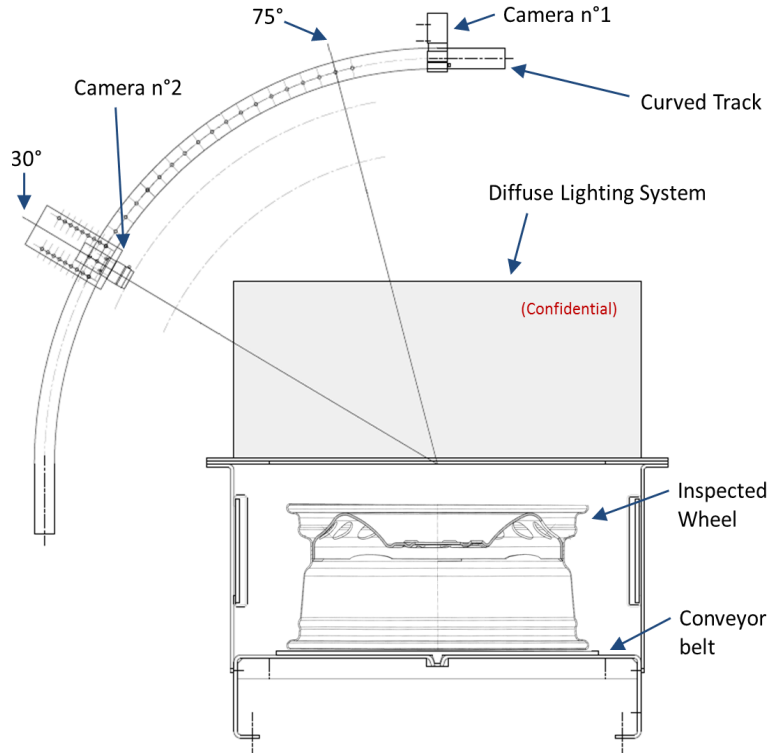
Figure 3.6: Illustration of the AVI prototype installation
