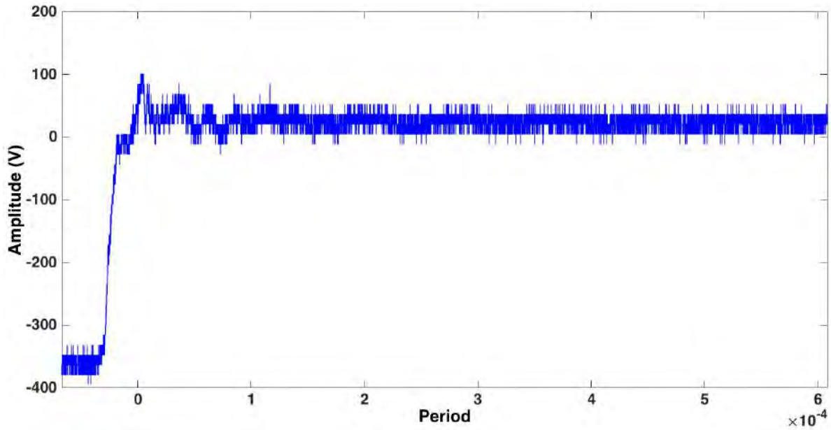
Figure IV.6: Rising edge of the voltage
